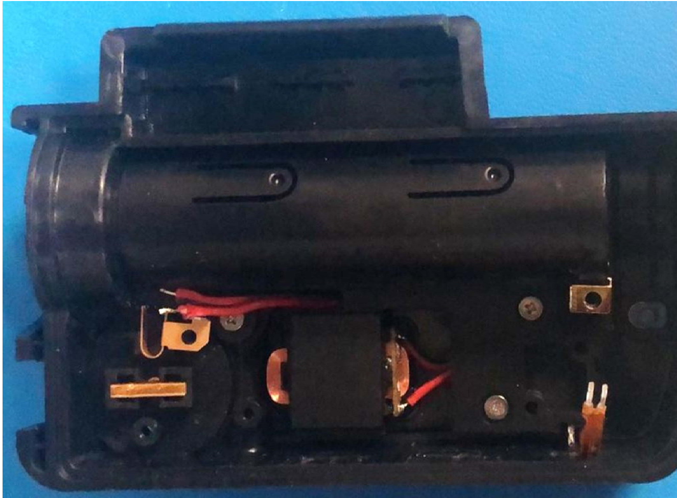
Figure E22.5 – Internal Photo – Battery Compartment
