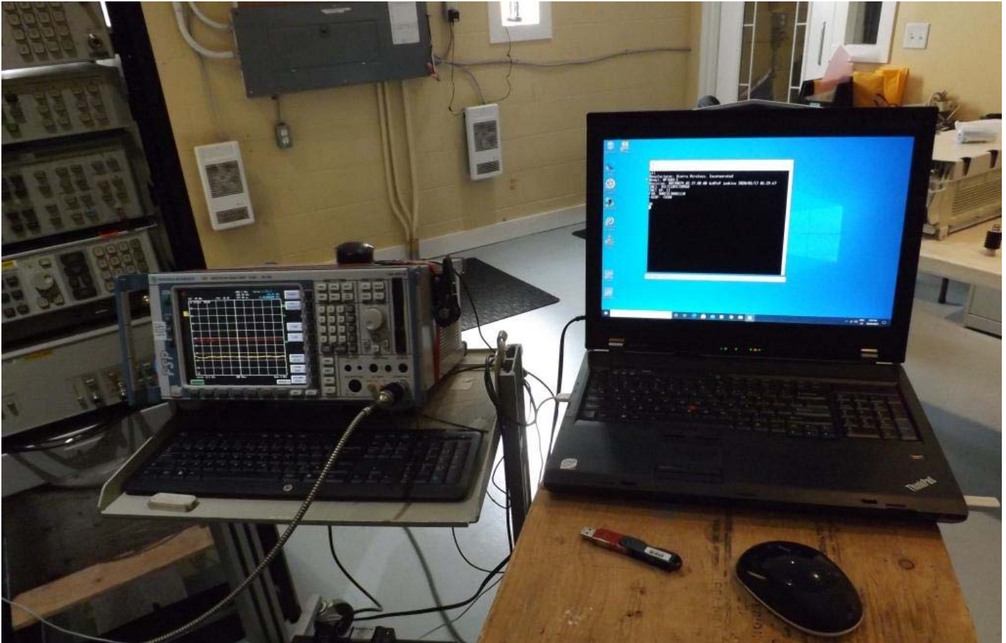
Figure E23.2 – Setup Photo – Conducted Measurements
