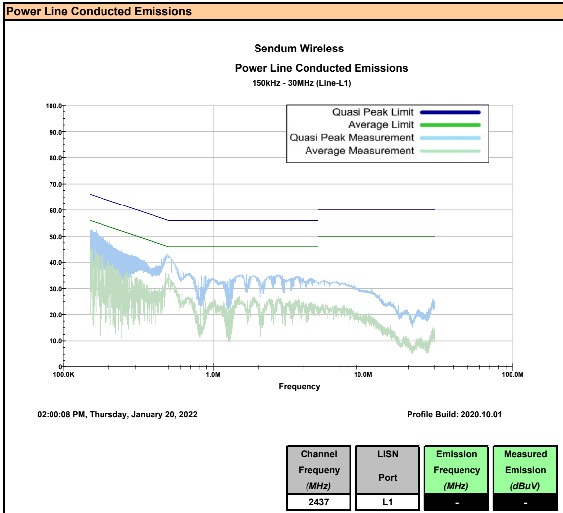
Plot 9.1 – Line Conducted Emissions, L1
