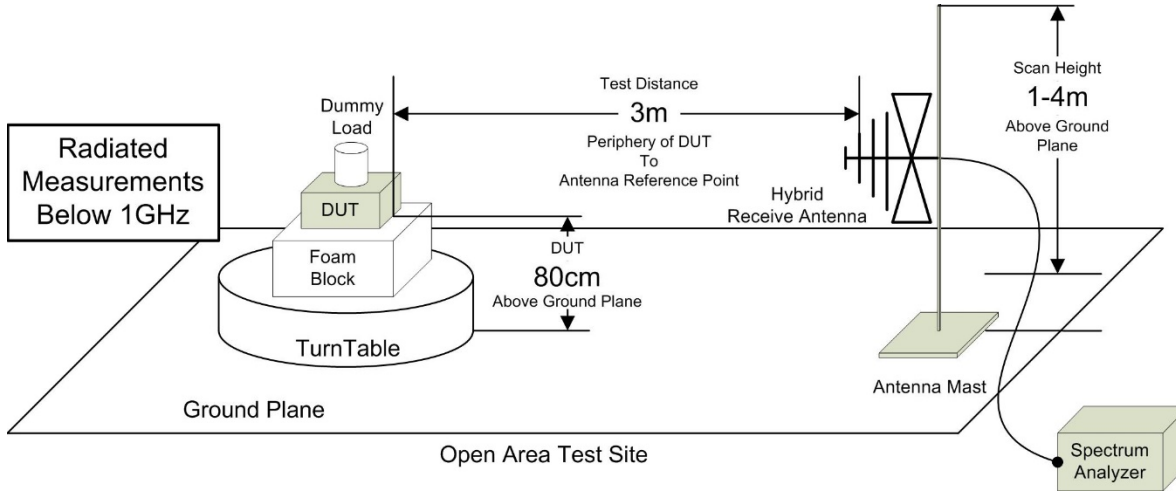
Figure A.3 – Test Setup Radiated Emissions Measurements 30 – 1000MHz w/ Signal Substitution
