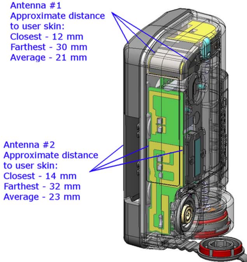
Figure E19.8 – Antenna Locations
