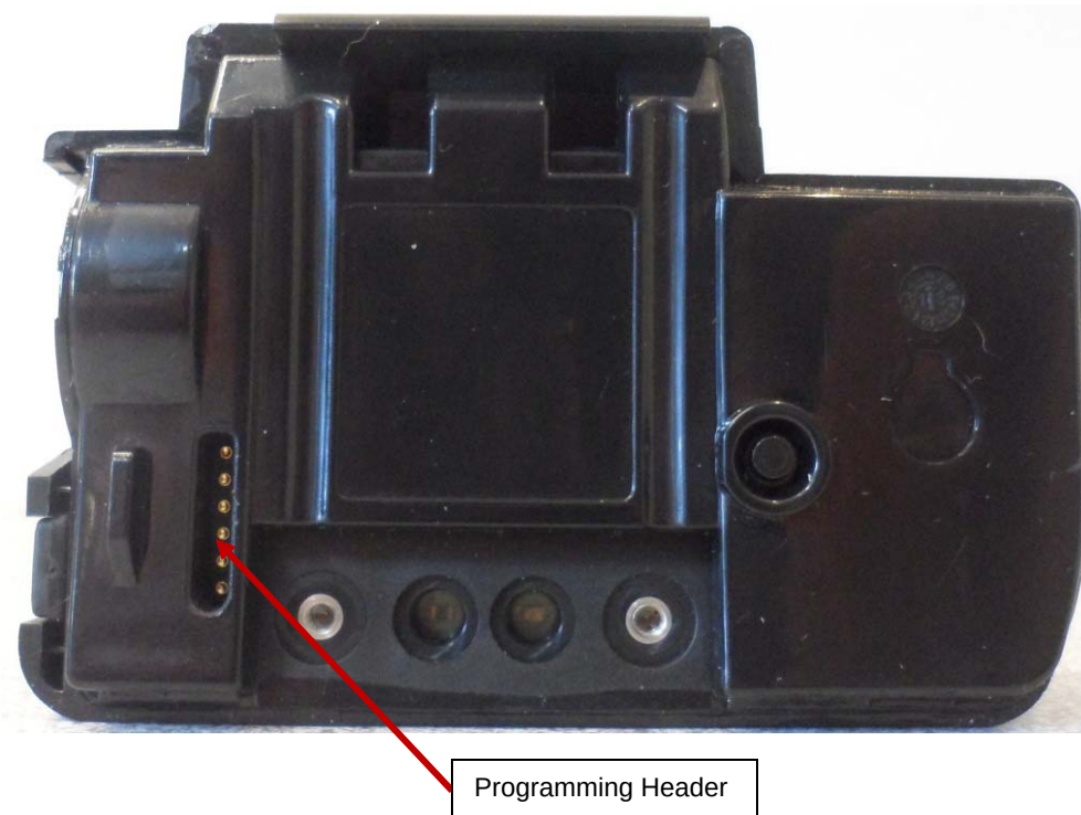
Figure E19.7 – External Photo – Belt Clamp Removed
