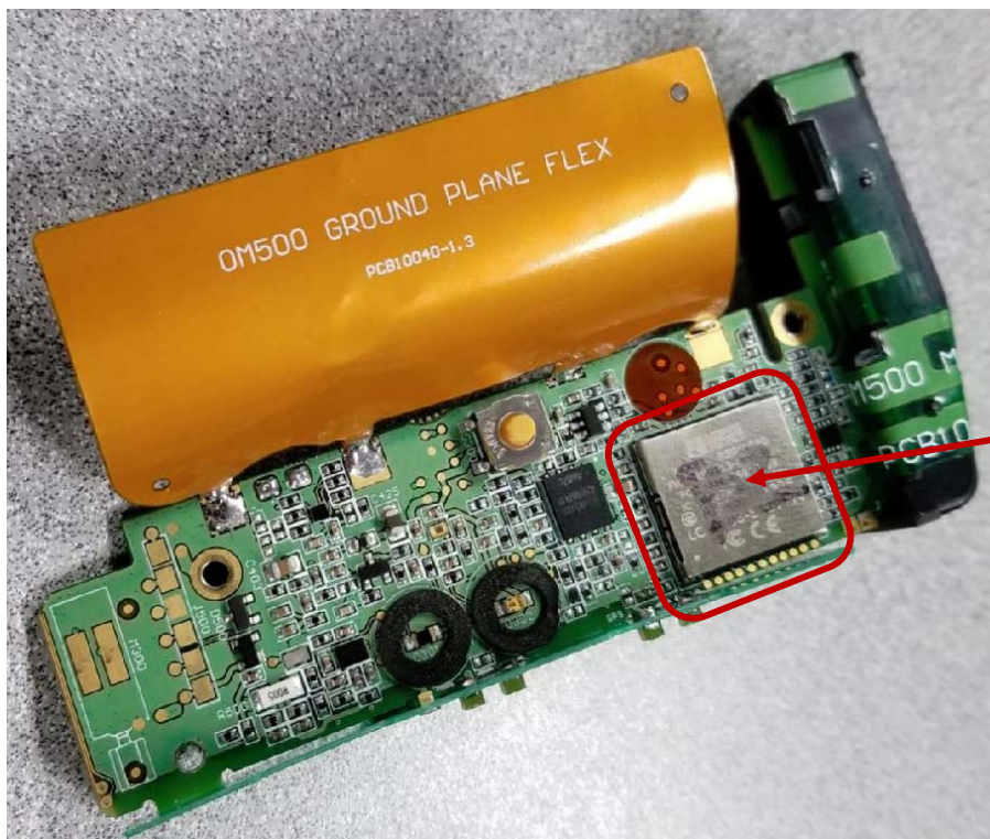
Figure E20.3 – Internal Photo – PCB Top
