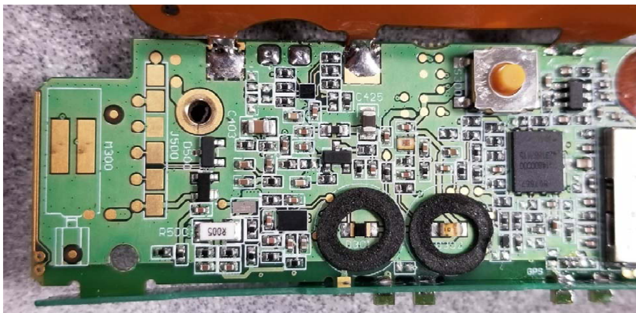
Figure E20.5 – Internal Photo – Close Up - PCB Top
