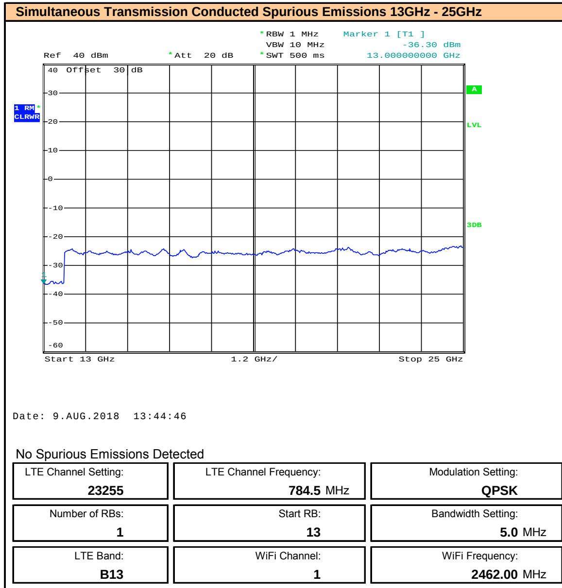
Plot 13.4 – Simultaneous Transmission Conducted Spurious Emissions – 13 to 25GHz
