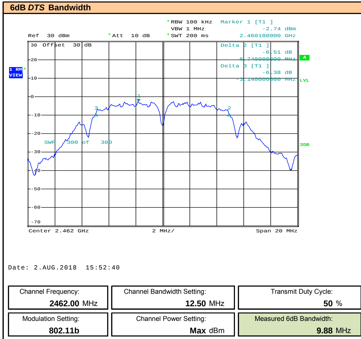
Plot 8.3 – 6dB DTS Bandwidth 2462MHz
