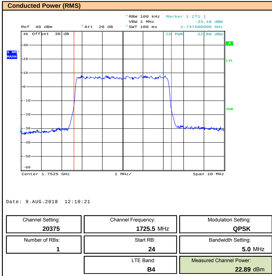
Plot 11.5 – Conducted Power B4- Channel 20375 - QPSK
