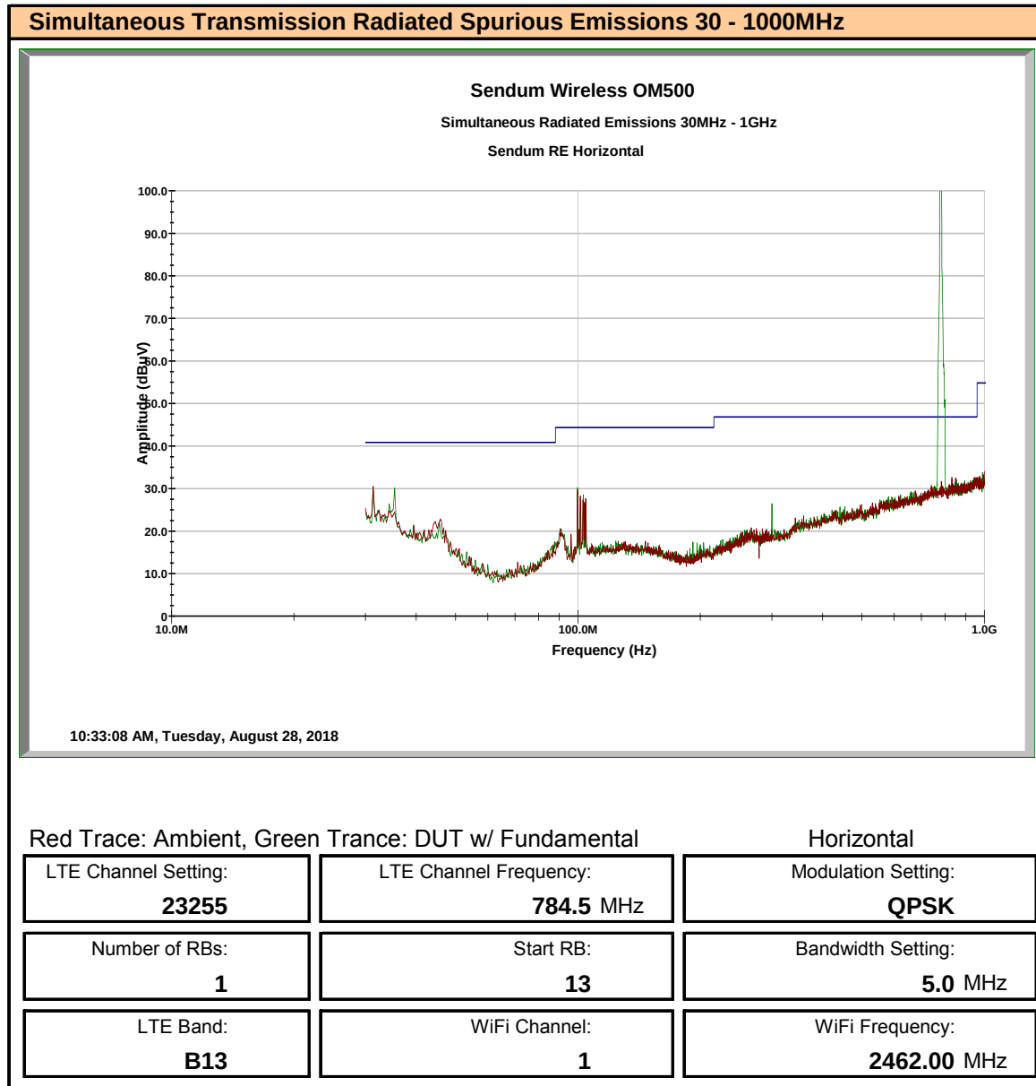
Plot 14.1 – Simultaneous Transmission Radiated Spurious Emissions – 30 - 1000MHz – Horizontal
