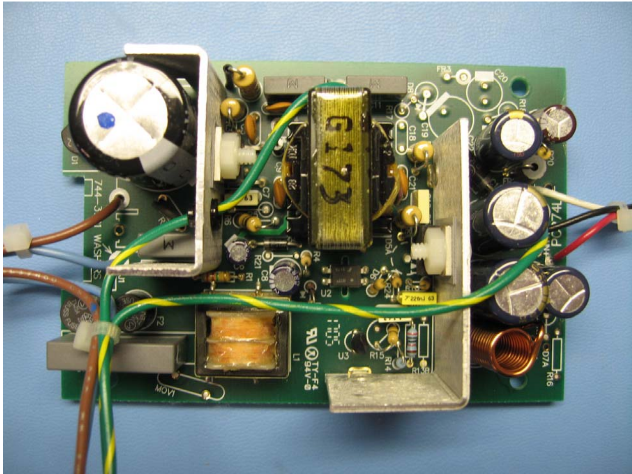
Figure 24 – View of Power Supplies
