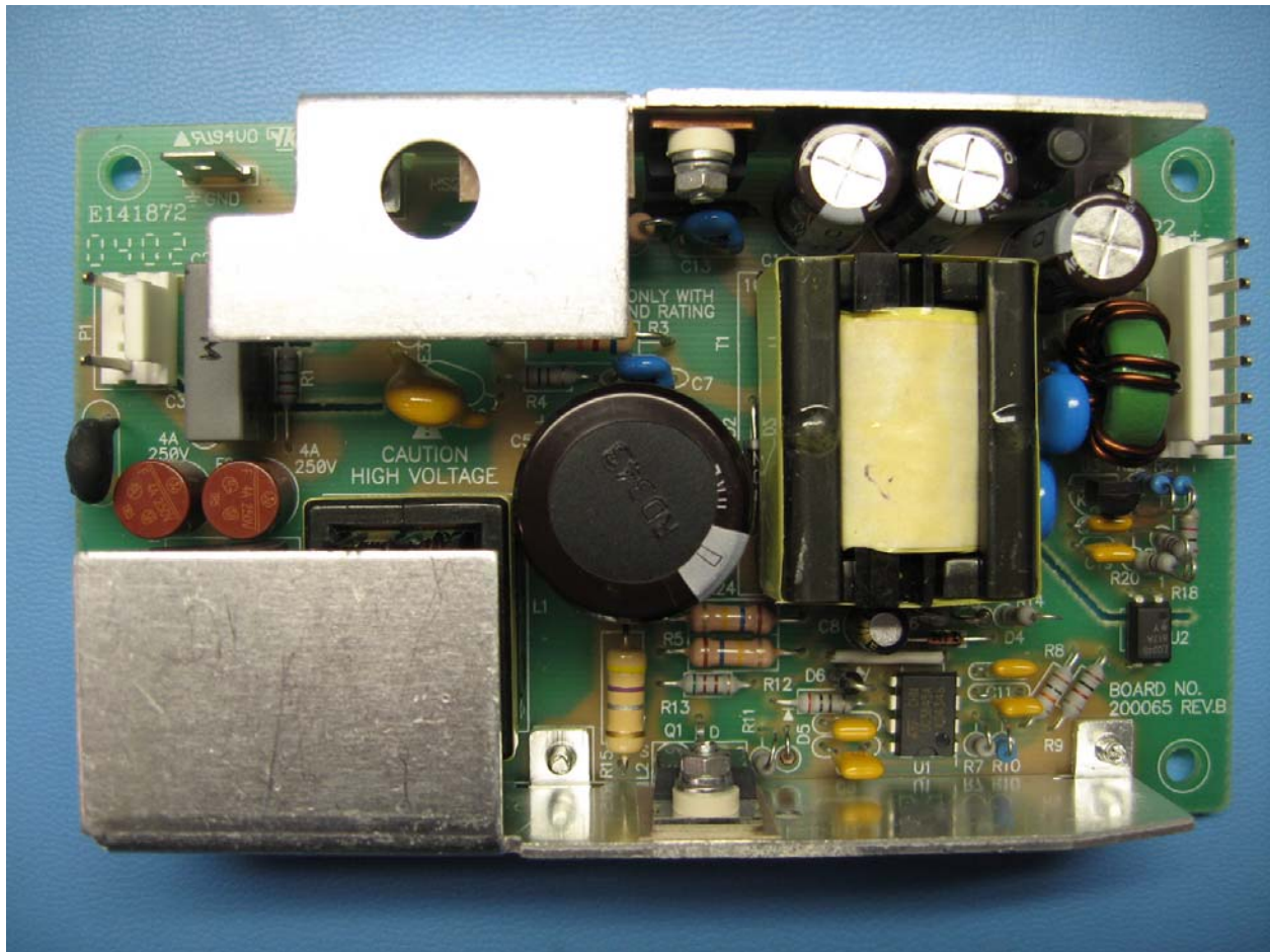
Figure 28 – View of Power Supplies
