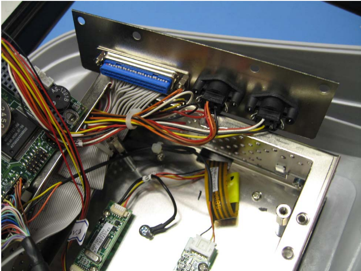
Figure 12 – Panel PC
