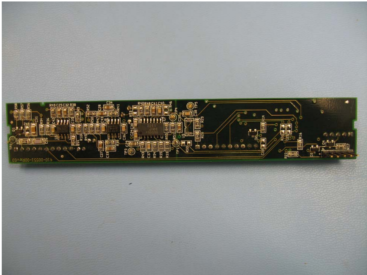
Figure 34 – Close up Control BD circuit board
