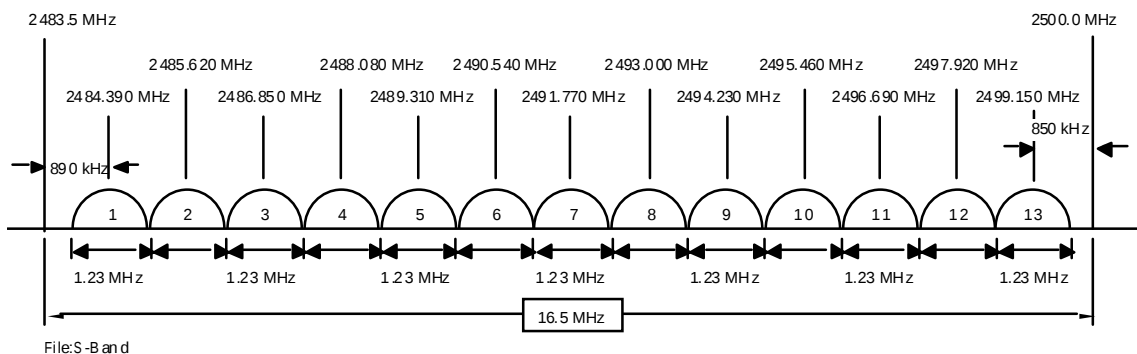
Figure 3-5 S - Band Channel Frequencies
