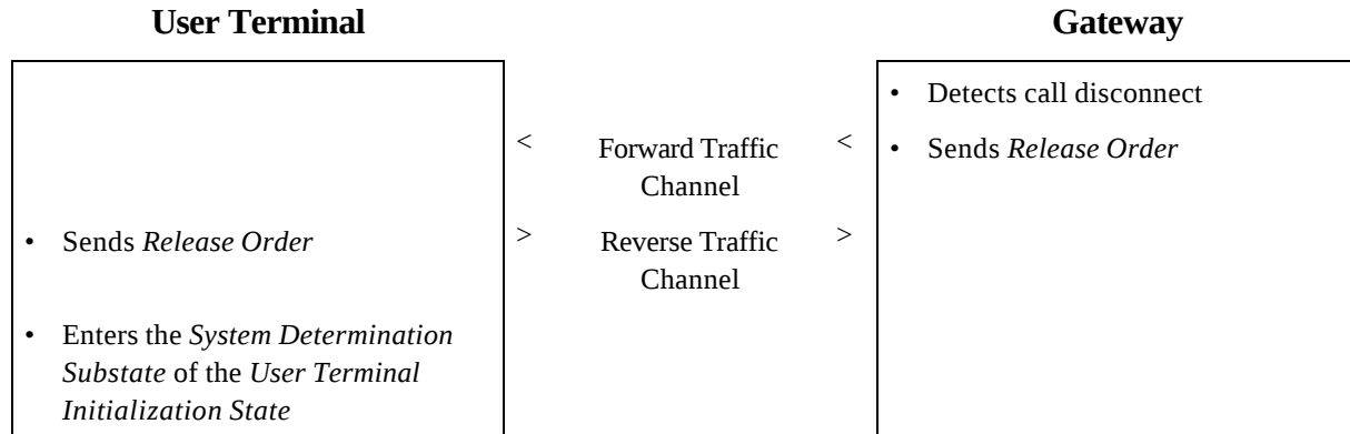
6 Figure 6-10. Simple Call Flow, Gateway Initiated Call Disconnect Example (TIA Call 7 Control Procedures) 8 (Part 1 of 2)
