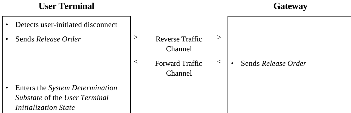
3 Figure 6-8. Simple Call Flow, User Terminal Initiated Call Disconnect Example (TIA Call 4 Control Procedures) 5 (Part 1 of 2)
