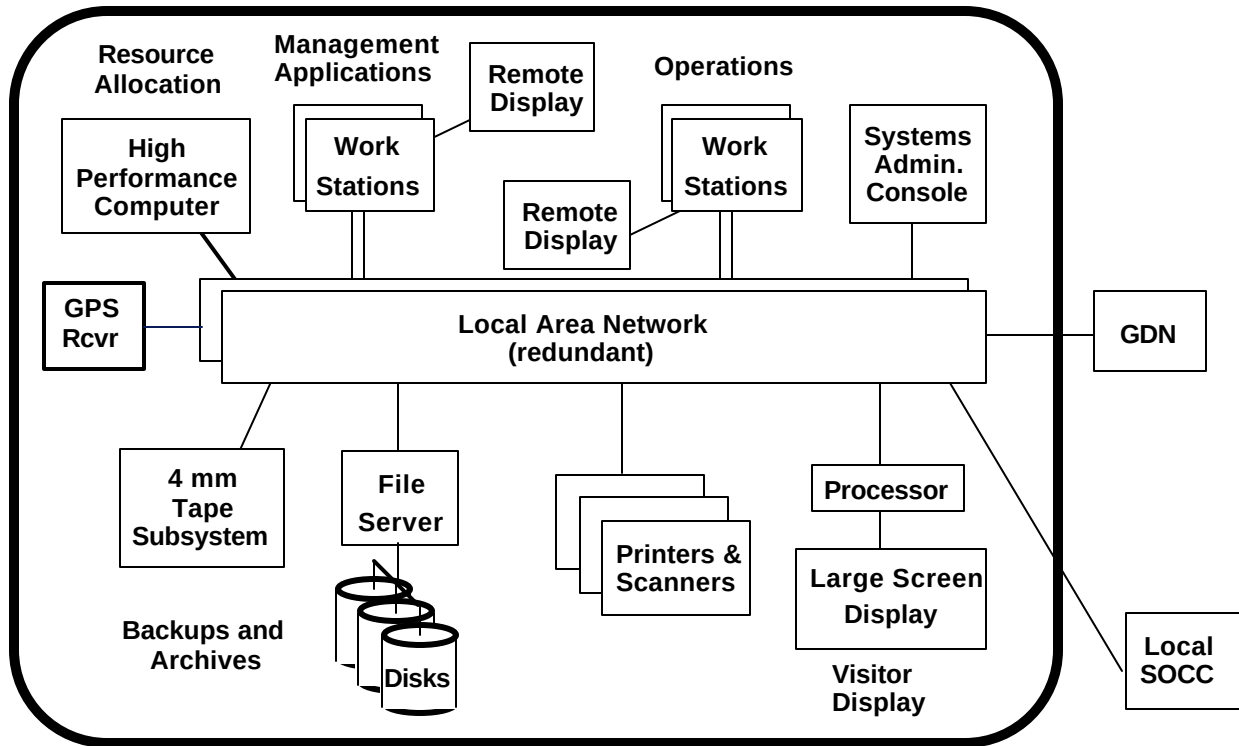
Figure 2-11 GOCC Simplified Block Diagram
