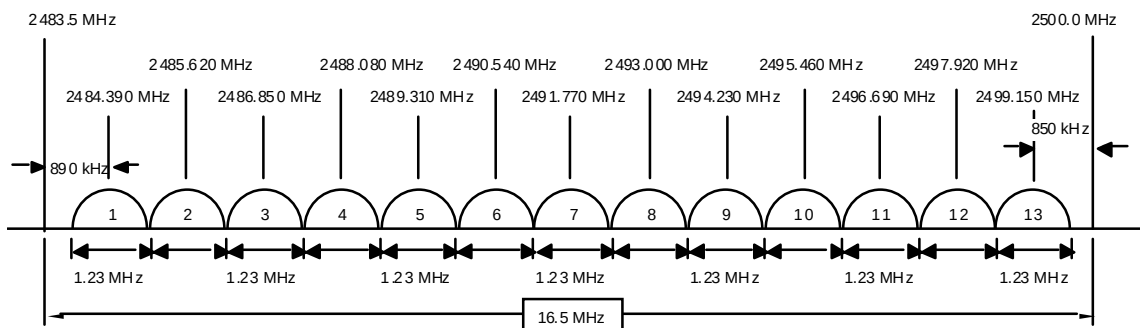
Figure 3-5 S - Band Channel Frequencies
