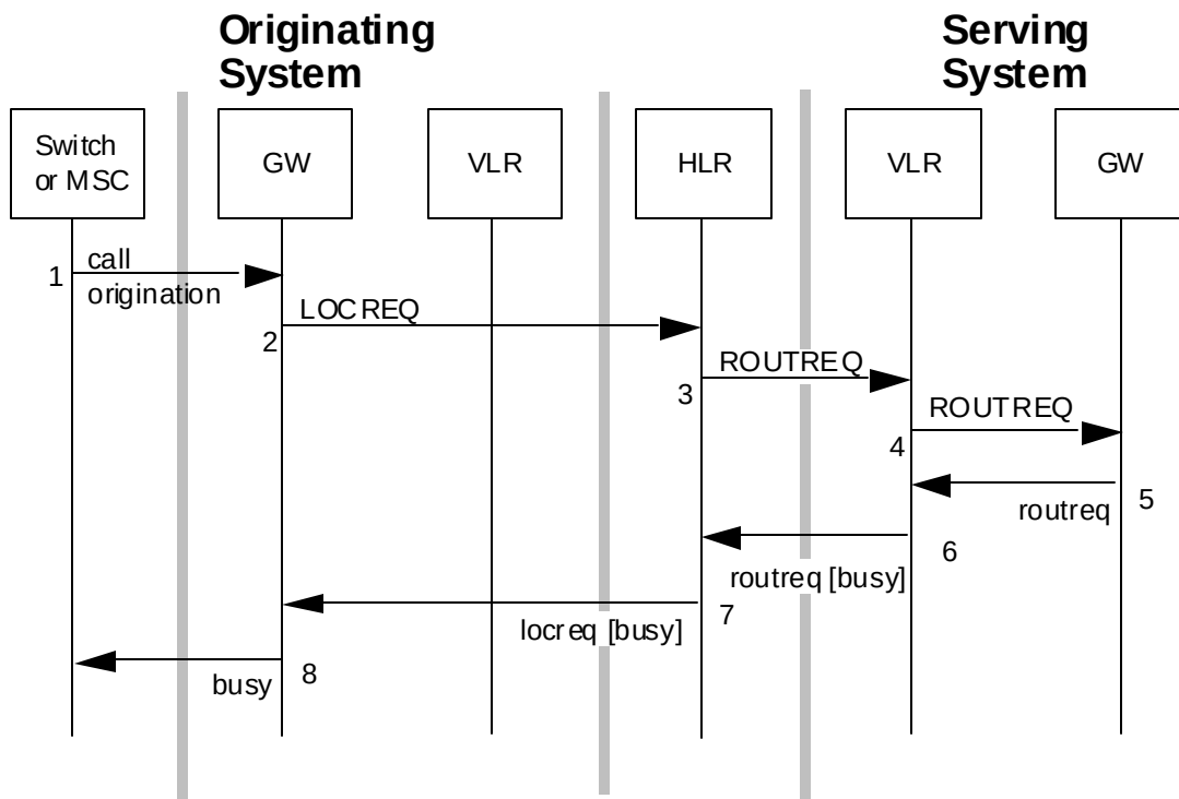
Figure 6-3 Roaming Call Delivery - Subscriber Busy
