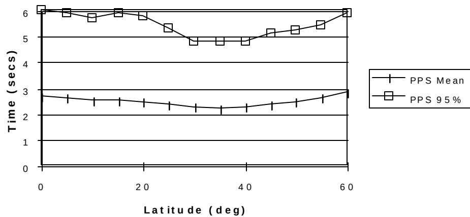
Figure 4-2 Acquisition Time as a function of Latitude
