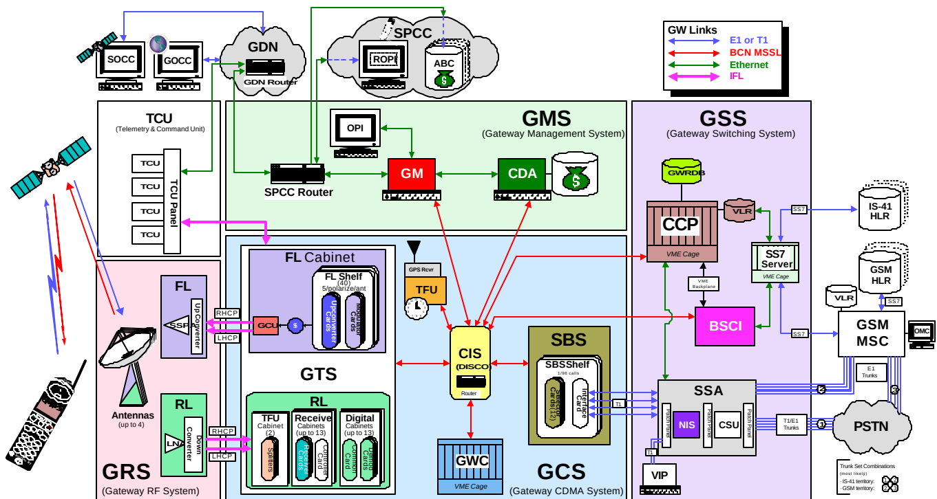
2 Figure 2-8 Gateway Simplified Block Diagram
