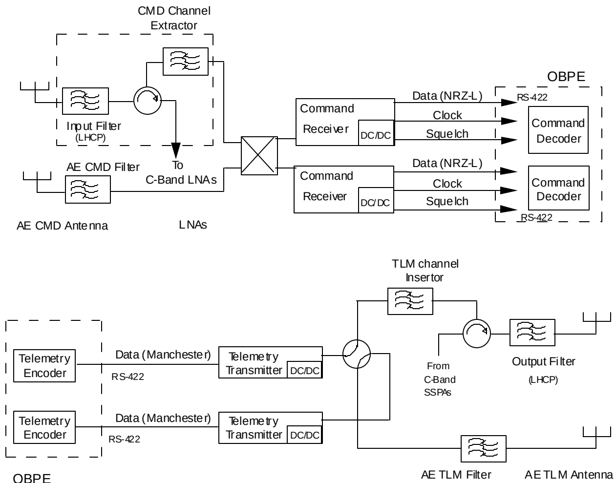
Figure 2-16 Satellite T&C - Compatible with Communications
