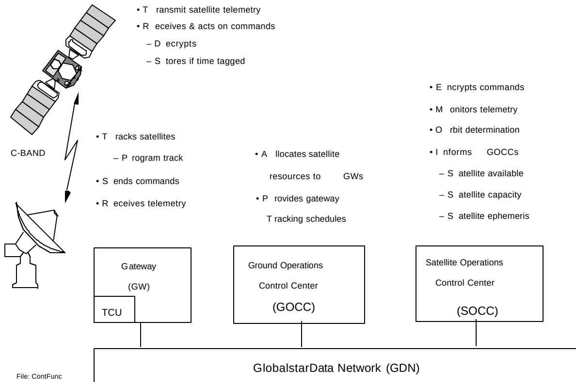
Figure 2-12 Ground Equipment Support for T&C Functions
