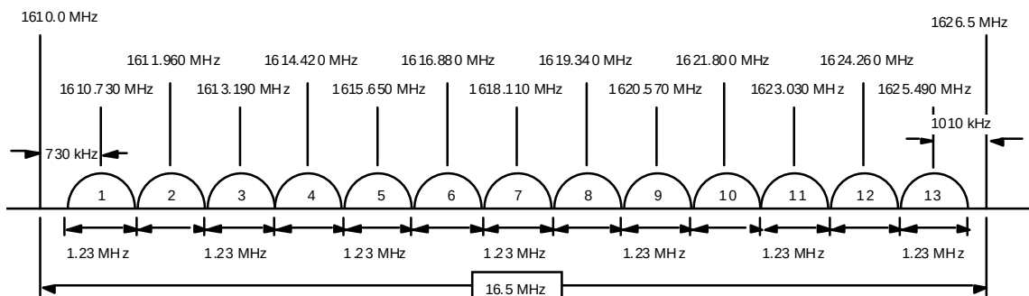
Figure 3-4 L - Band Channel
