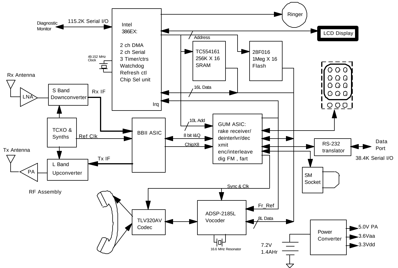
Figure 2-4 Globalstar User Terminal Block Diagram
