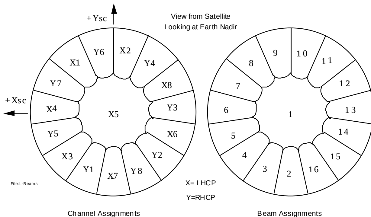
Figure 3-3 L- Band Beams
