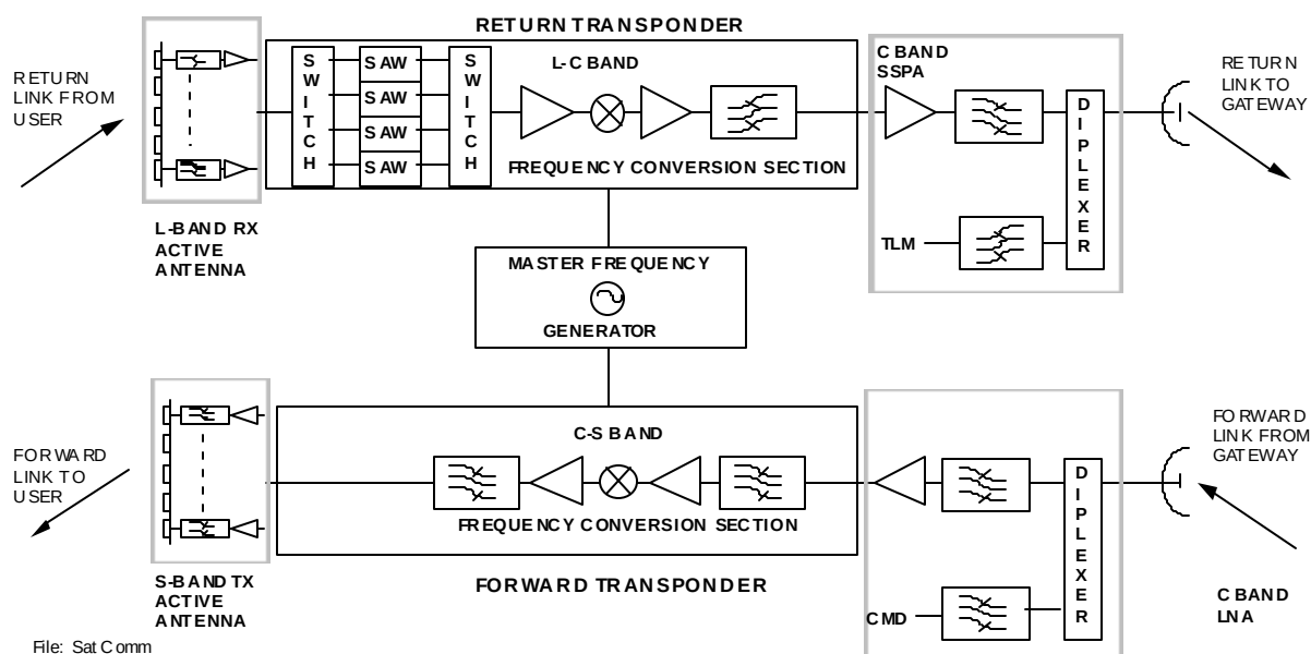
Figure 2-15 Communications Payload Simplified Block
