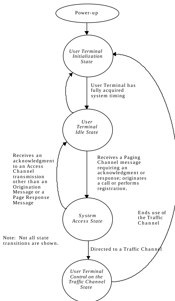
Figure 2-5 User Terminal Startup Scenario within Globalstar
