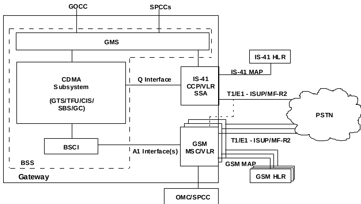
Figure 5-1 Gateway Architecture
