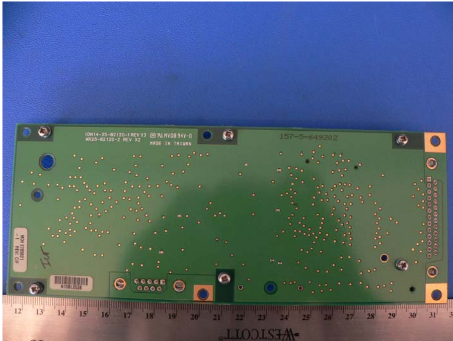
Data modem board 2 Solder side View
