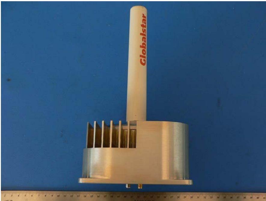
Antenna End View
