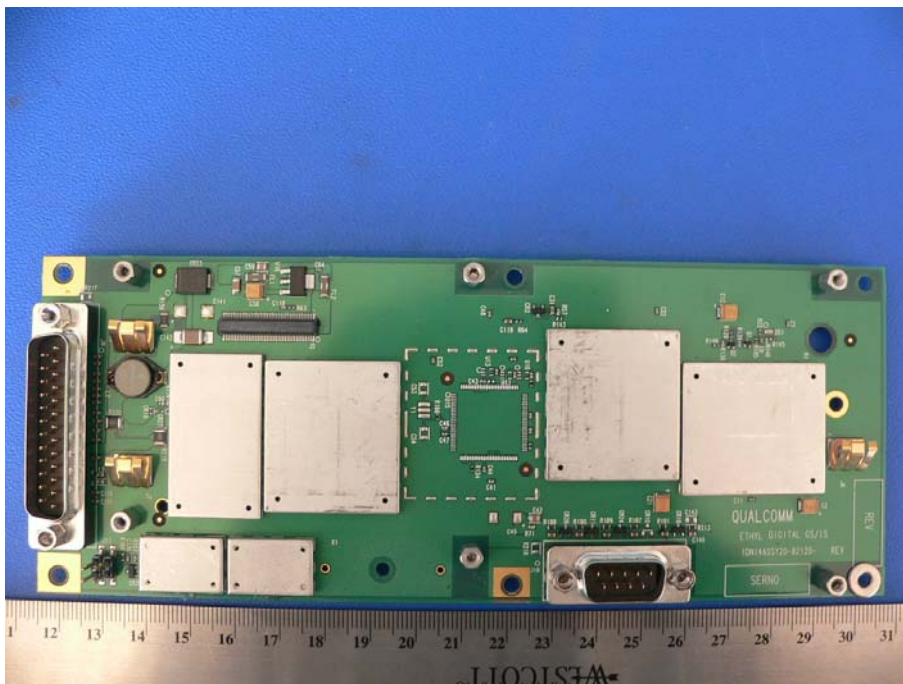
Data modem board 2 Component side View
