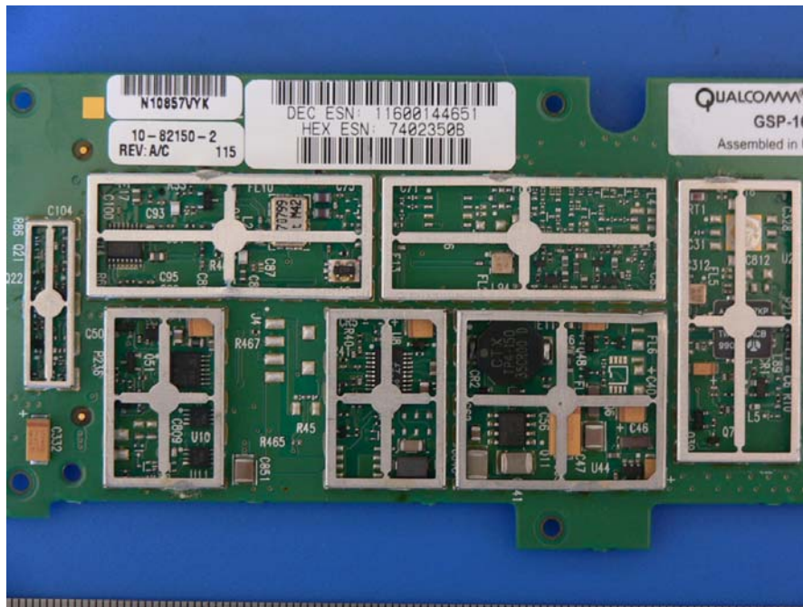
RF Shielding Off View 1
