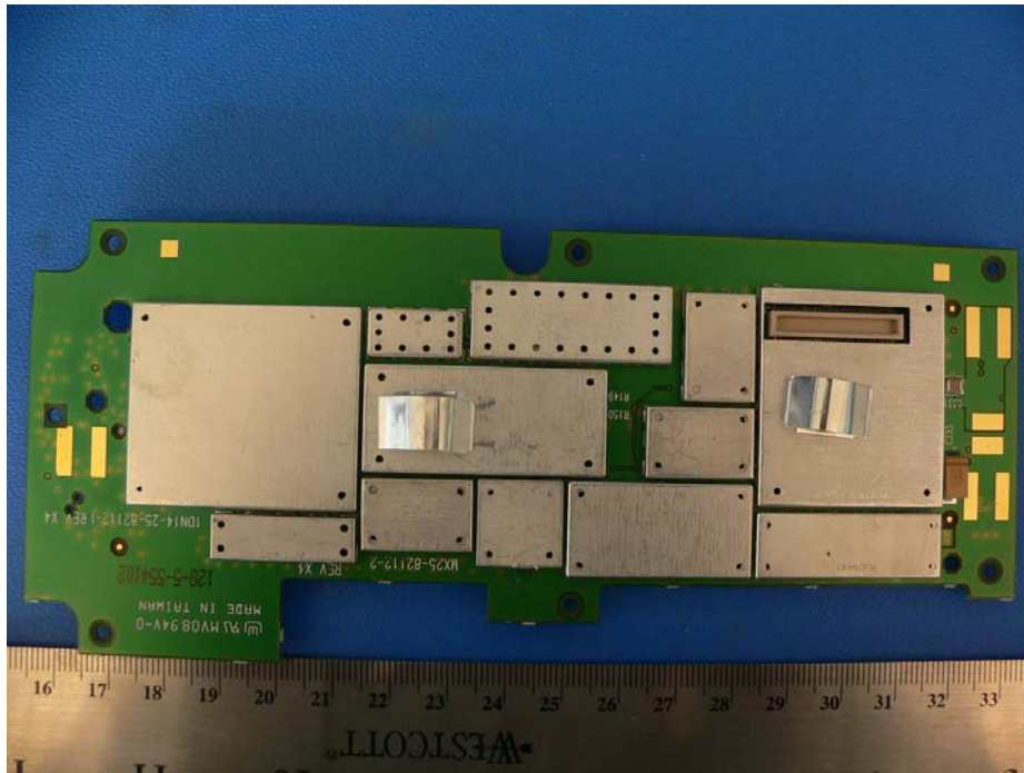
Data modem Solder side View
