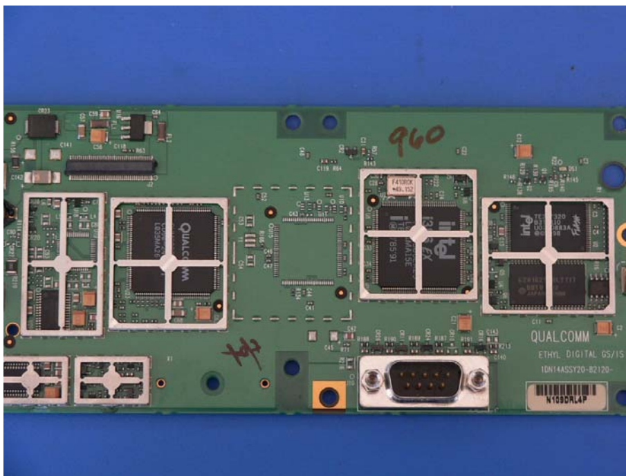
RF Shielding Off View 3
