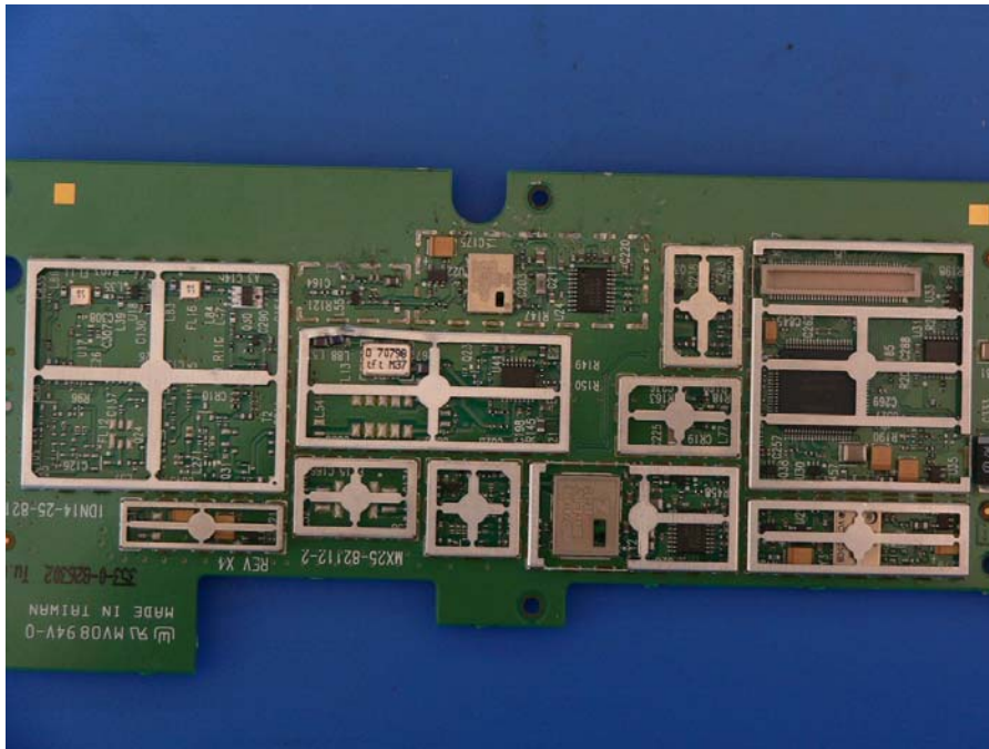
RF Shielding Off View 2
