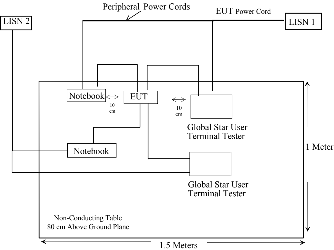
Test Setup Block Diagram
