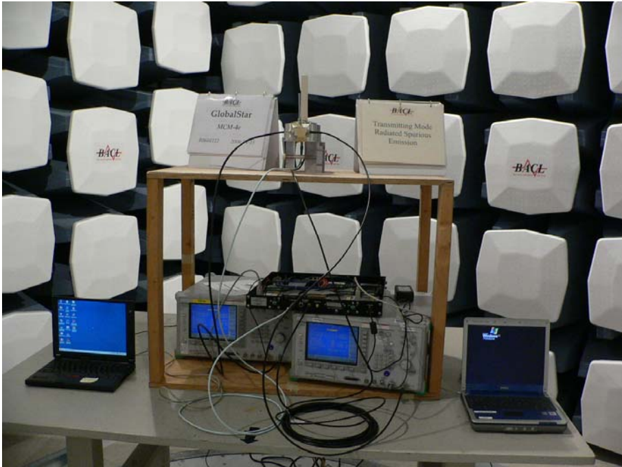
Radiated Setup – Transmitter – Front View
