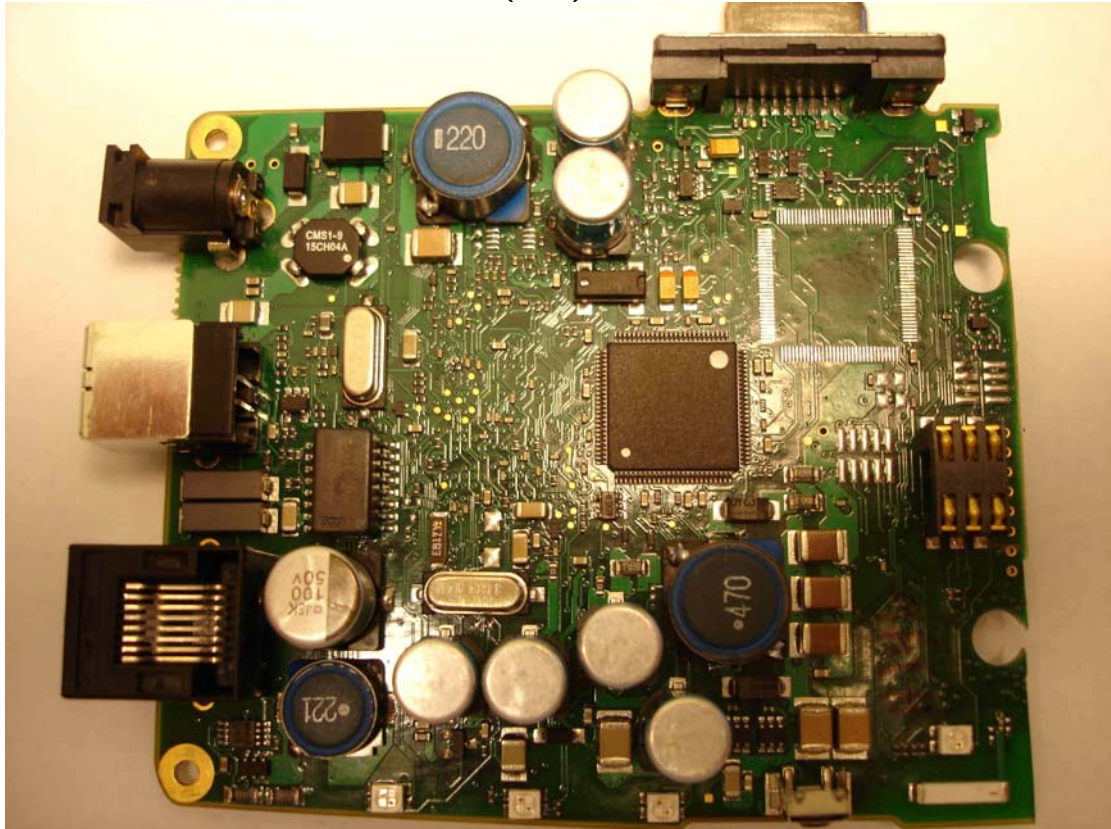
Nera WorldPro 1000 Interface unit (IDU)
