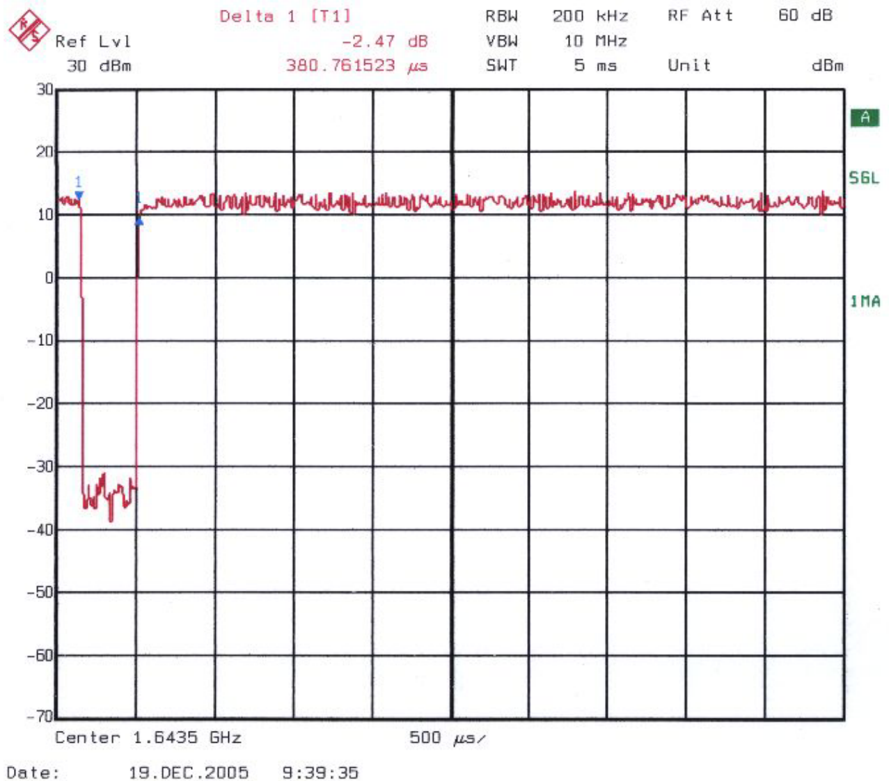
Fig 8 Duty cycle
