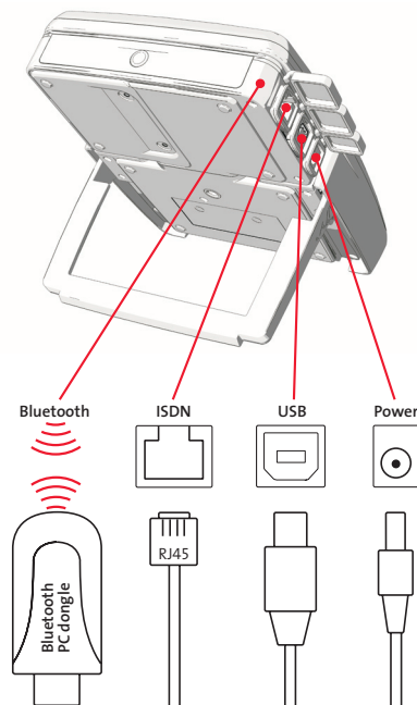
Figure 4 Nera WorldPro1000 connectors.
