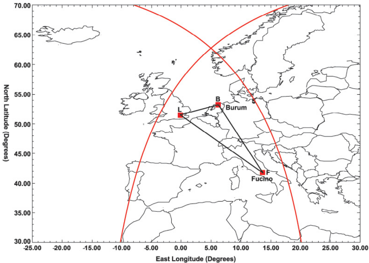
Figure A-3 BGAN Satellite Access Station.
