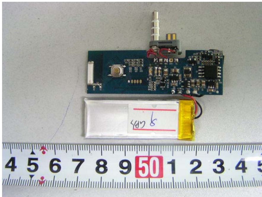
EUT – Inside View (5)
