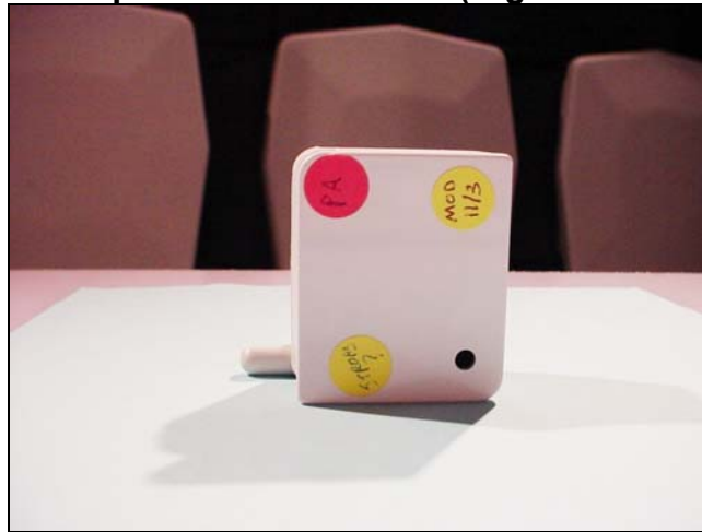
View of the EUT setup in Side orientation (Highest emissions measured)
