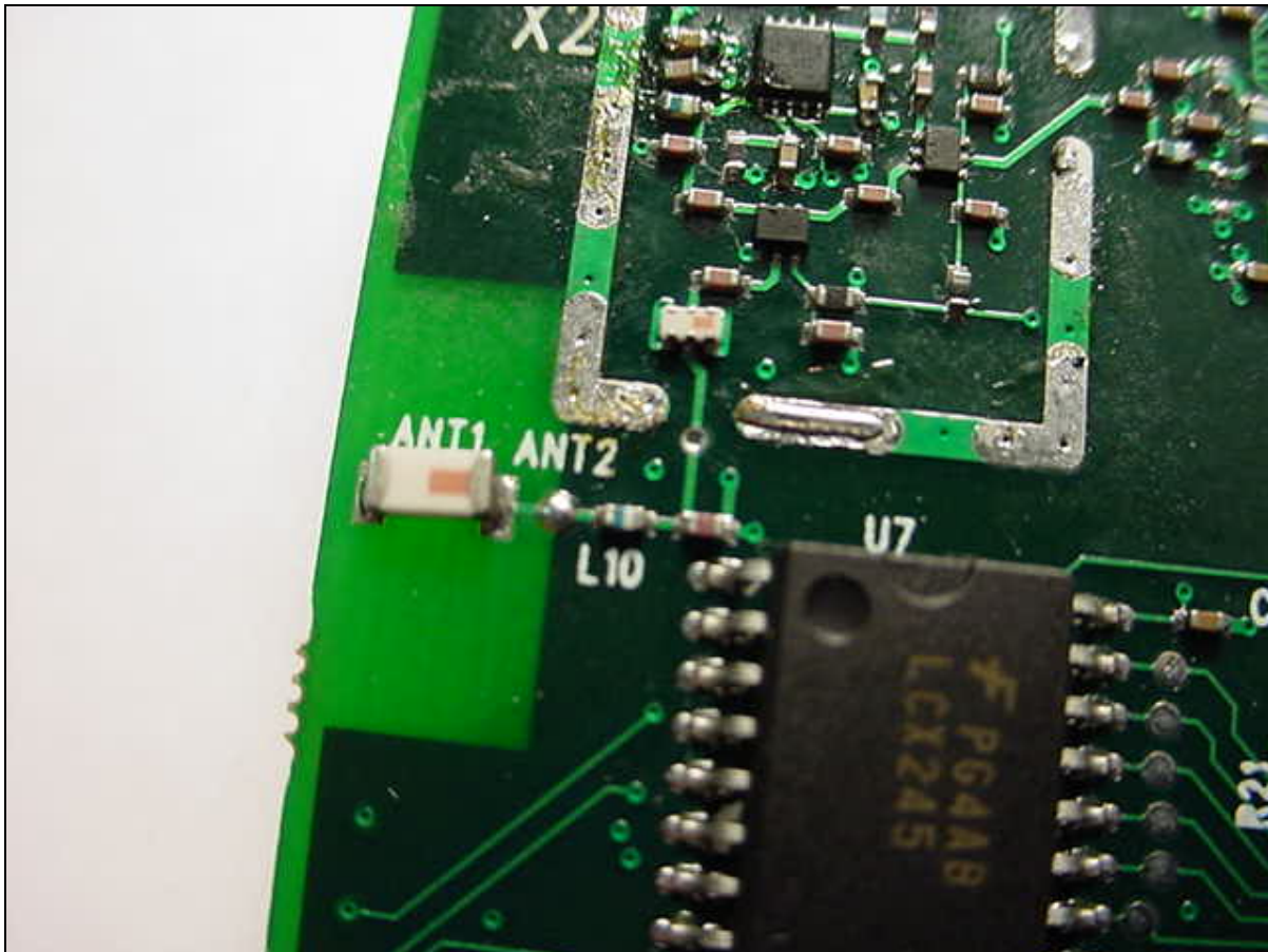
Photo Six – Internal Chip Antenna
