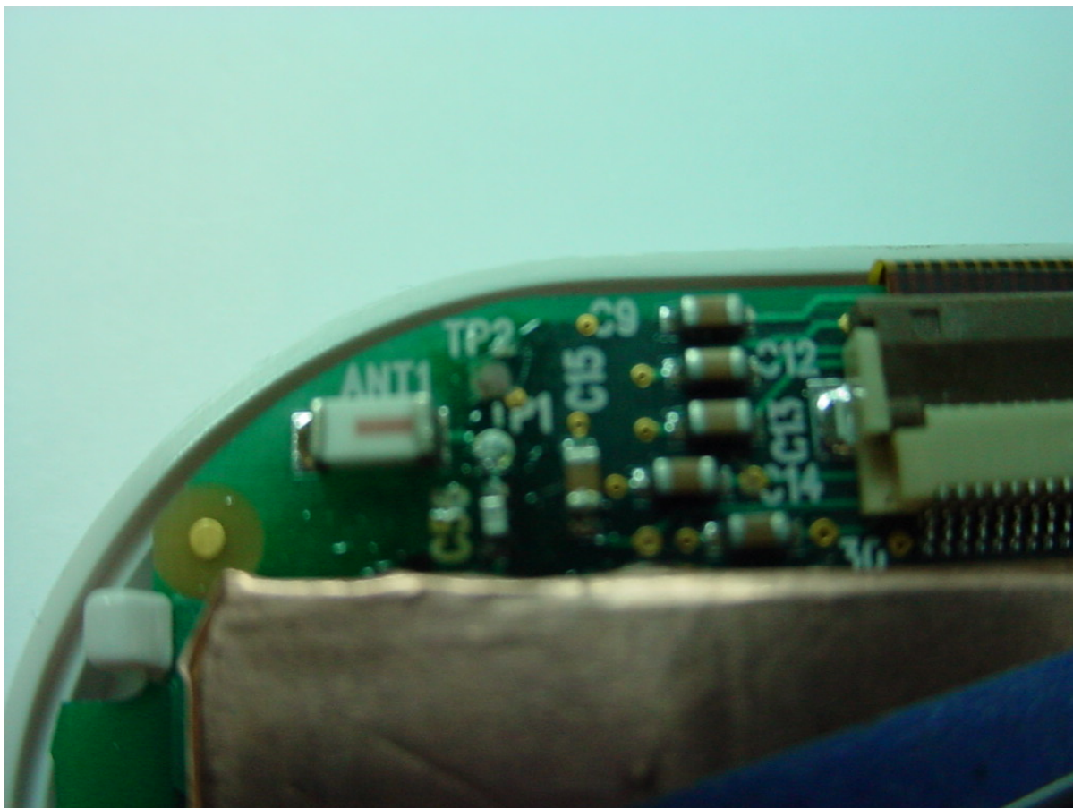
Photo Six – Internal Close-up of Antenna
