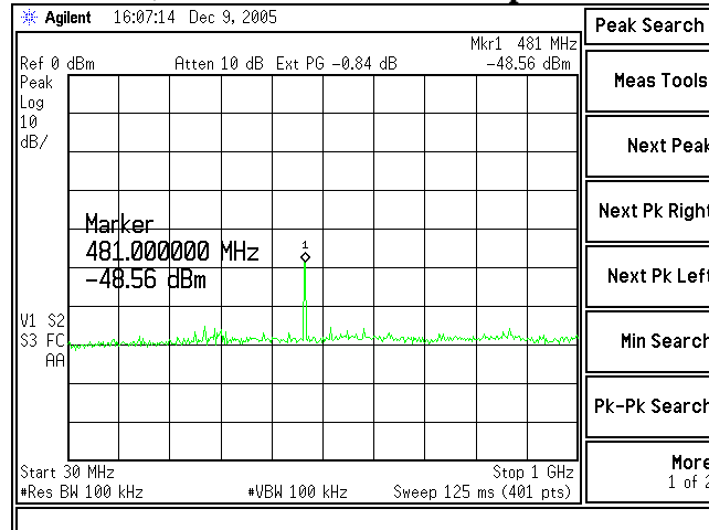
Channel 7, shown from 30 MHz up to 1000 MHz
