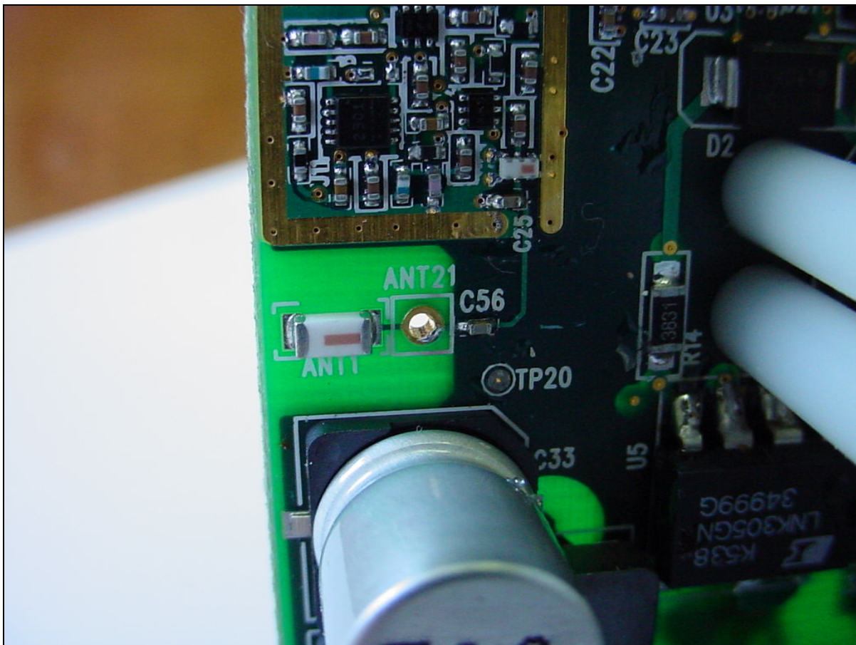
Photo Five – Internal Close-Up of Surface Mount Antenna
