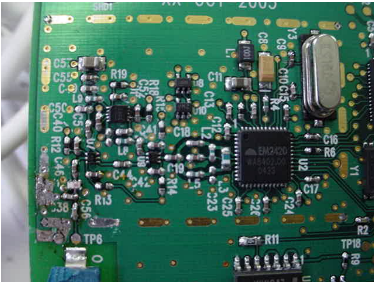
Photo Four – Internal Close Up of RF Section
