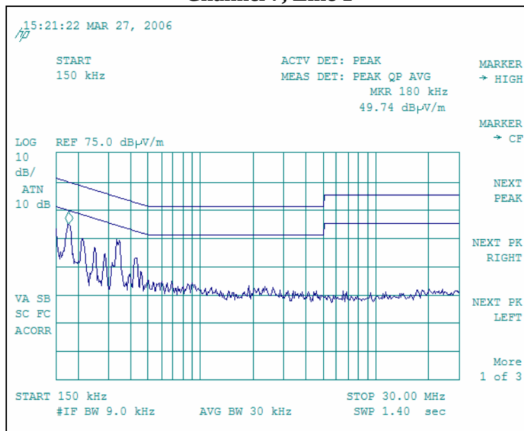
Channel 7, Line 1
