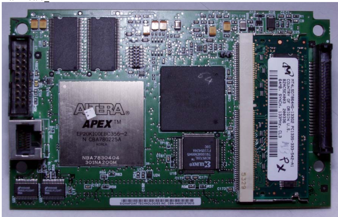
Main Board_2
