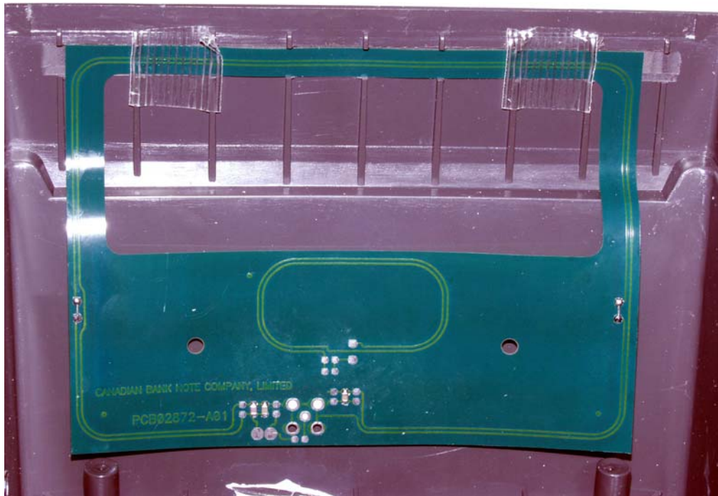
Modular Loop Antenna (Secondary):
