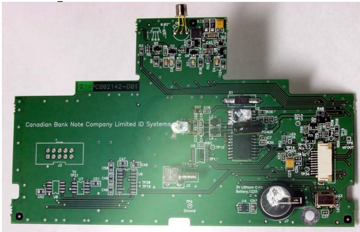
User Interface_1
