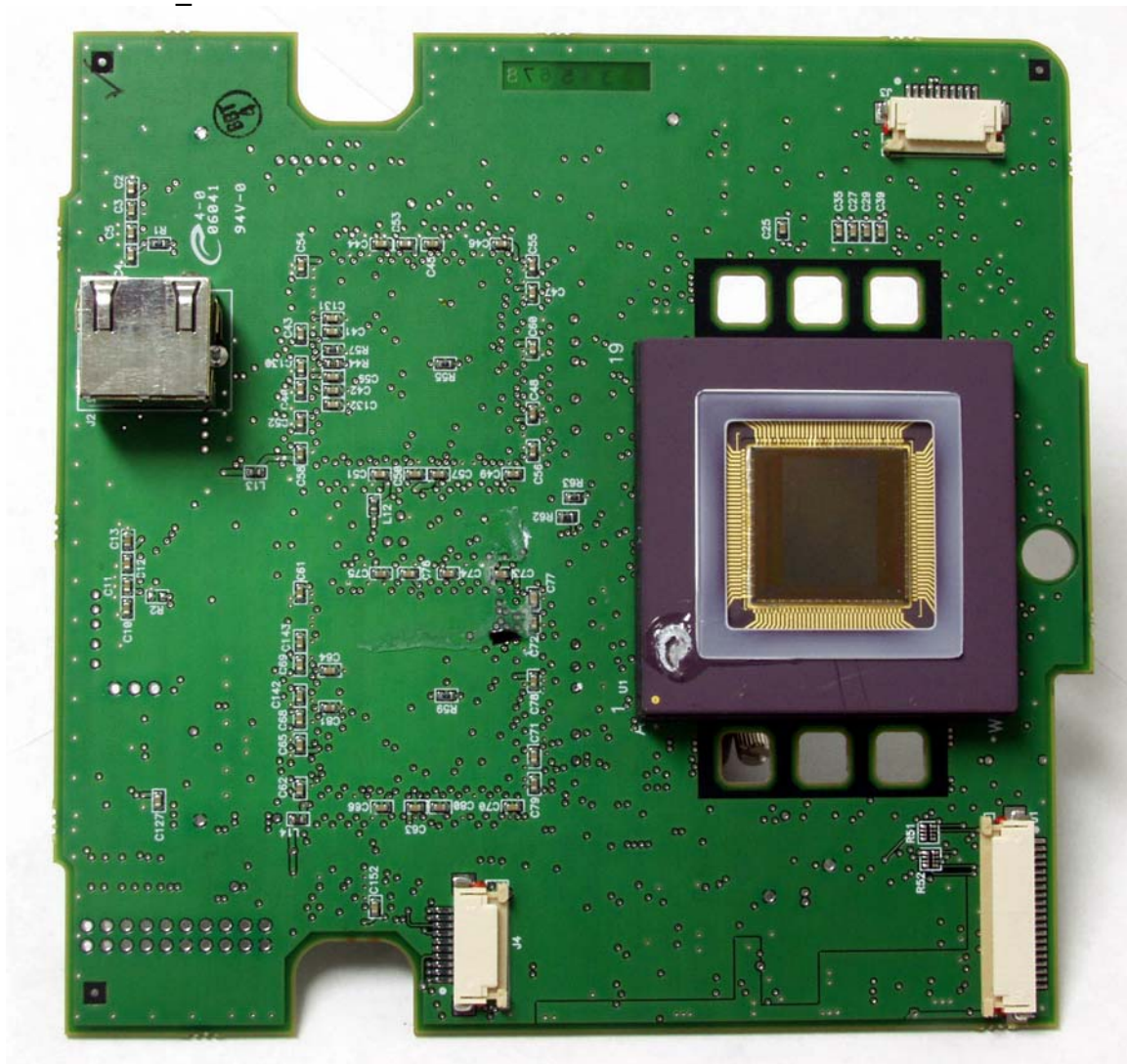
Sensor Board_2
