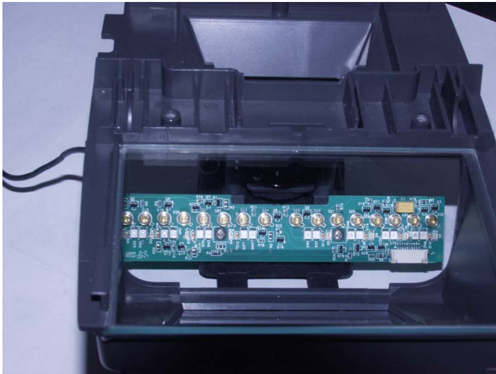
LED-board:
