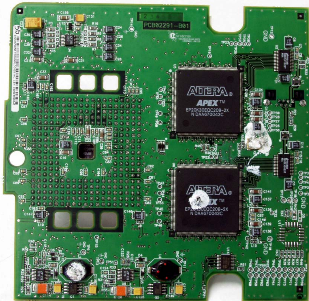
Sensor Board_1
