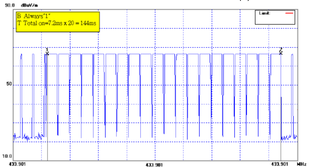
Plot For Total Duration of EUT at active state: T_{(on)}
