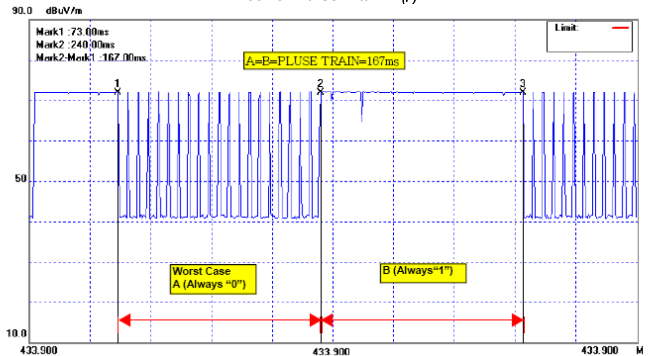
Plot For Pulse Train: T_{(P)}
