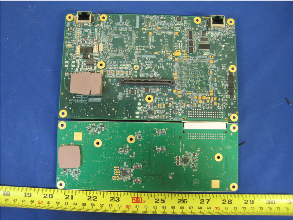
Solder View
