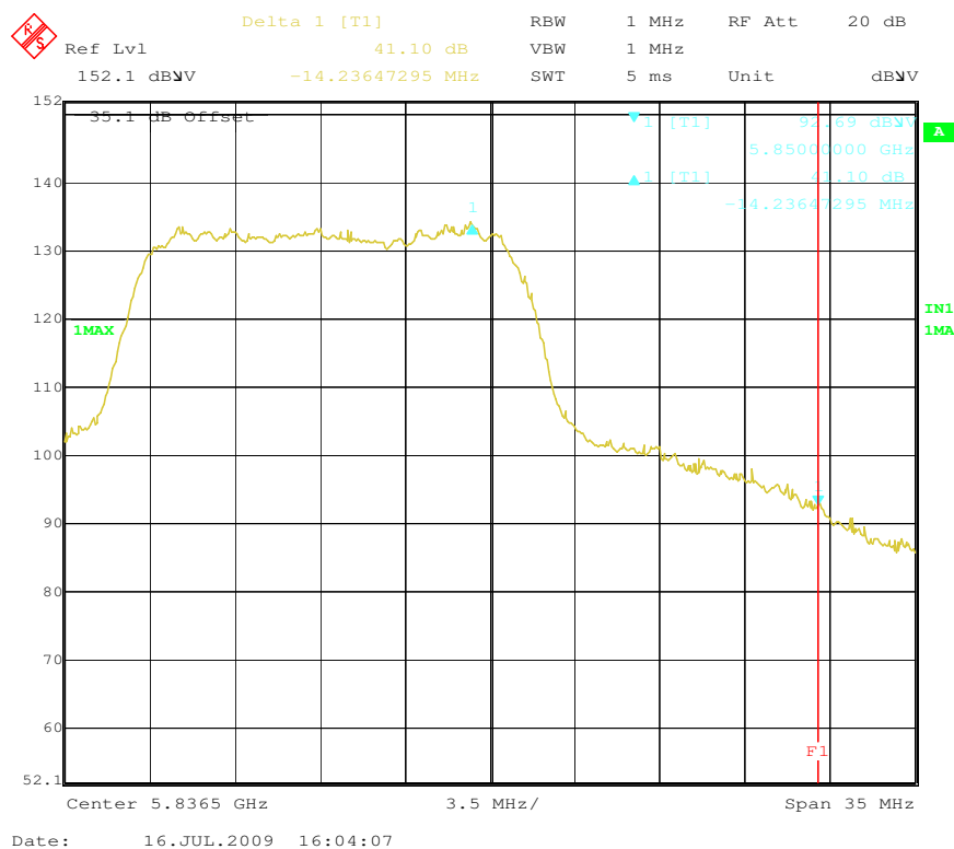
High Channel (16MHz Mode 1)
