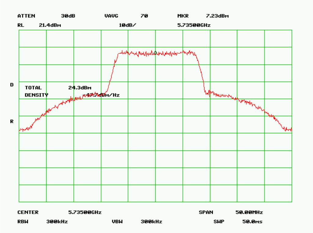
Low Channel (16MHz Mode 2)
