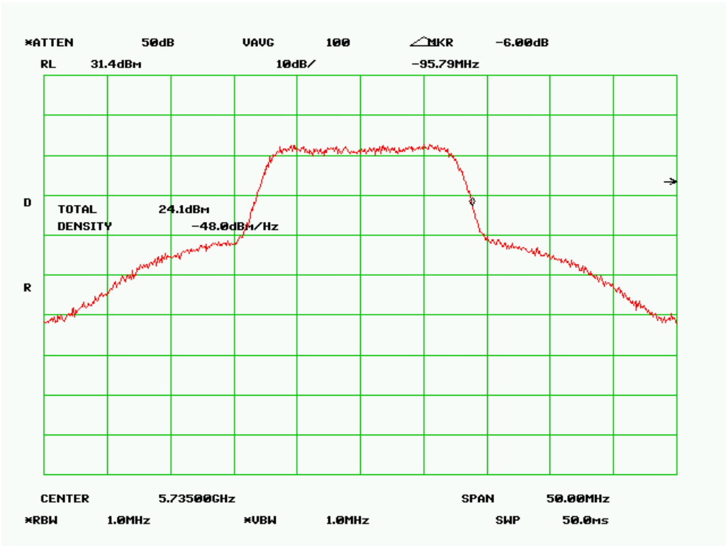
Low Channel (16MHz Mode 3)
