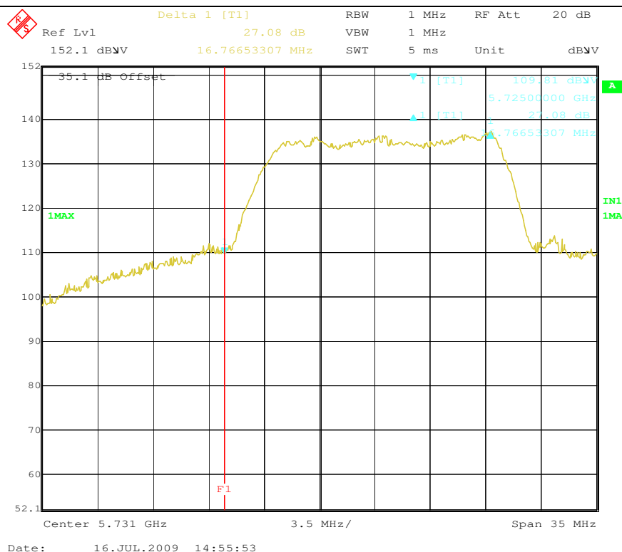
Low Channel (16MHz Mode 3)
