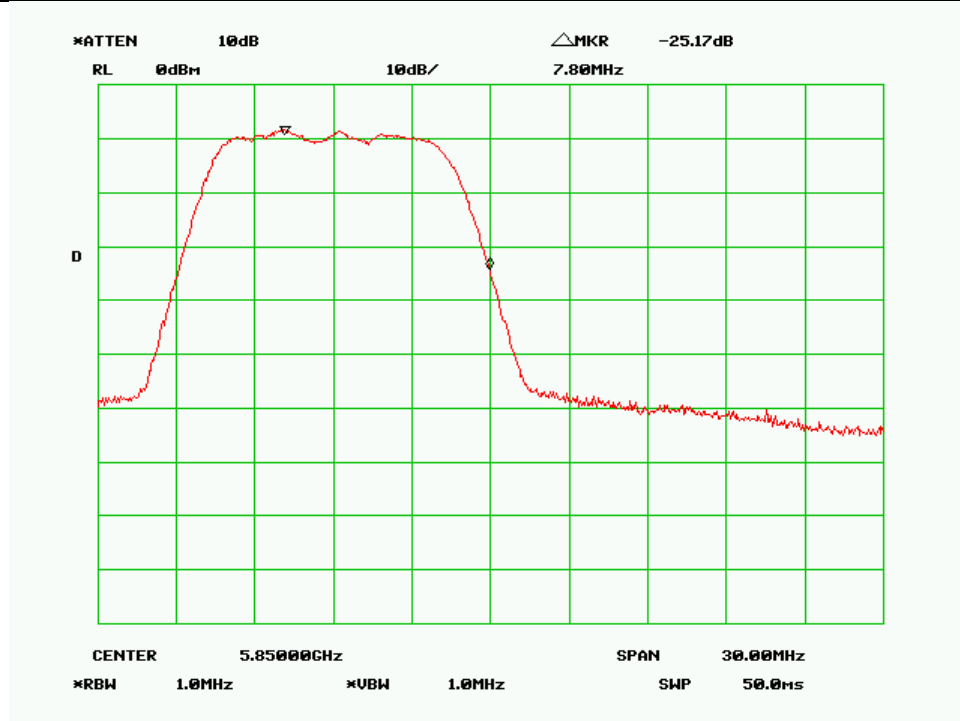
High Channel-10MHz, 256QAM, Horizontal Polarity
