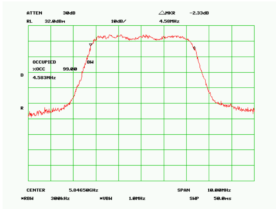
99% Bandwidth – High Channel (5MHz 256QAM Mode)
