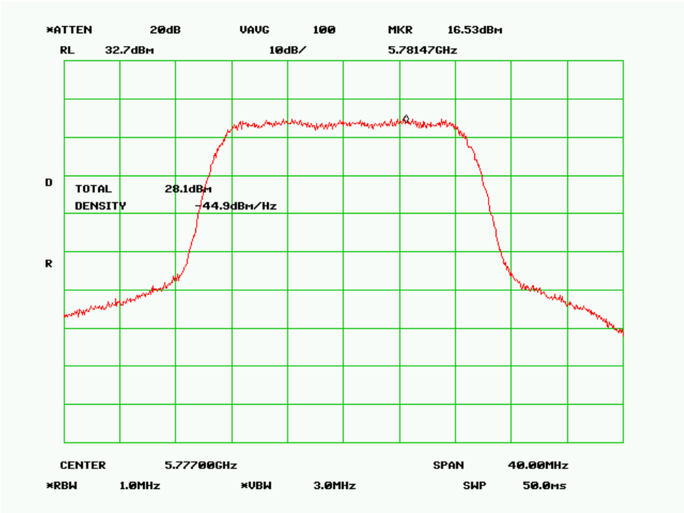
Mid Channel (20MHz 256QAM Mode)
