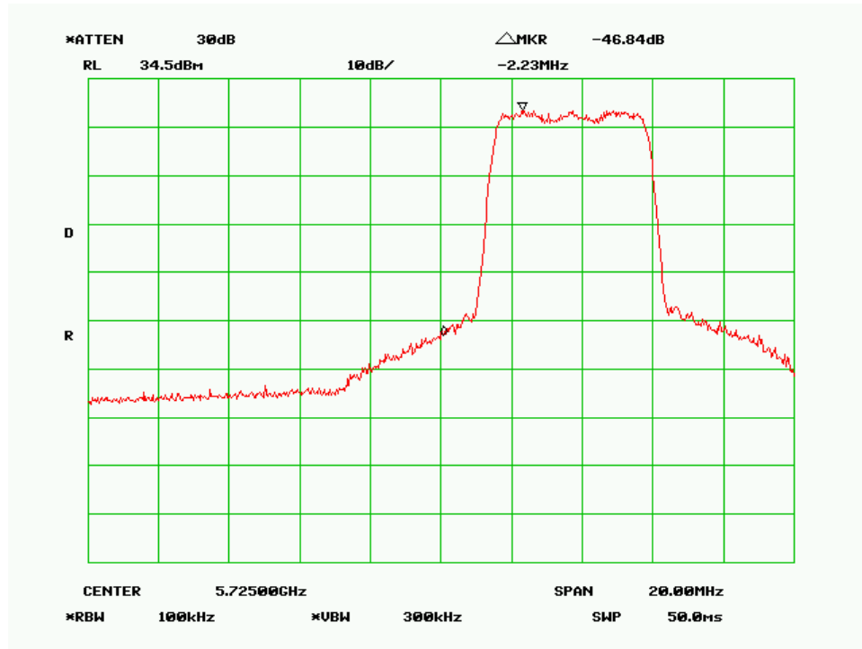
Low Channel-5MHz, 256QAM
