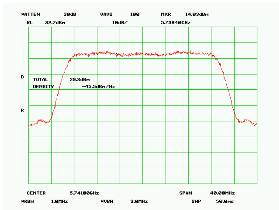
Low Channel (30MHz QPSK Mode)
