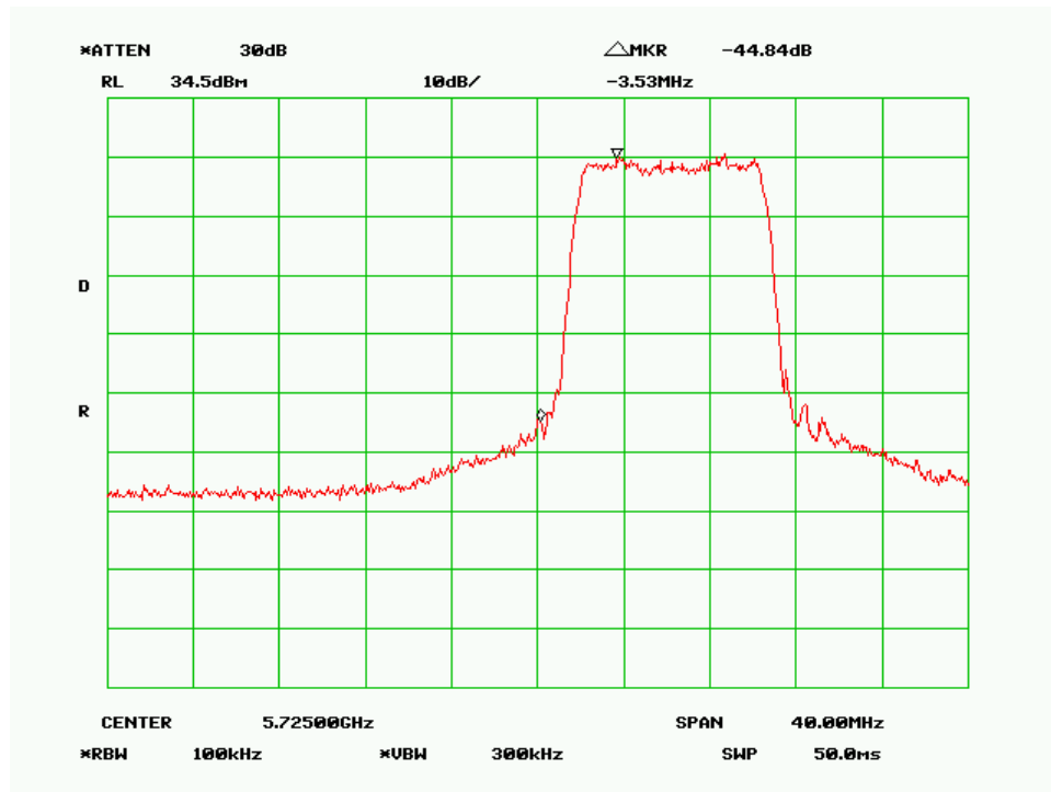
Low Channel-10MHz, QPSK
