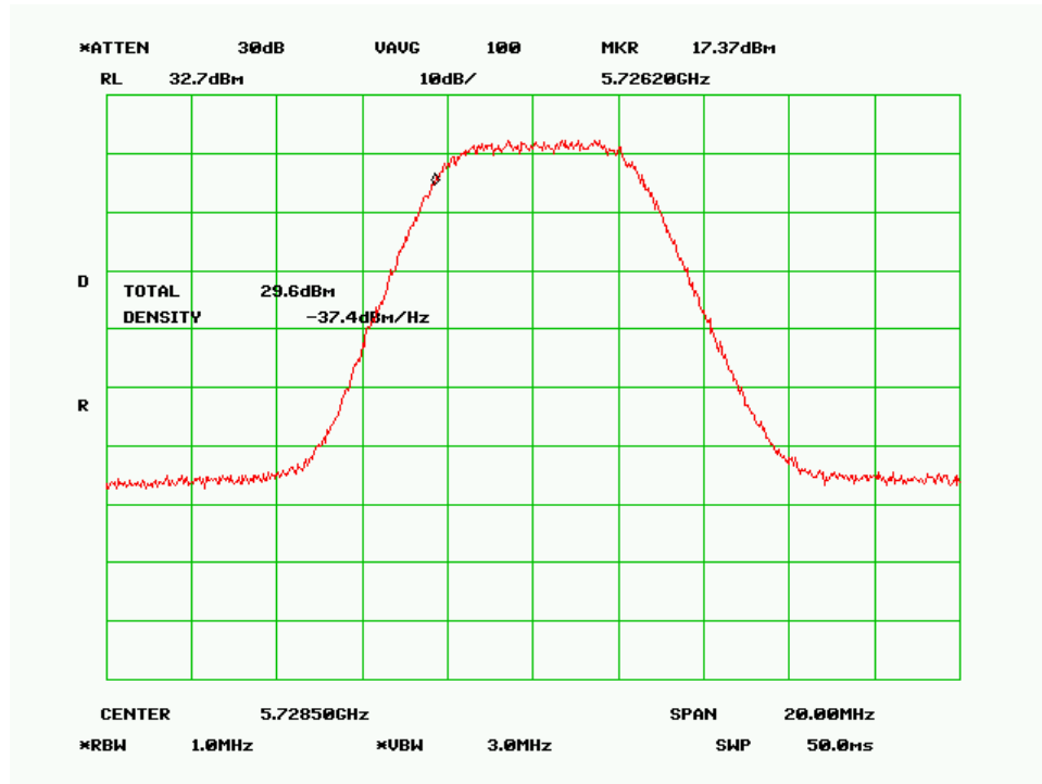
Low Channel (5MHz QPSK Mode)
