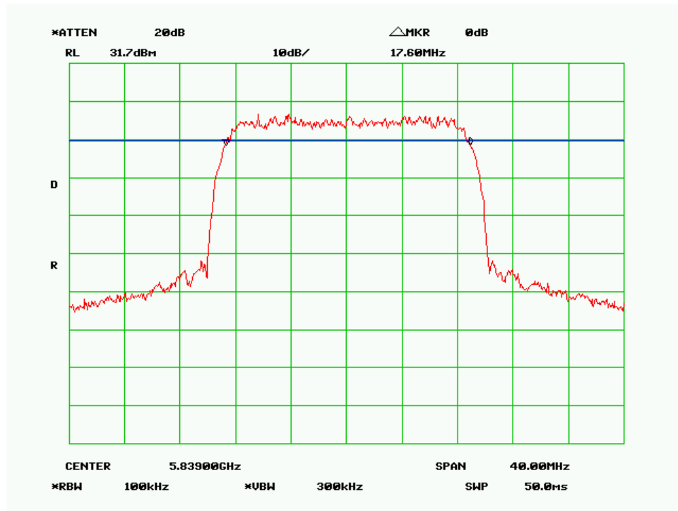
6dB Bandwidth – High Channel (20MHz 256QAM Mode)
