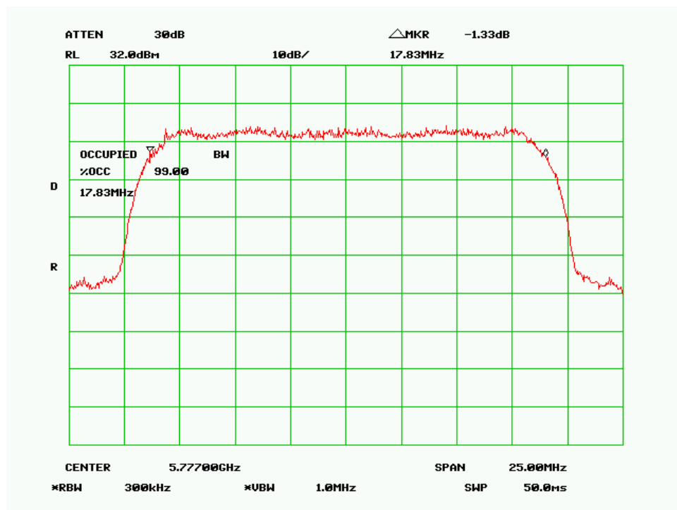
99% Bandwidth - Mid Channel (20MHz QPSK Mode)
