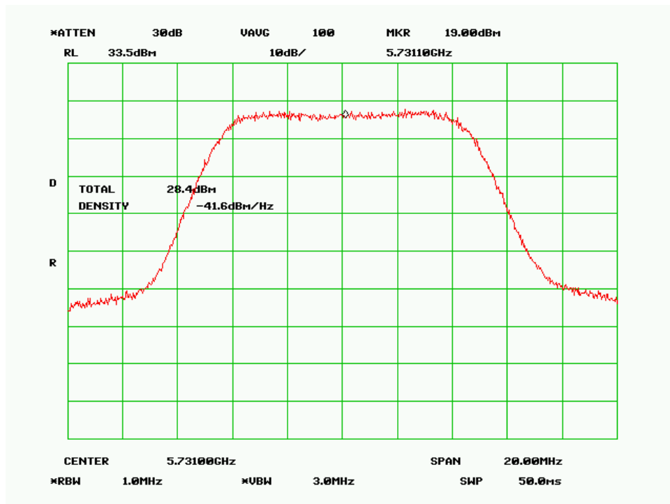
Low Channel (10MHz 256QAM Mode)
