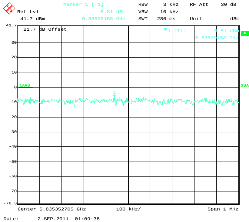
High Channel (20MHz 256QAM Mode)
