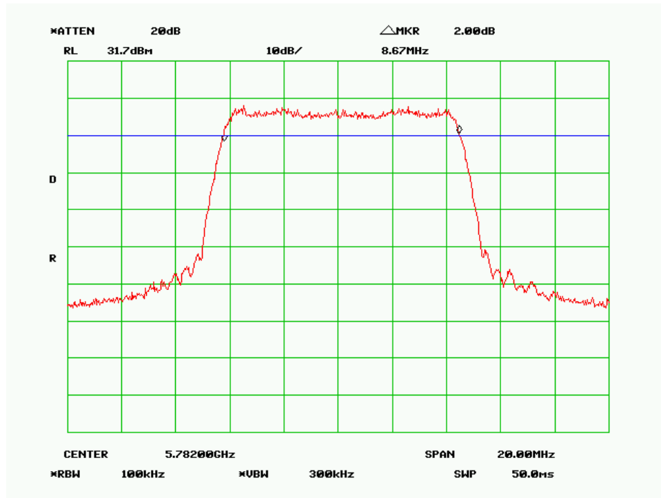
6 dB Bandwidth – Mid Channel (10MHz 256QAM Mode)
