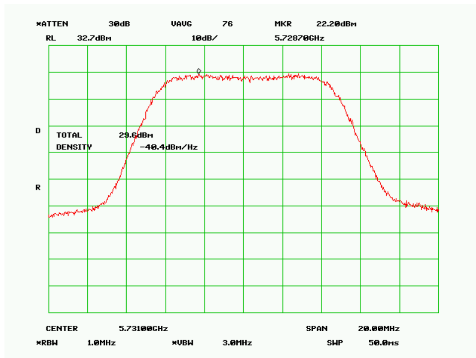
Low Channel (10MHz QPSK Mode)
