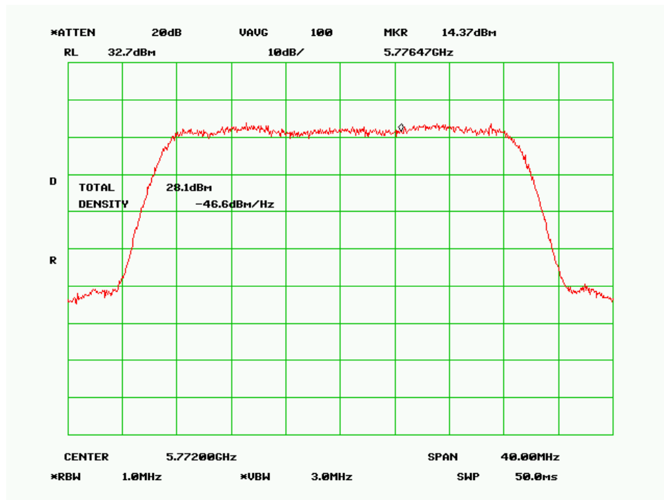
Mid Channel (30MHz 256QAM Mode)
