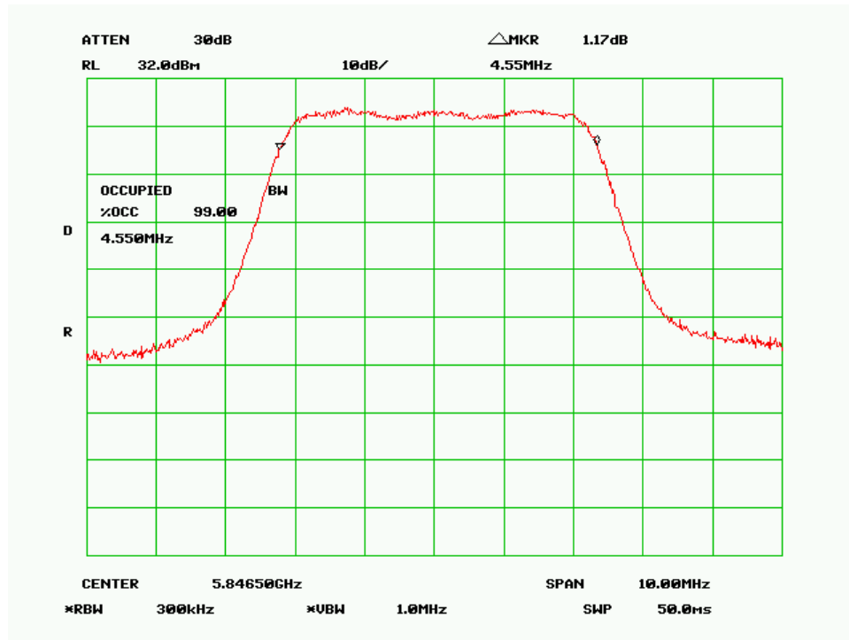
99% Bandwidth – High Channel (5MHz QPSK Mode)
