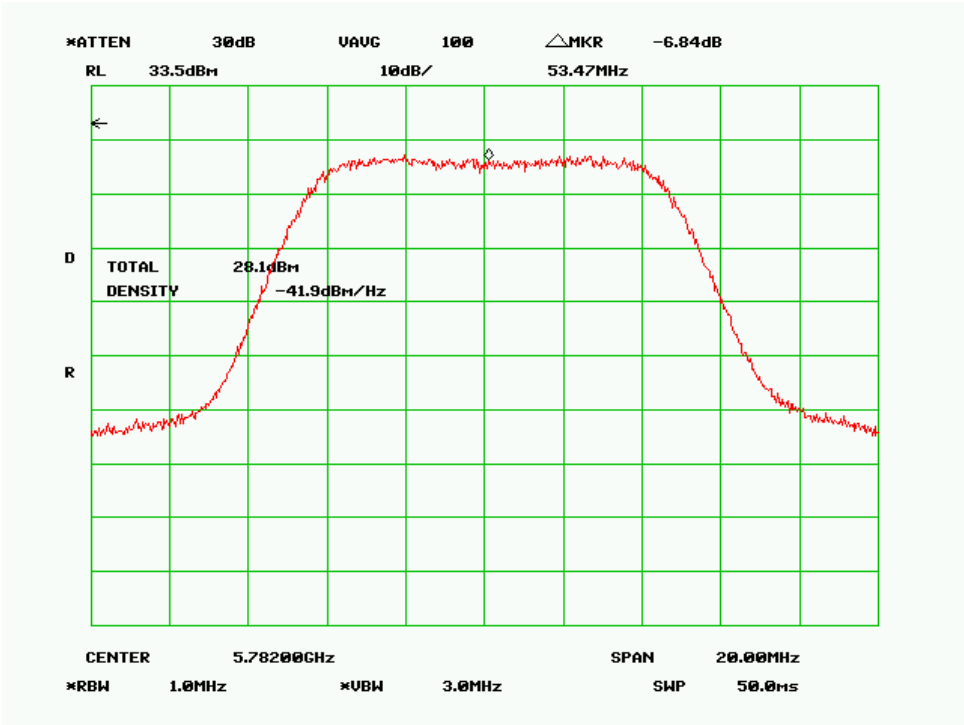
Mid Channel (10MHz 256QAM Mode)
