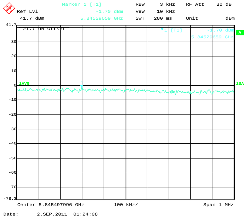
High Channel (5MHz 256QAM Mode)
