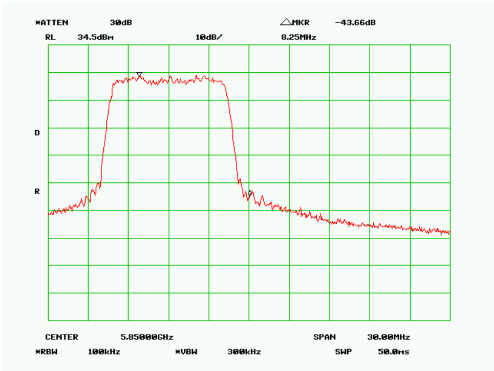
High Channel-10MHz, 256QAM
