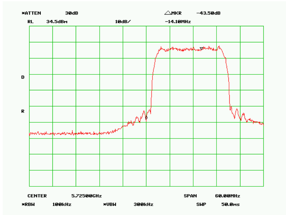
Low Channel-20MHz, 256QAM
