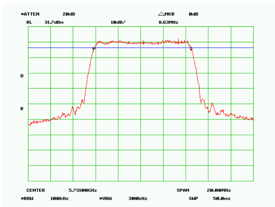
6 dB Bandwidth – Low Channel (10MHz QPSK Mode)
