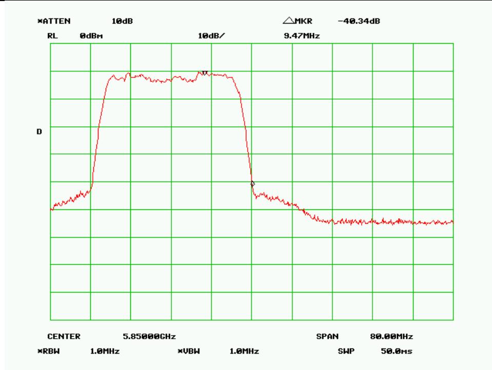
High Channel-30MHz, 256QAM, Horizontal Polarity
