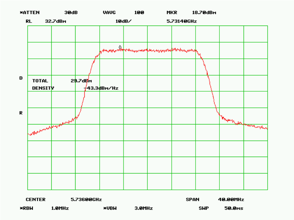
Low Channel (20MHz QPSK Mode)
