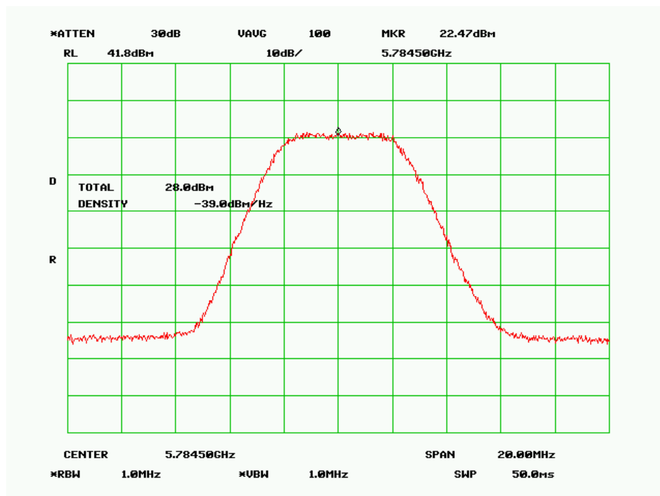
Mid Channel (5MHz 256QAM Mode)
