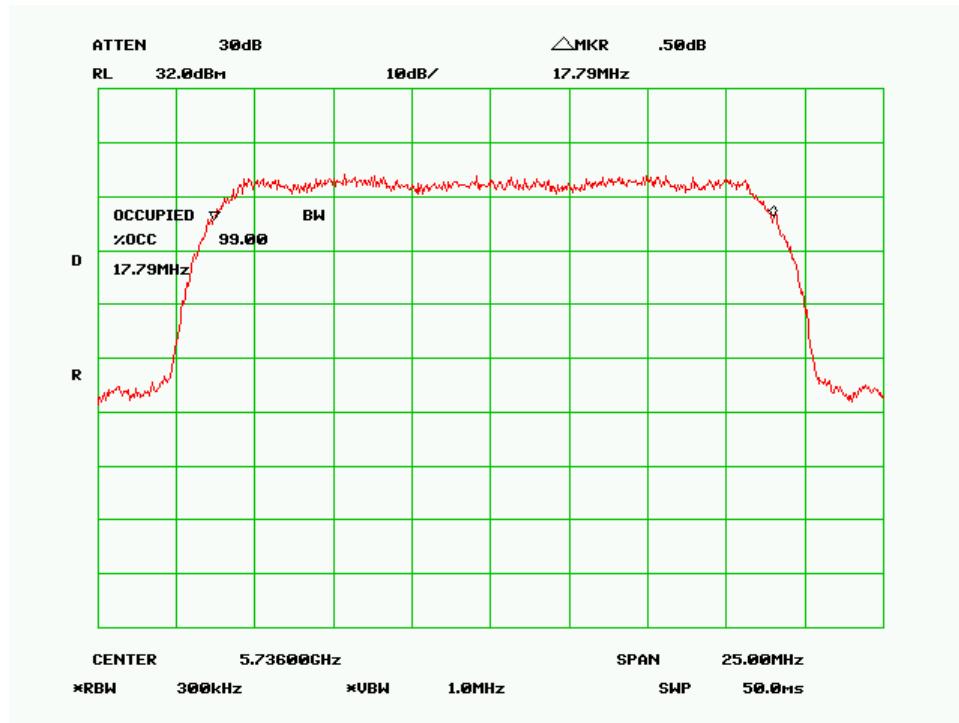
99% Bandwidth – Low Channel (20MHz 256QAM Mode)
