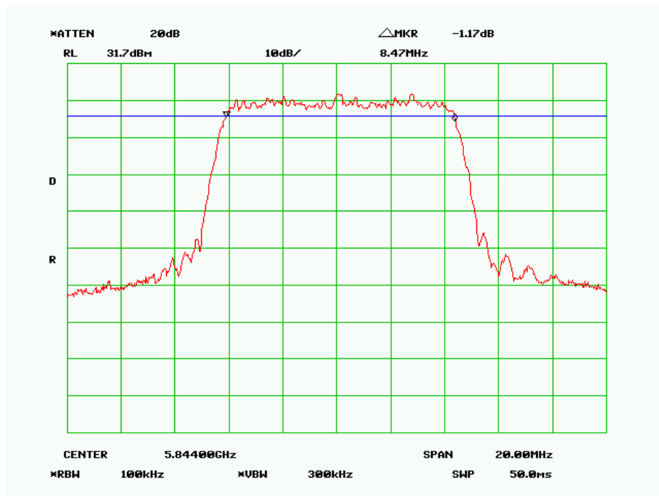
6 dB Bandwidth – High Channel (10MHz QPSK Mode)
