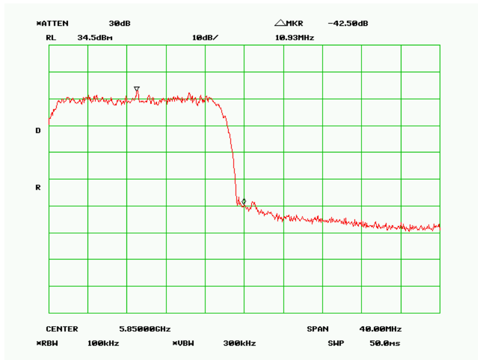
High Channel-20MHz, QPSK
