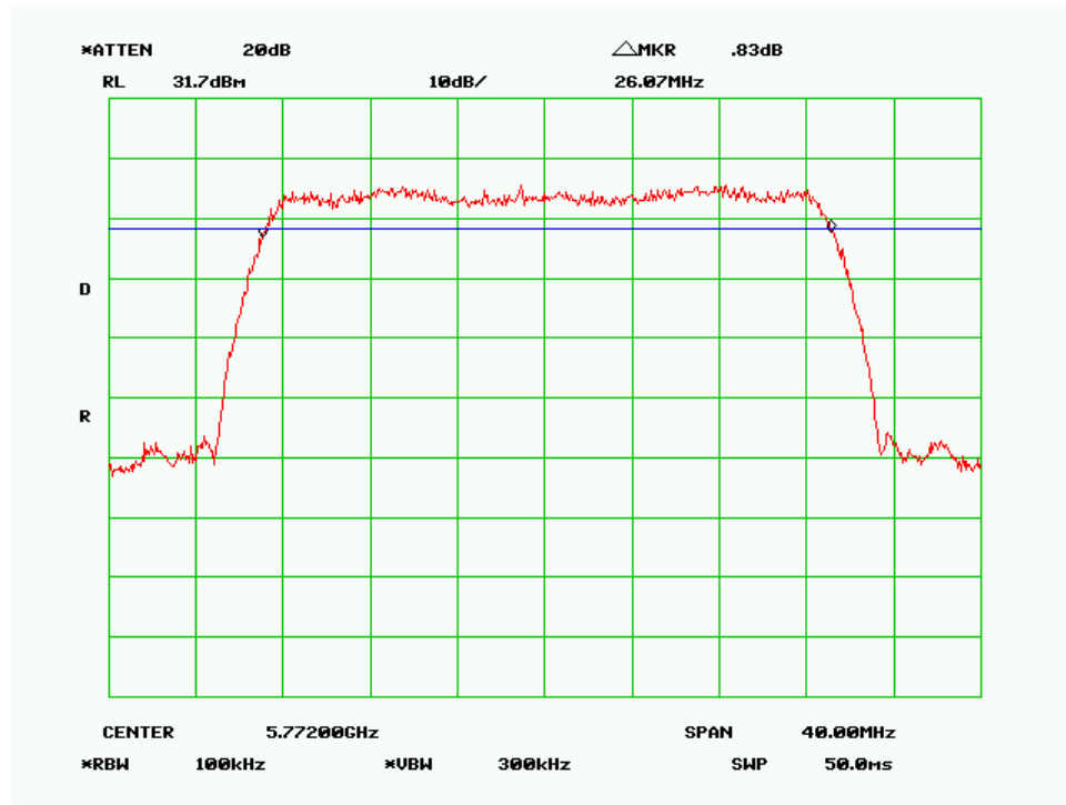
6dB Bandwidth – Mid Channel (30MHz 256QAM Mode)
