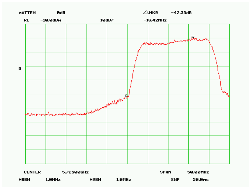
Low Channel-20MHz, 256QAM, Vertical Polarity
