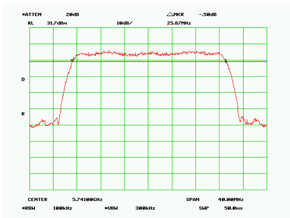
6dB Bandwidth – Low Channel (30MHz 256QAM Mode)
