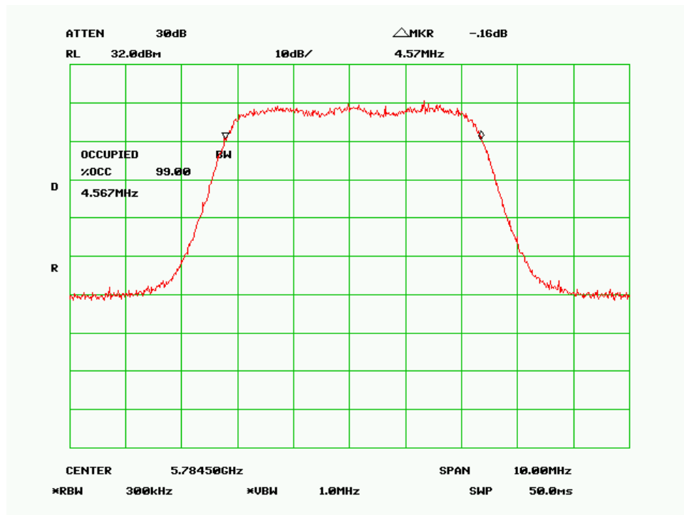
99% Bandwidth - Mid Channel (5MHz 256QAM Mode)
