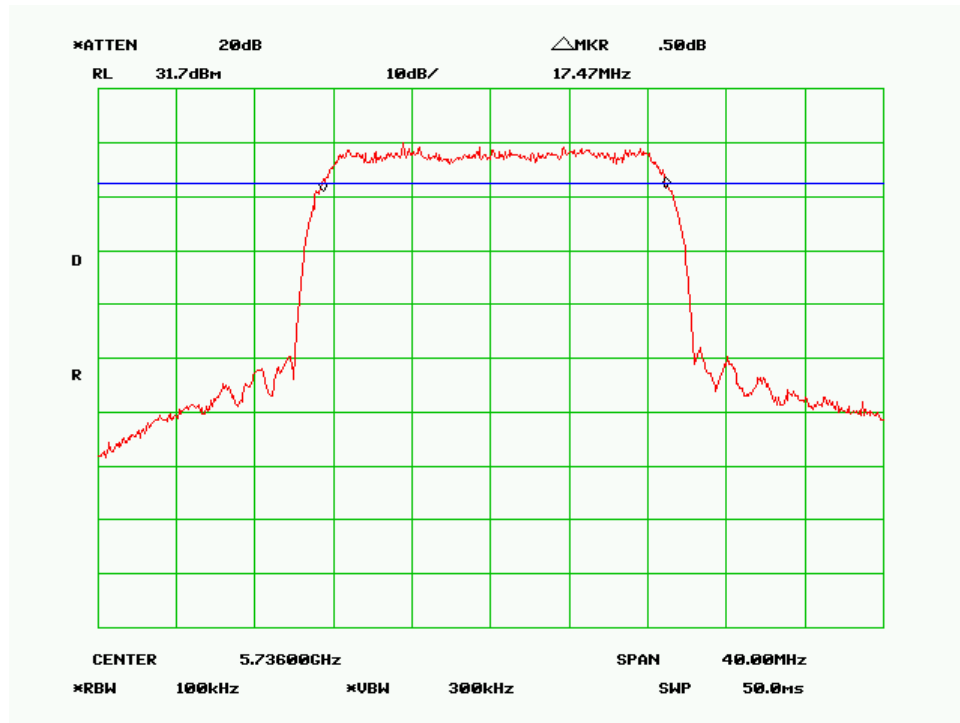
6 dB Bandwidth – Low Channel (20MHz QPSK Mode)
