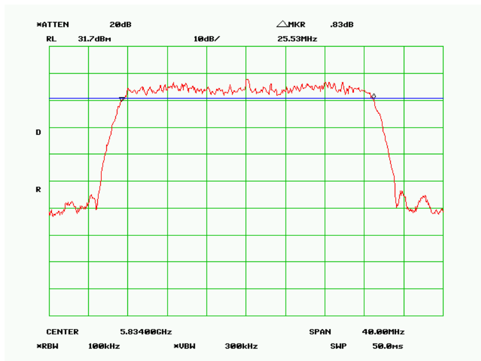
6dB Bandwidth – High Channel (30MHz QPSK Mode)
