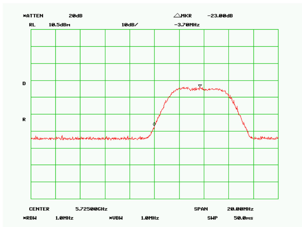
Low Channel-5MHz, 256QAM, Vertical Polarity
