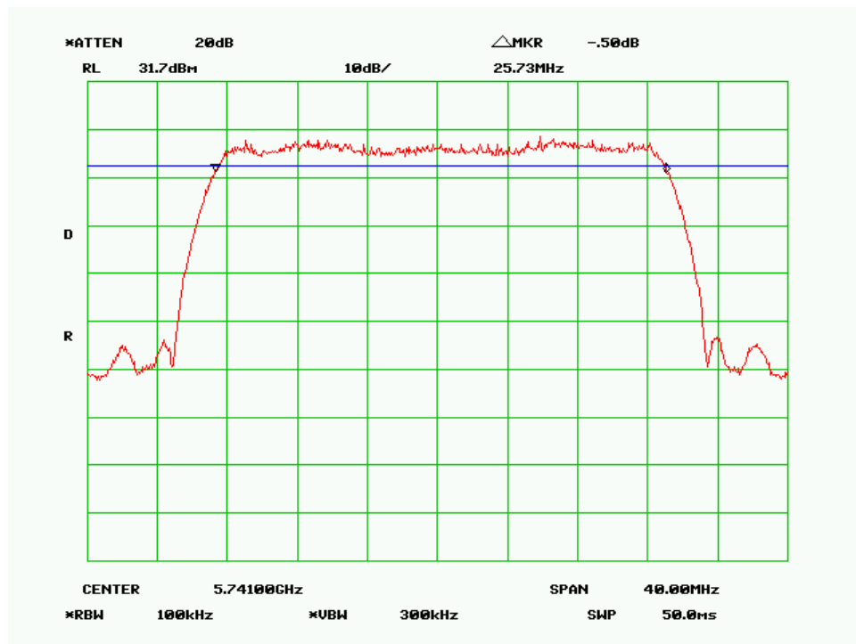
6dB Bandwidth – Low Channel (30MHz QPSK Mode)
