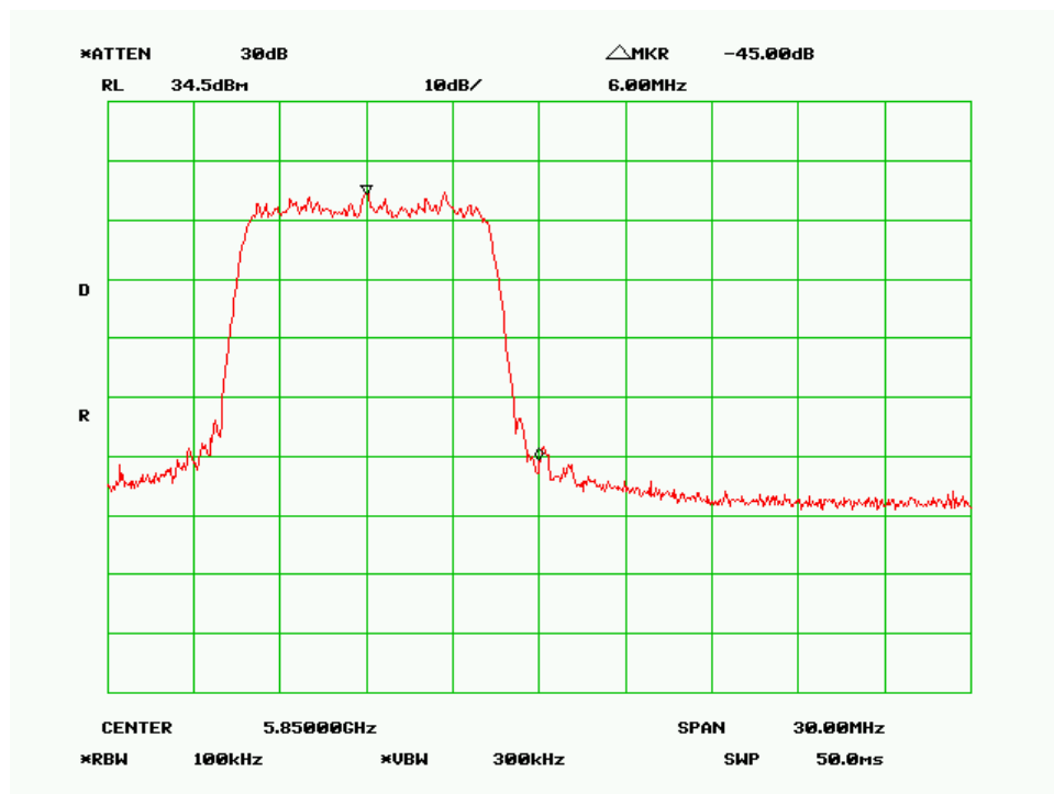
High Channel-10MHz, QPSK
