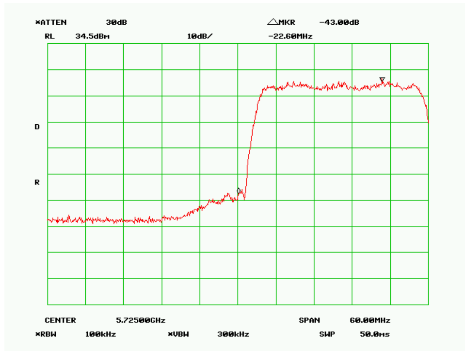
Low Channel-30MHz, 256QAM
