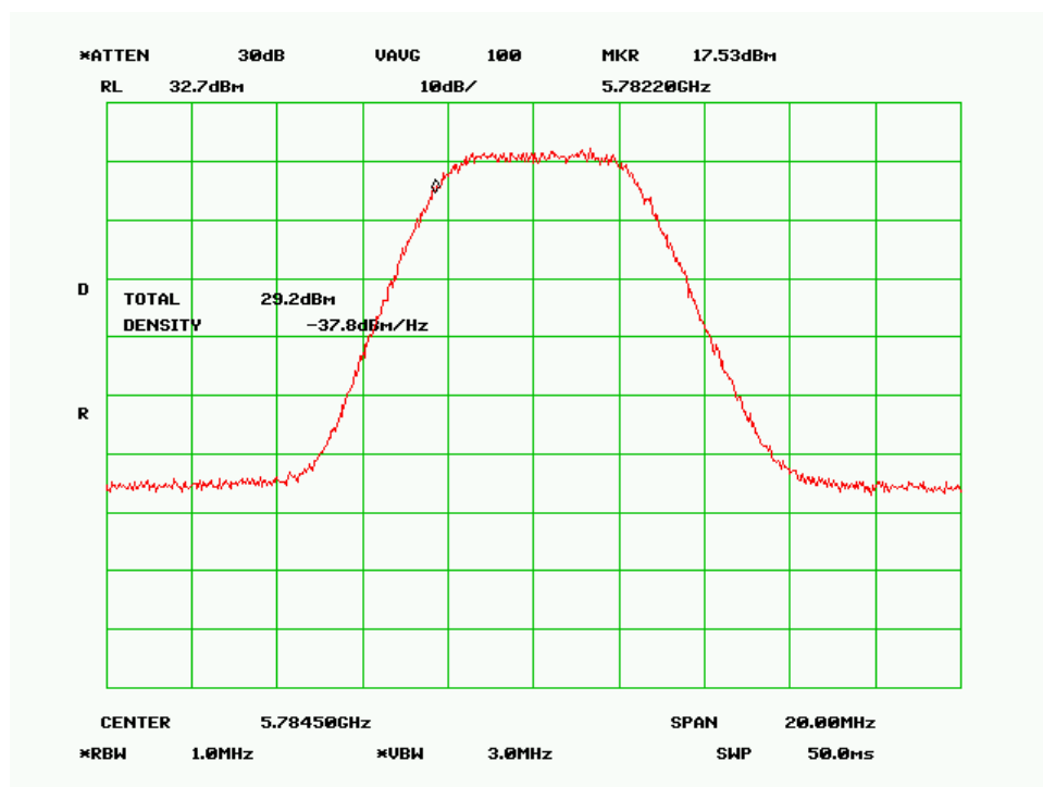
Mid Channel (5MHz QPSK Mode)
