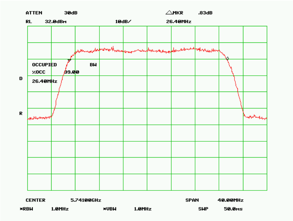
99% Bandwidth – Low Channel (30MHz 256QAM Mode)
