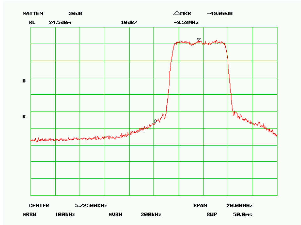
Low Channel-5MHz, QPSK
