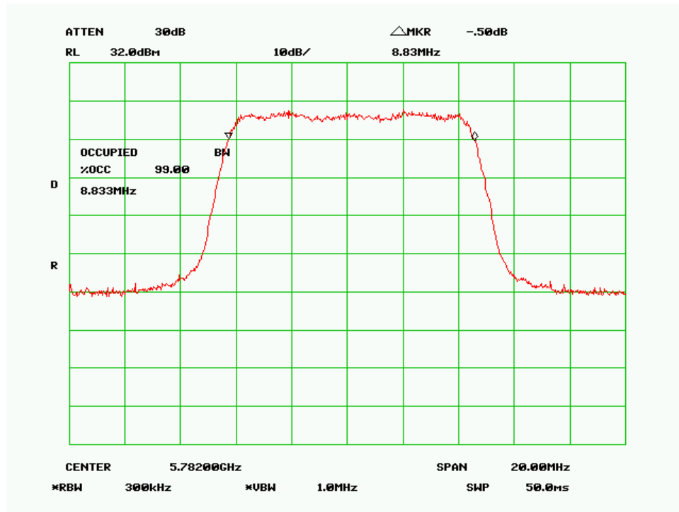
99% Bandwidth – Mid Channel (10MHz QPSK Mode)
