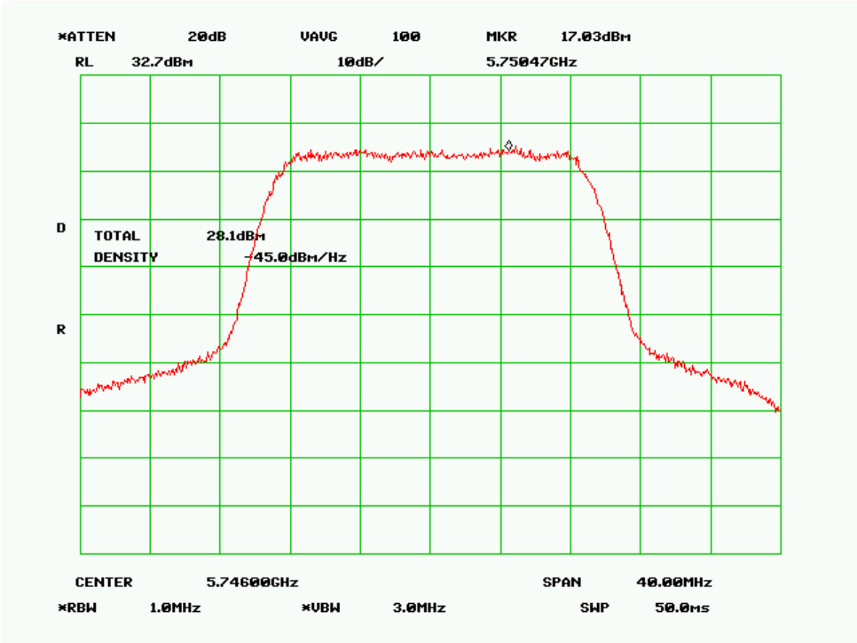
Low Channel (20MHz 256QAM Mode)
