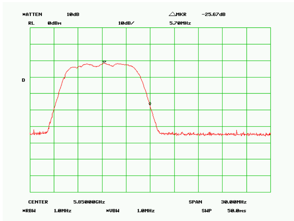
High Channel-10MHz, 256QAM, Vertical Polarity
