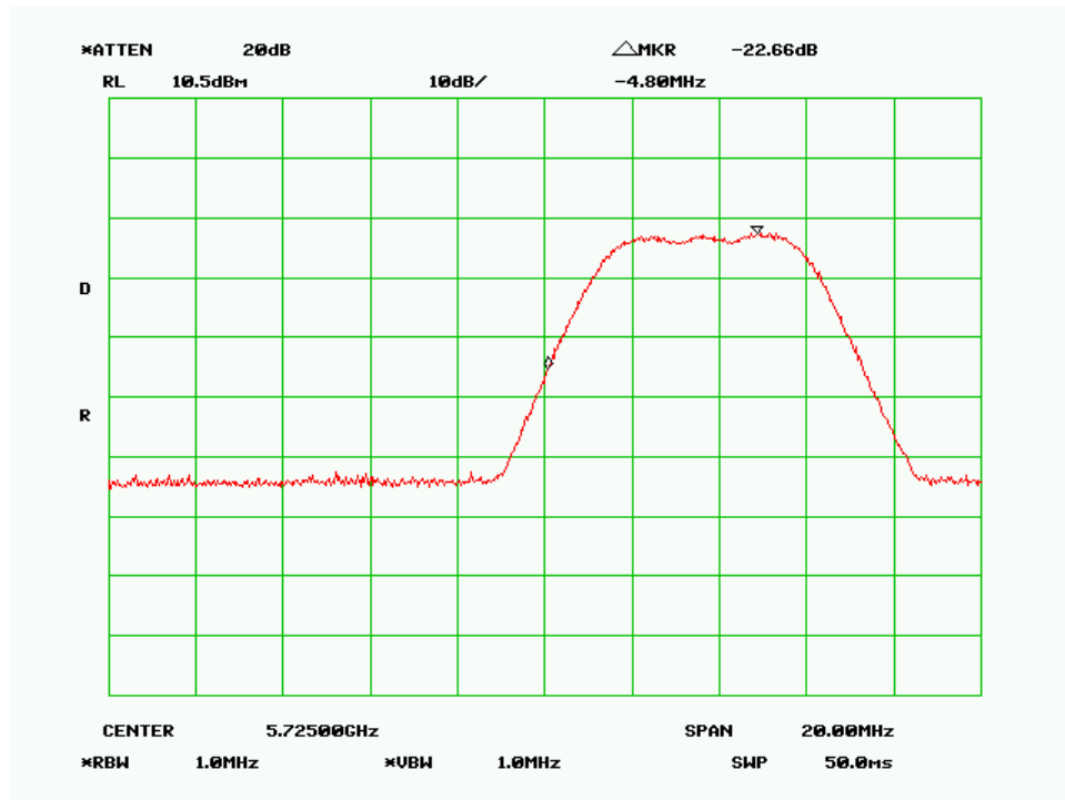
Low Channel-5MHz, 256QAM, Horizontal Polarity
