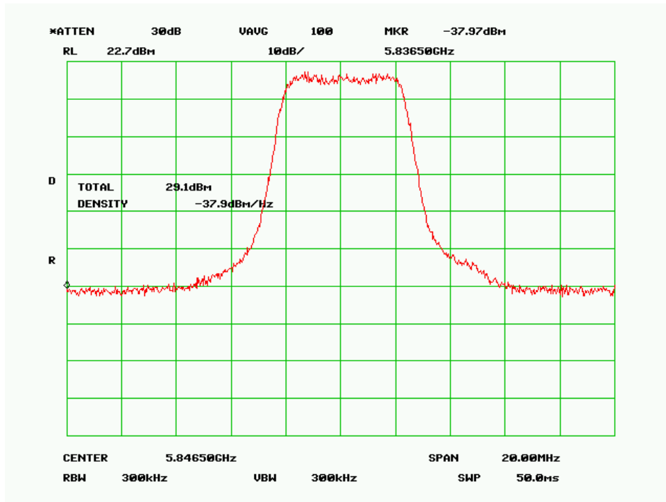
High Channel (5MHz 256QAM Mode)
