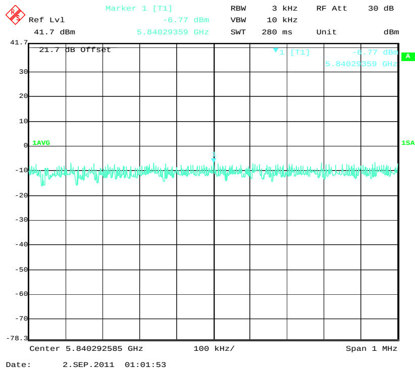
High Channel (30MHz QPSK Mode)
