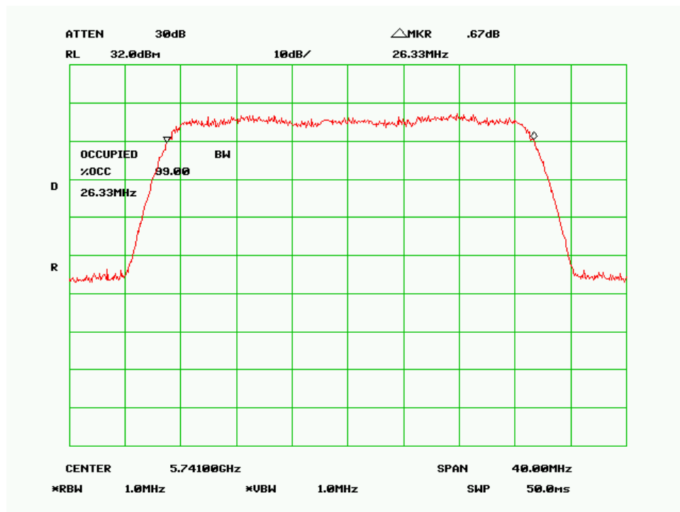
99% Bandwidth – Low Channel (30MHz QPSK Mode)
