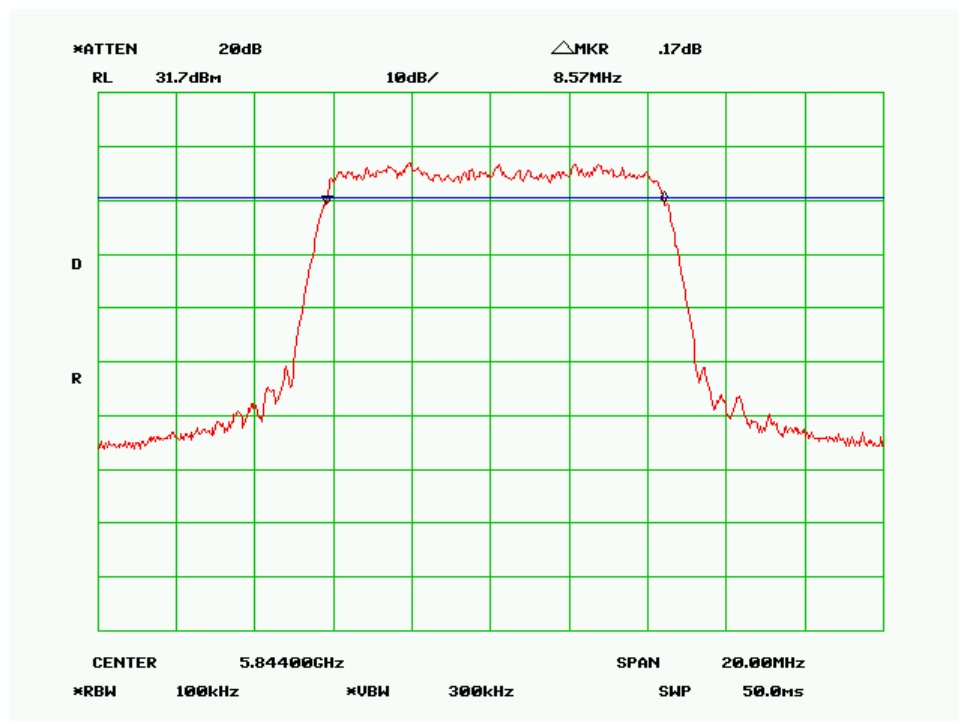
6 dB Bandwidth – High Channel (10MHz 256QAM Mode)
