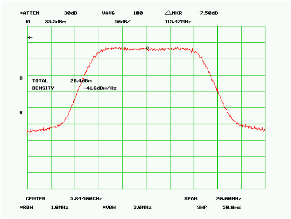
High Channel (10MHz 256QAM Mode)
