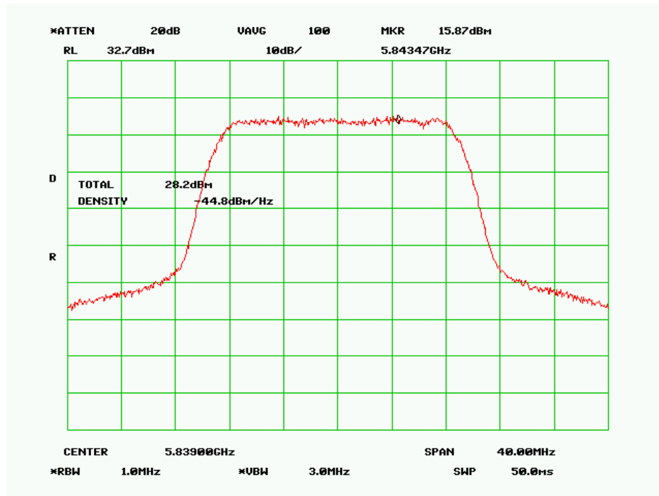
High Channel (20MHz 256QAM Mode)
