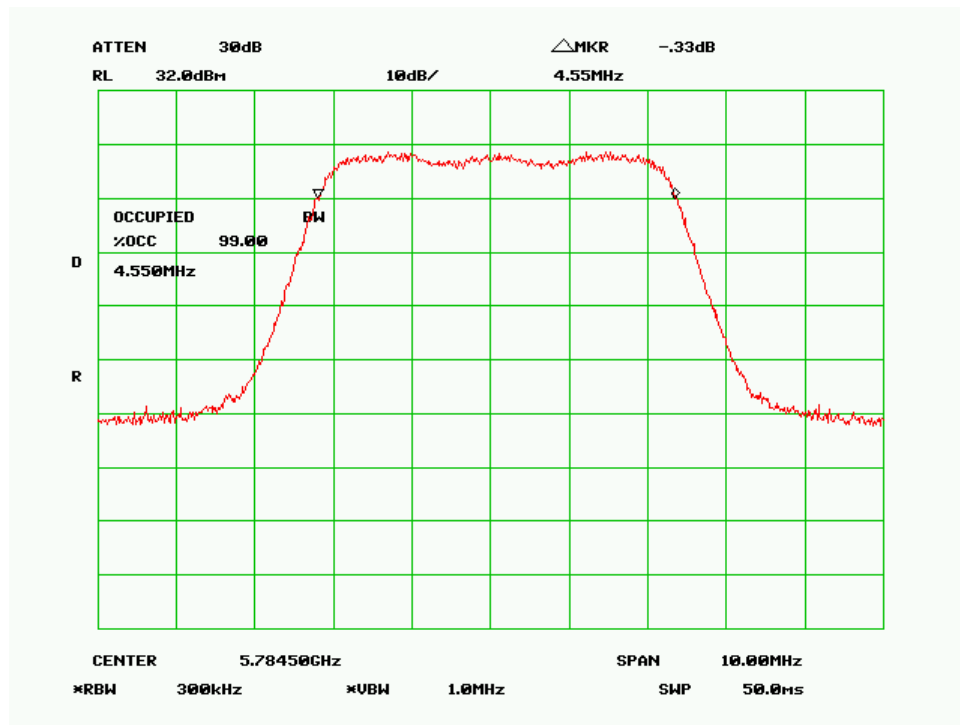
99% Bandwidth - Mid Channel (5MHz QPSK Mode)
