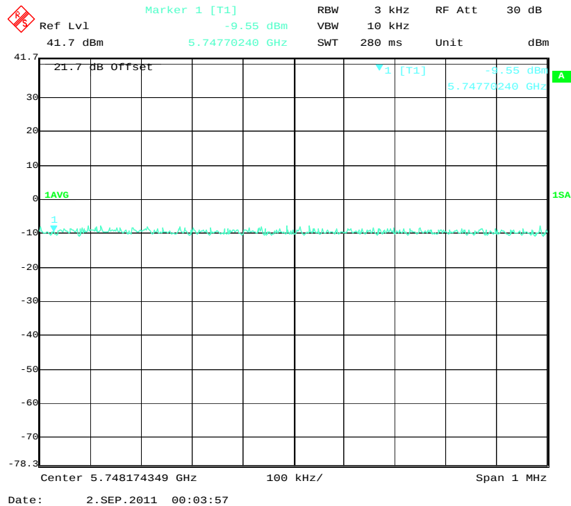
Low Channel (30MHz 256QAM Mode)
