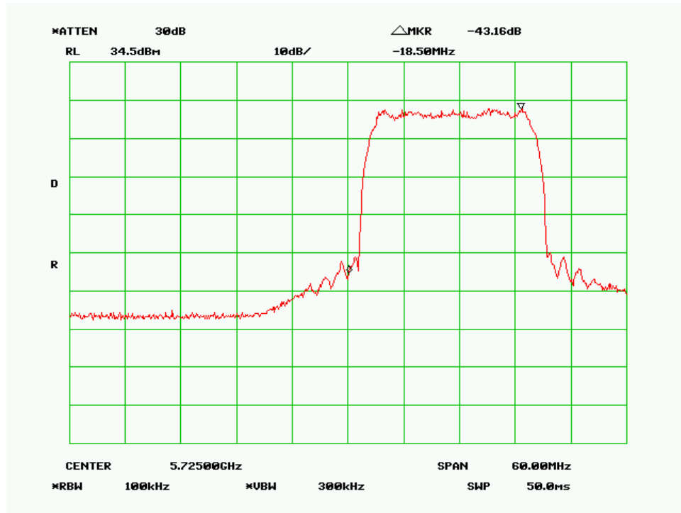
Low Channel-20MHz, QPSK
