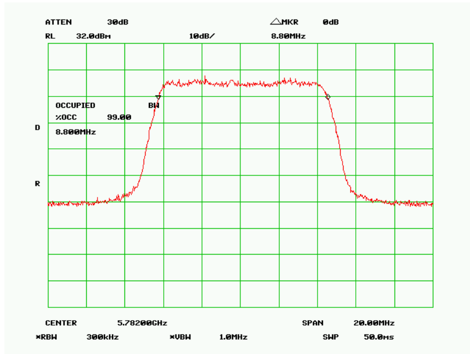
99% Bandwidth – Mid Channel (10MHz 256QAM Mode)
