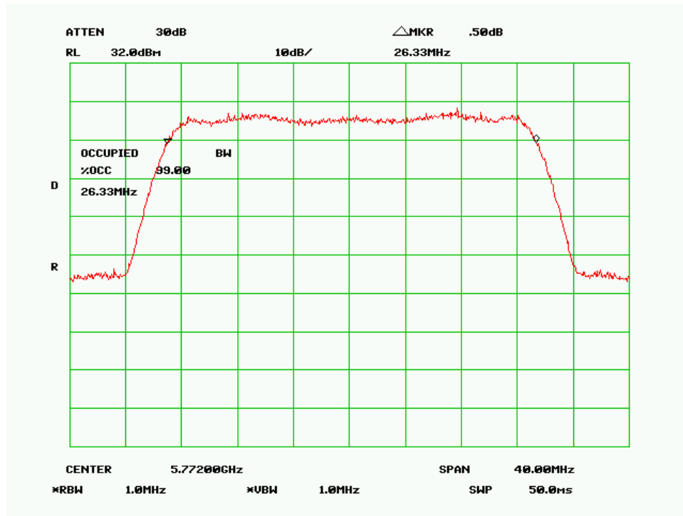
99% Bandwidth – Mid Channel (30MHz QPSK Mode)
