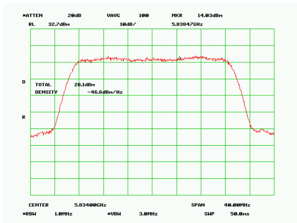
High Channel (30MHz 256QAM Mode)
