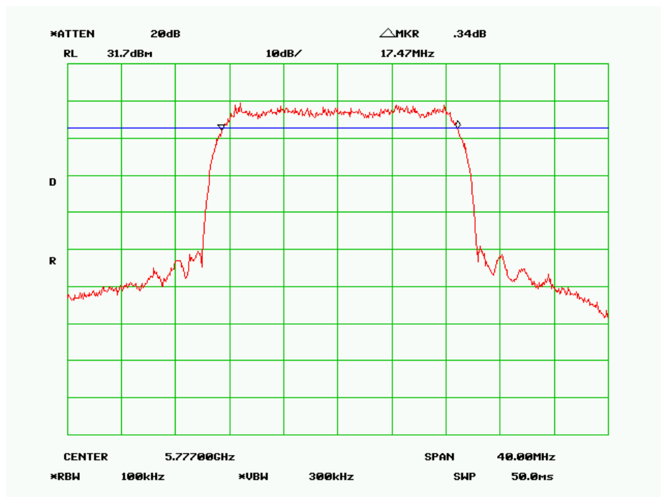
6 dB Bandwidth – Mid Channel (20MHz QPSK Mode)
