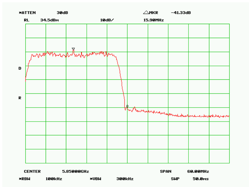
High Channel-30MHz, QPSK
