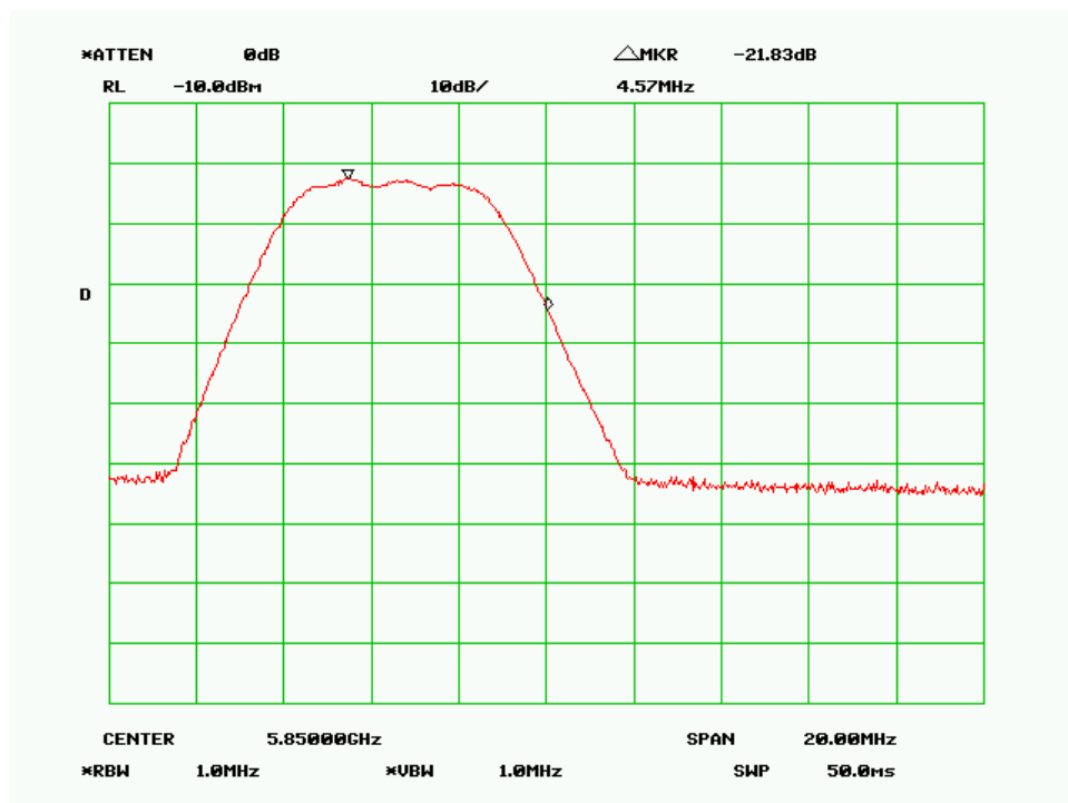
High Channel-5MHz, 256QAM, Vertical Polarity
