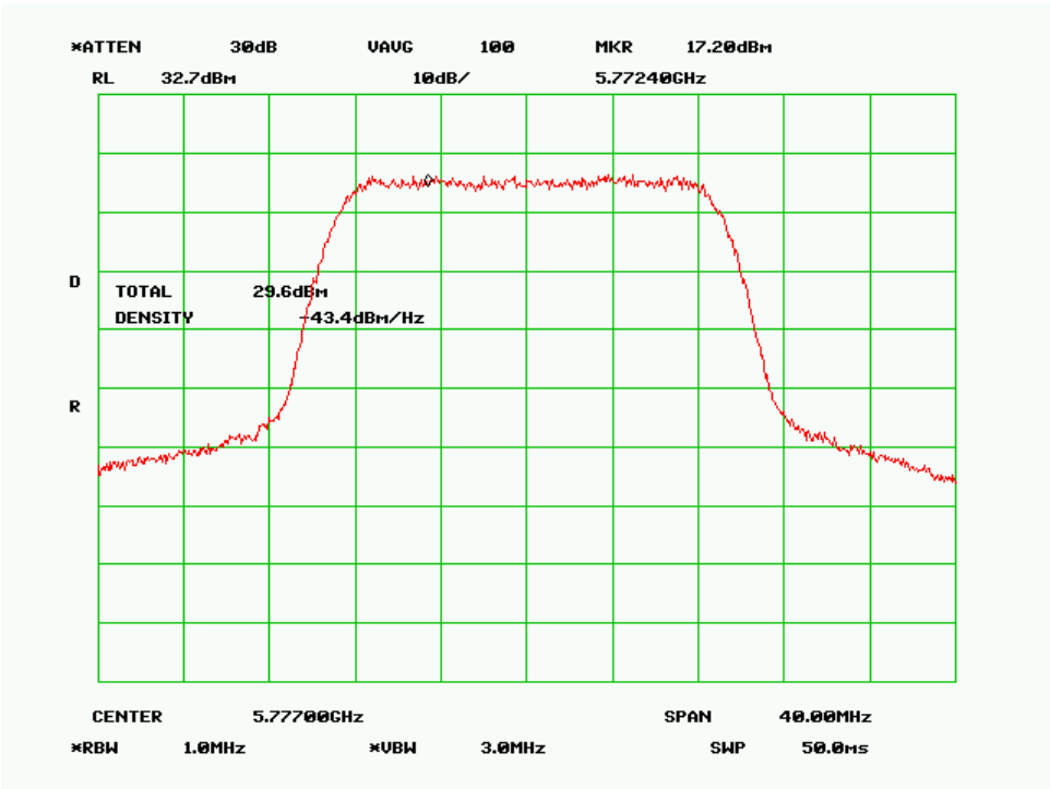
Mid Channel (20MHz QPSK Mode)
