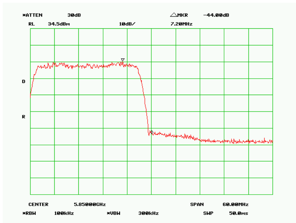
High Channel-30MHz, 256QAM
