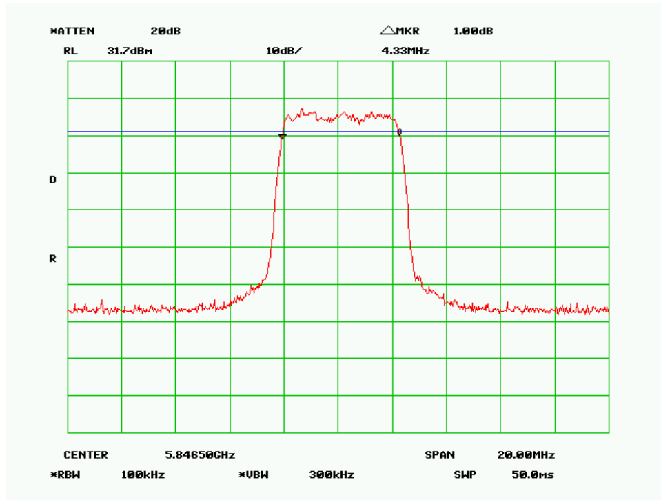
6 dB Bandwidth – High Channel (5MHz 256QAM Mode)
