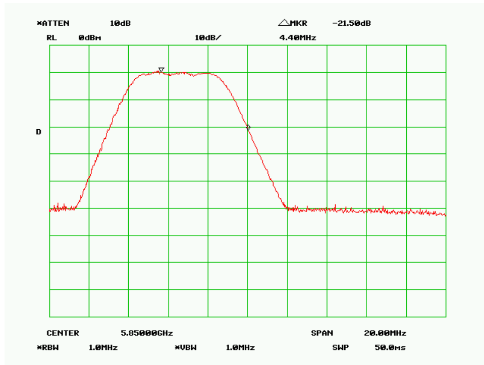
High Channel-5MHz, 256QAM, Horizontal Polarity
