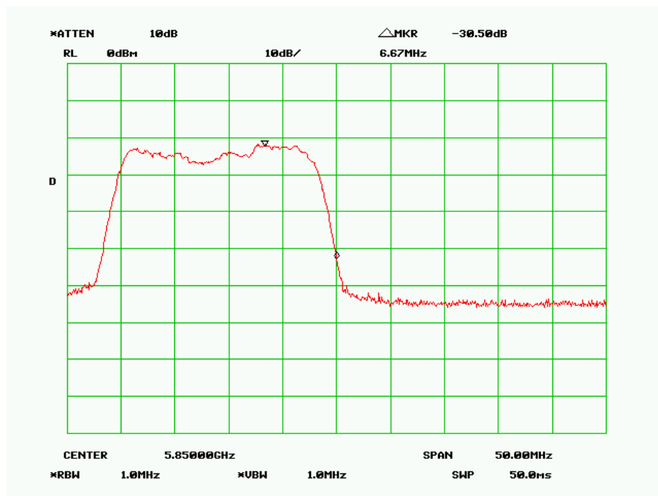
High Channel-20MHz, 256QAM, Vertical Polarity
