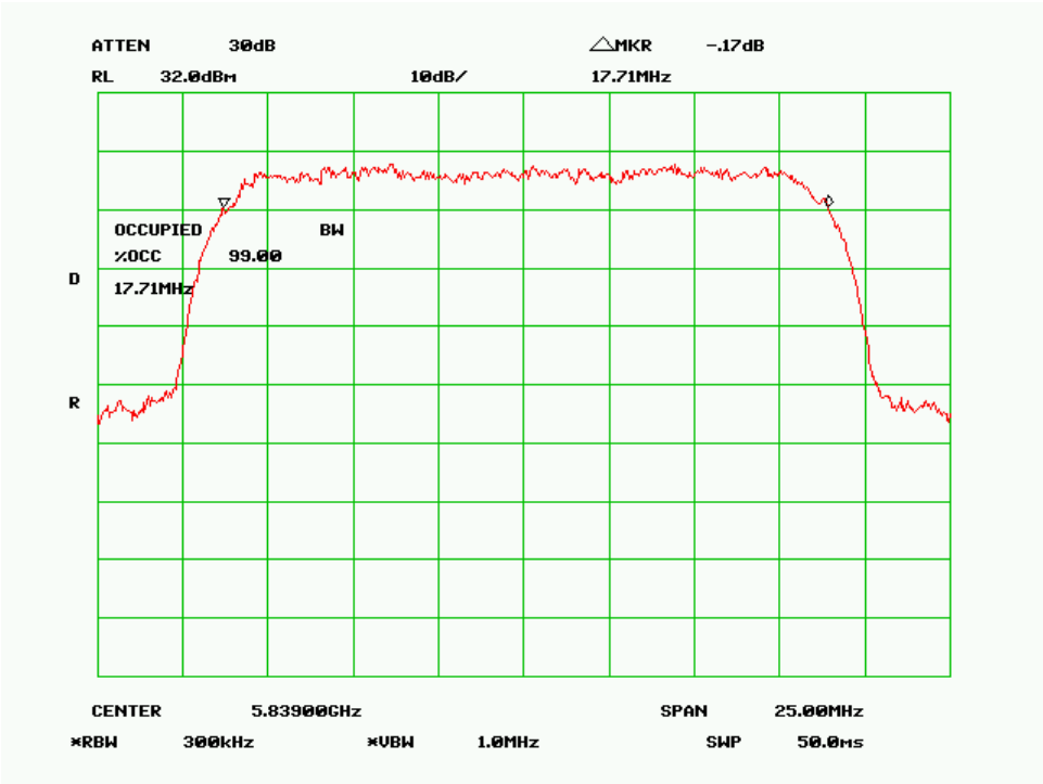
99% Bandwidth – High Channel (20MHz 256QAM Mode)
