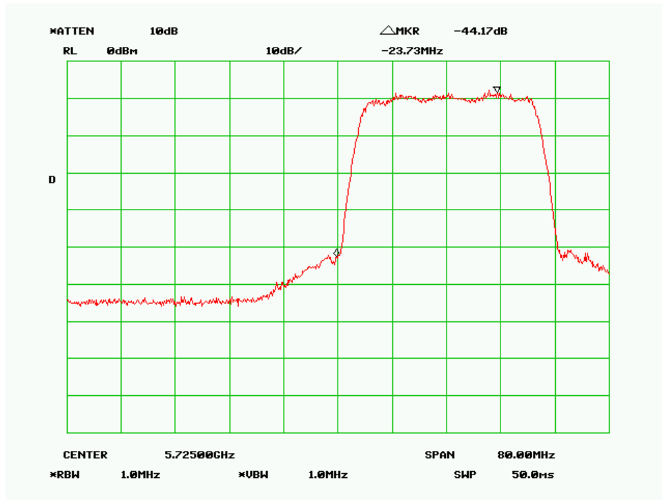
Low Channel-30MHz, 256QAM, Horizontal Polarity
