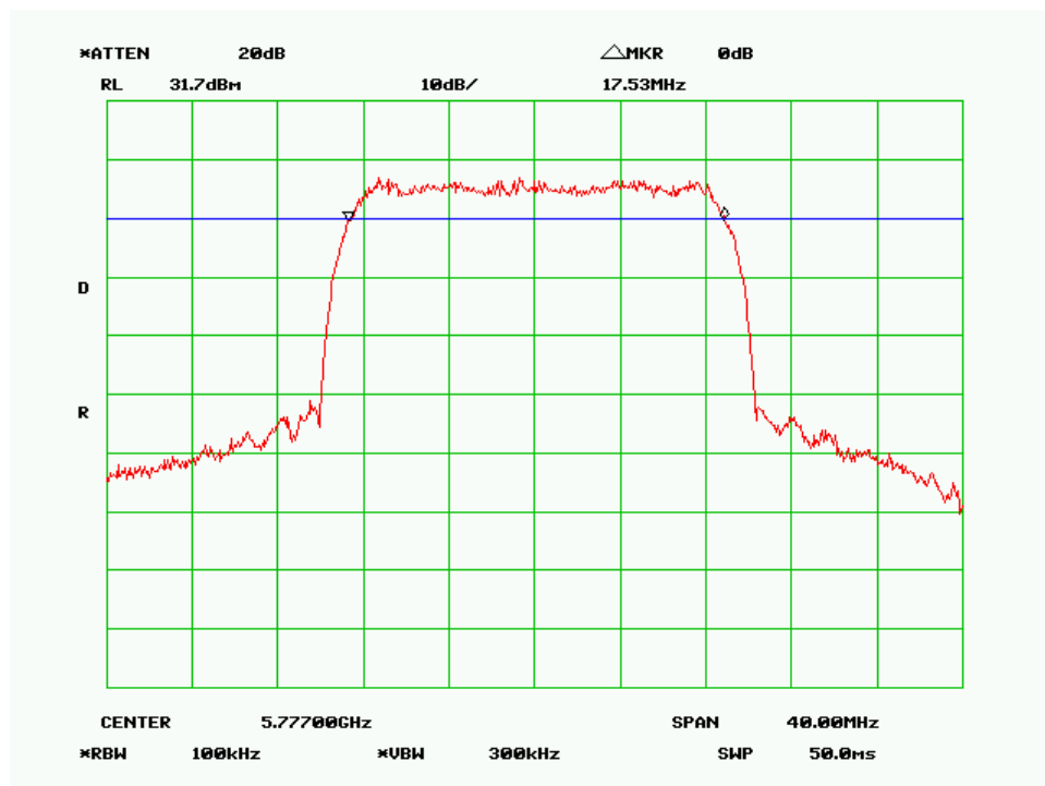
6 dB Bandwidth – Mid Channel (20MHz 256QAM Mode)
