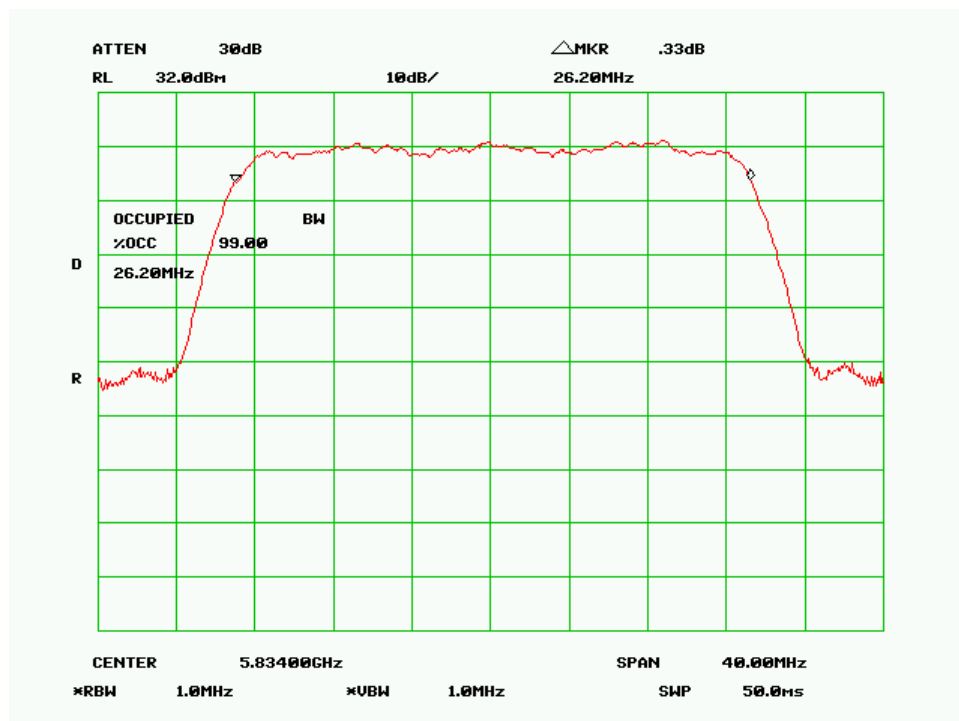
99% Bandwidth – High Channel (30MHz QPSK Mode)
