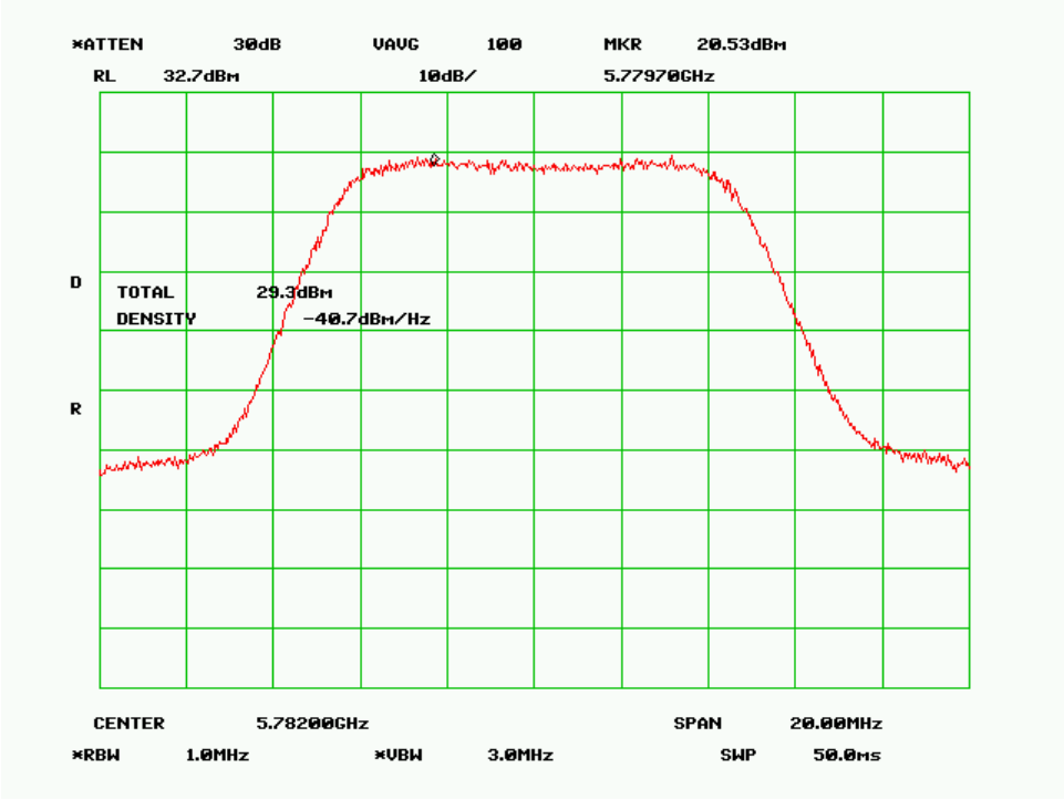
Mid Channel (10MHz QPSK Mode)
