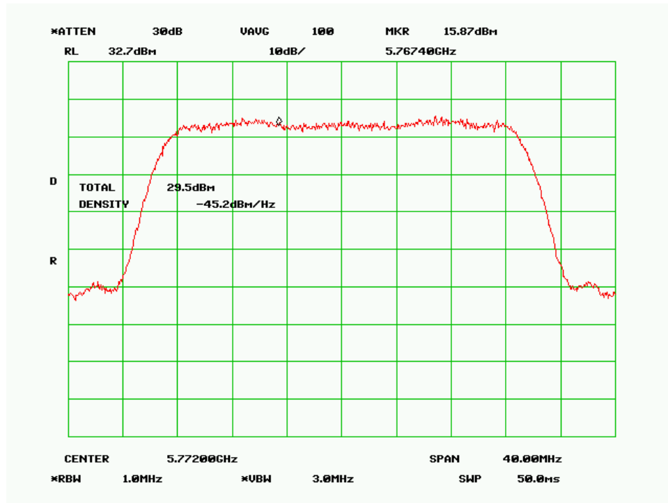
Mid Channel (30MHz QPSK Mode)
