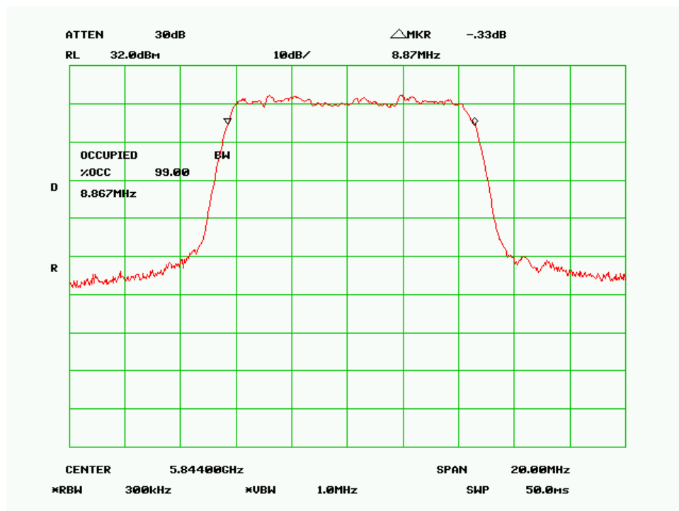
99% Bandwidth – High Channel (10MHz 256QAM Mode)
