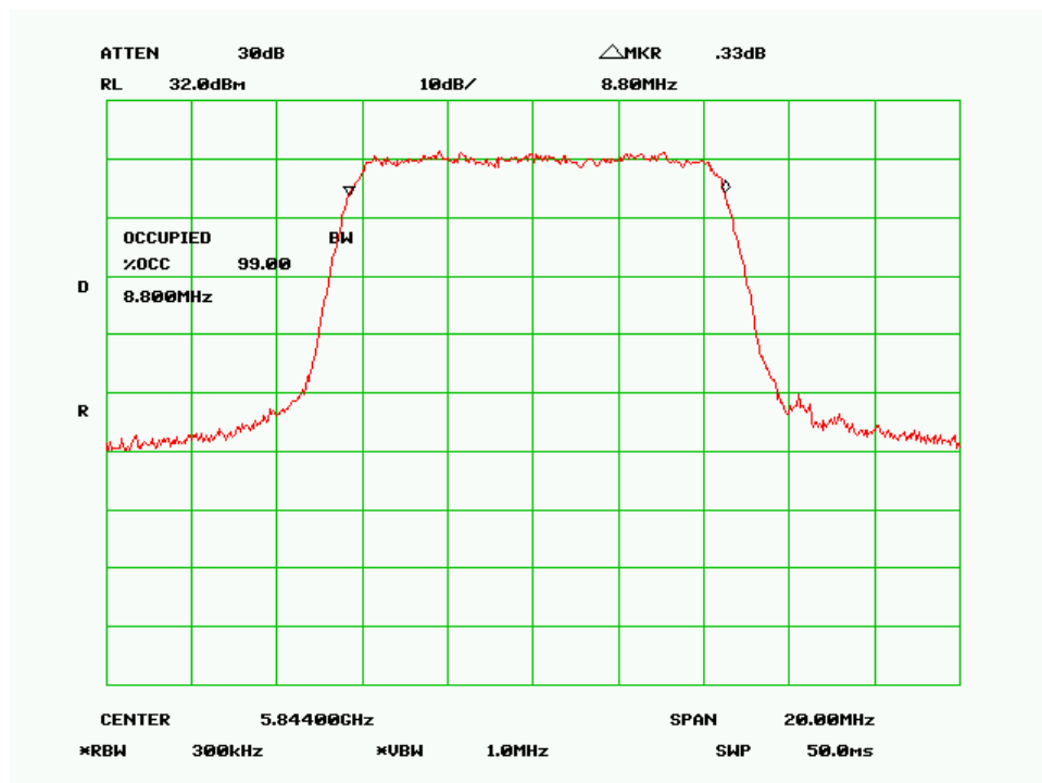
99% Bandwidth – High Channel (10MHz QPSK Mode)
