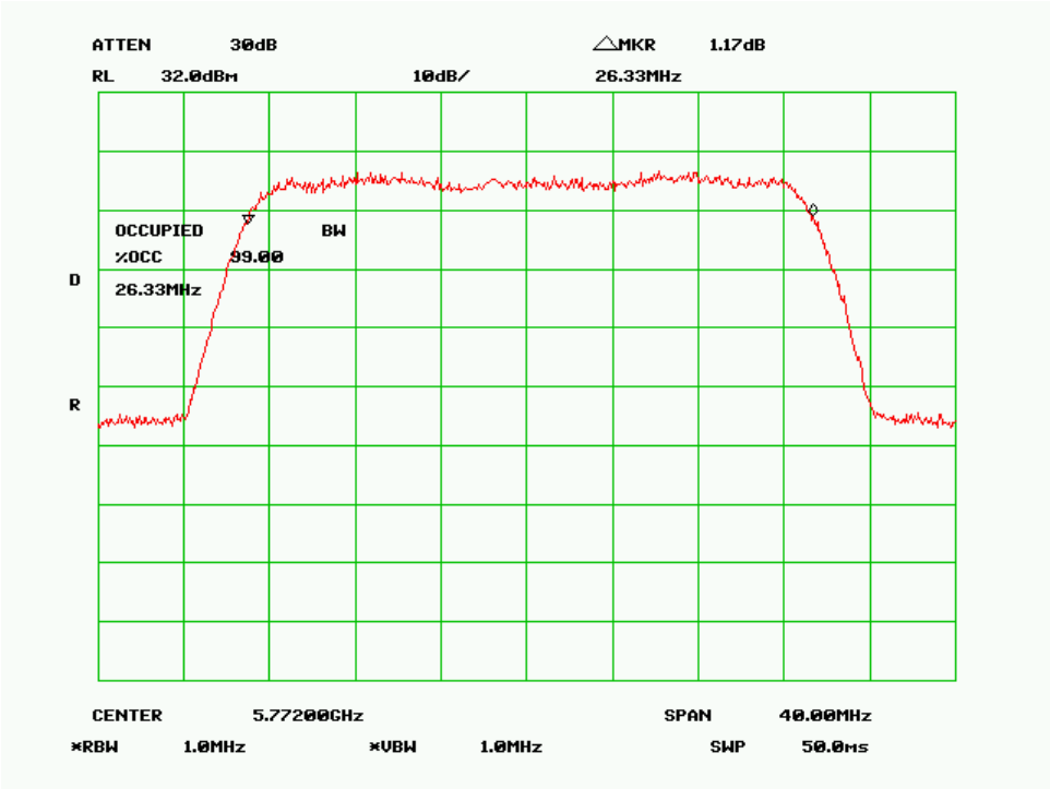
99% Bandwidth – Mid Channel (30MHz 256QAM Mode)
