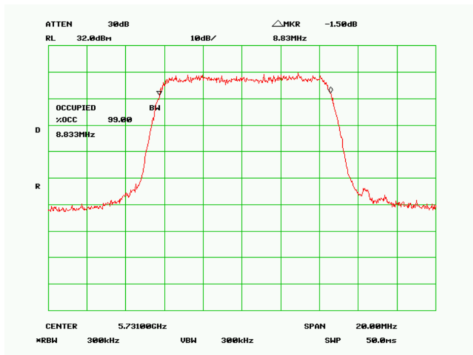
99% Bandwidth – Low Channel (10MHz QPSK Mode)
