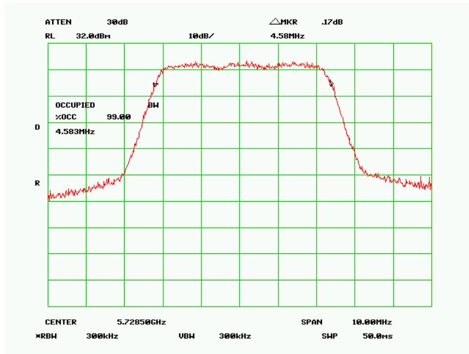
99% Bandwidth - Low Channel (5MHz 256QAM Mode)
