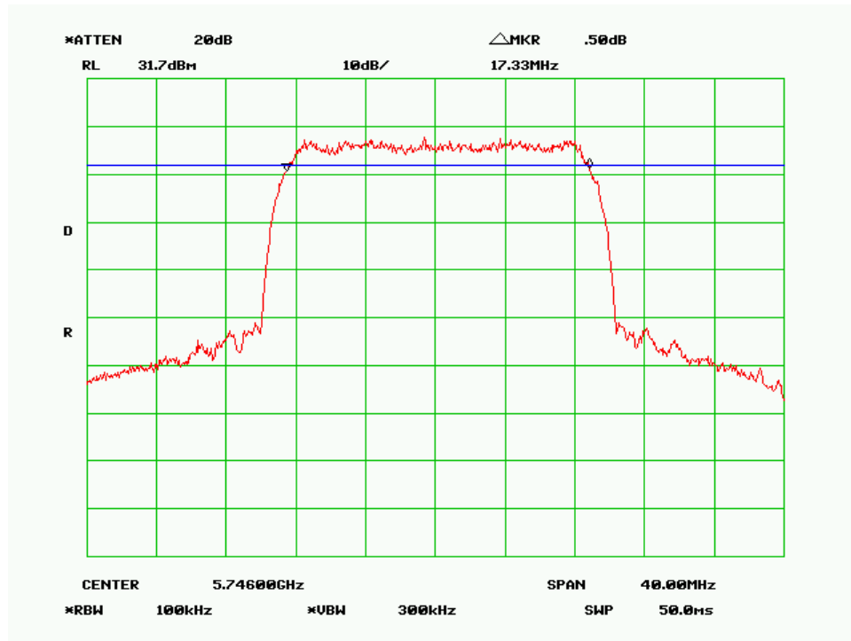
6 dB Bandwidth – Low Channel (20MHz 256QAM Mode)
