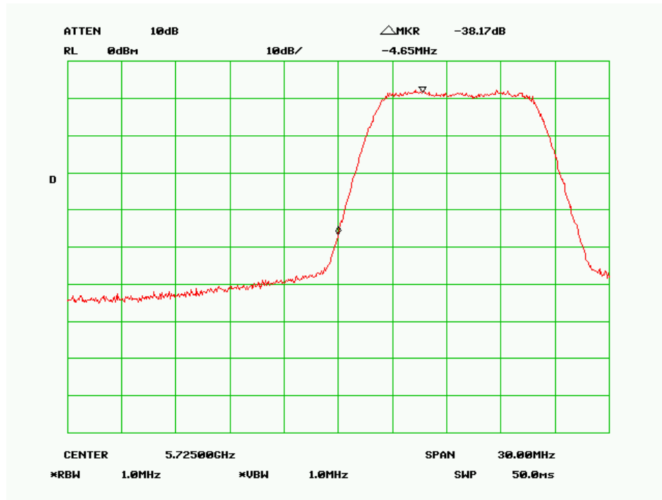
Low Channel-10MHz, 256QAM, Horizontal Polarity
