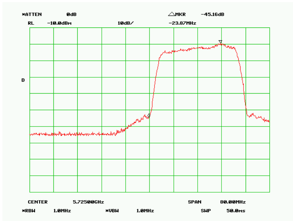
Low Channel-30MHz, 256QAM, Vertical Polarity
