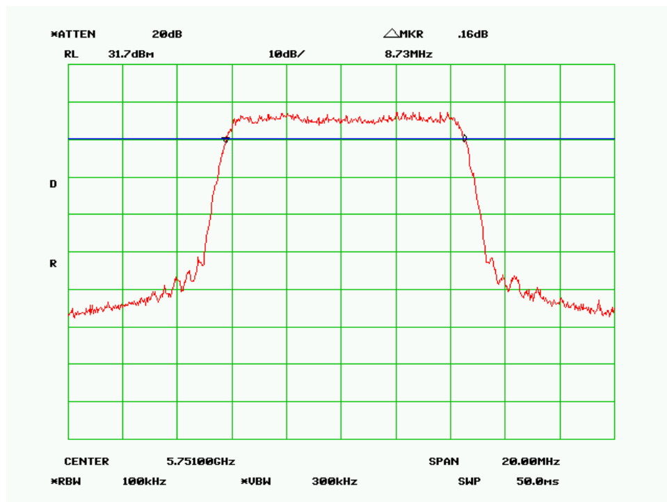
6 dB Bandwidth – Low Channel (10MHz 256QAM Mode)
