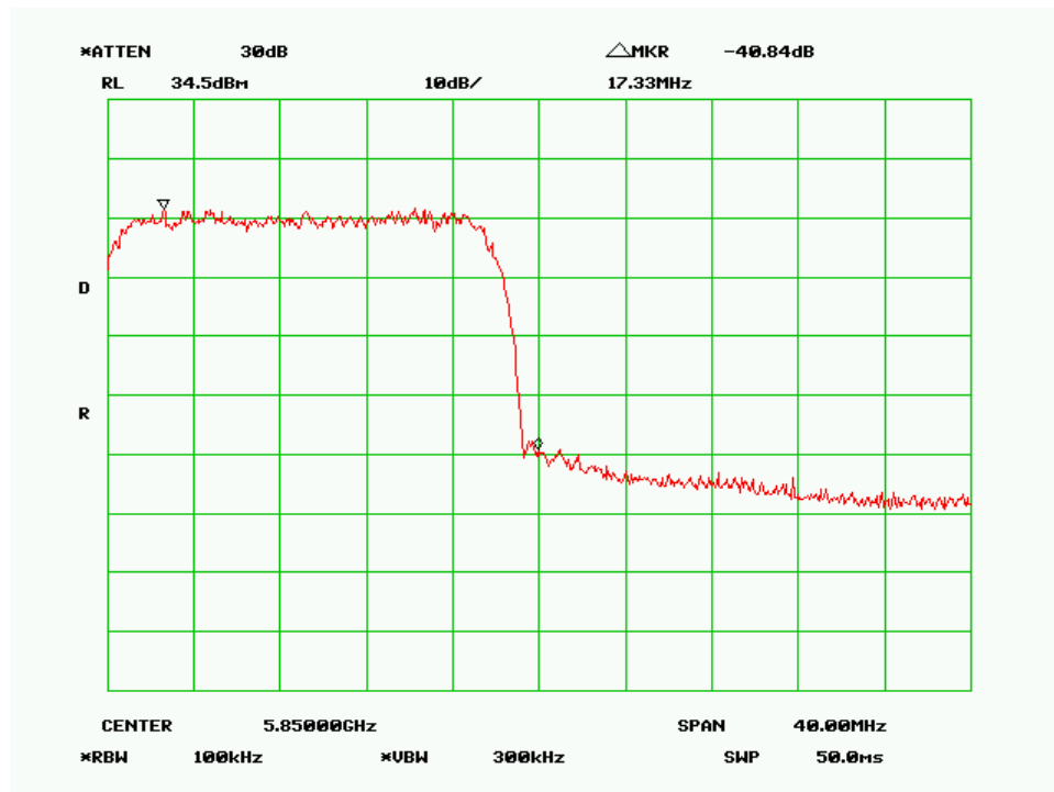
High Channel-20MHz, 256QAM
