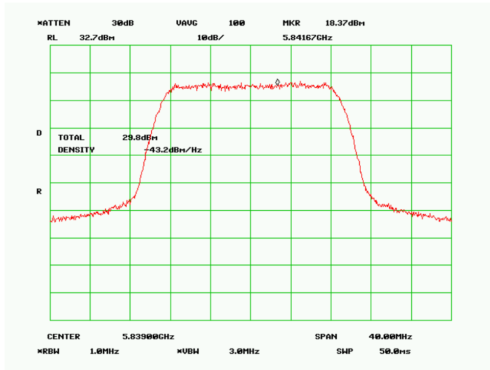
High Channel (20MHz QPSK Mode)
