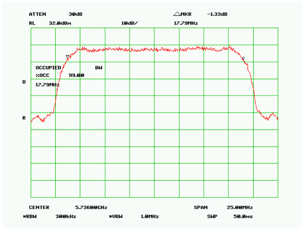
99% Bandwidth - Low Channel (20MHz QPSK Mode)
