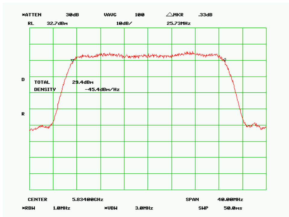
High Channel (30MHz QPSK Mode)
