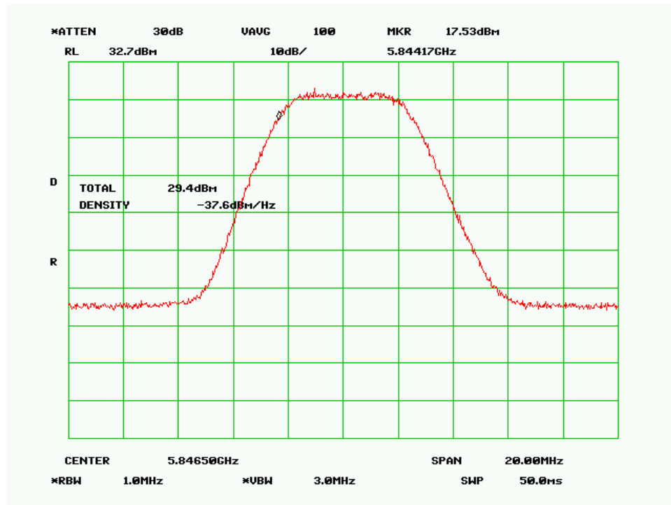
High Channel (5MHz QPSK Mode)
