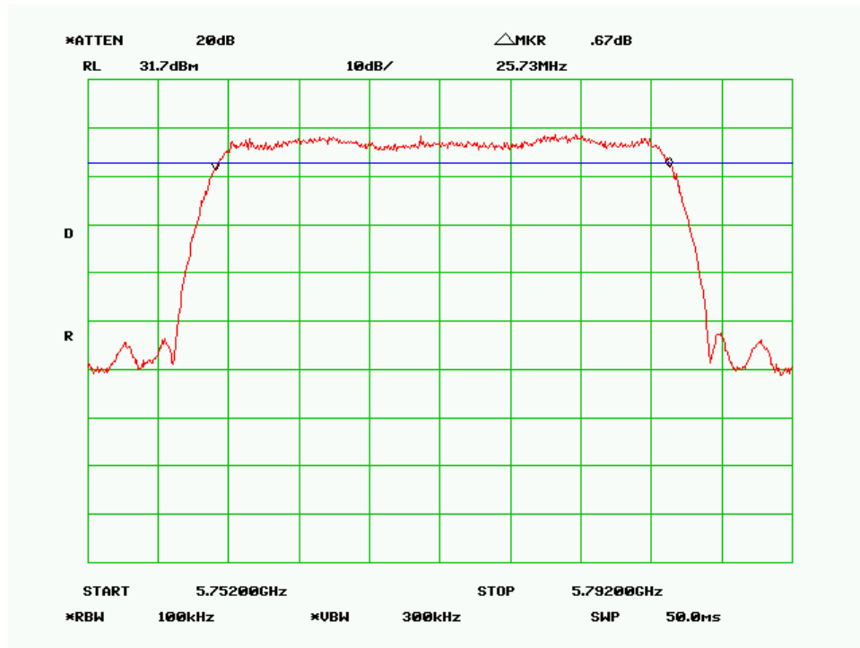
6dB Bandwidth – Mid Channel (30MHz QPSK Mode)
