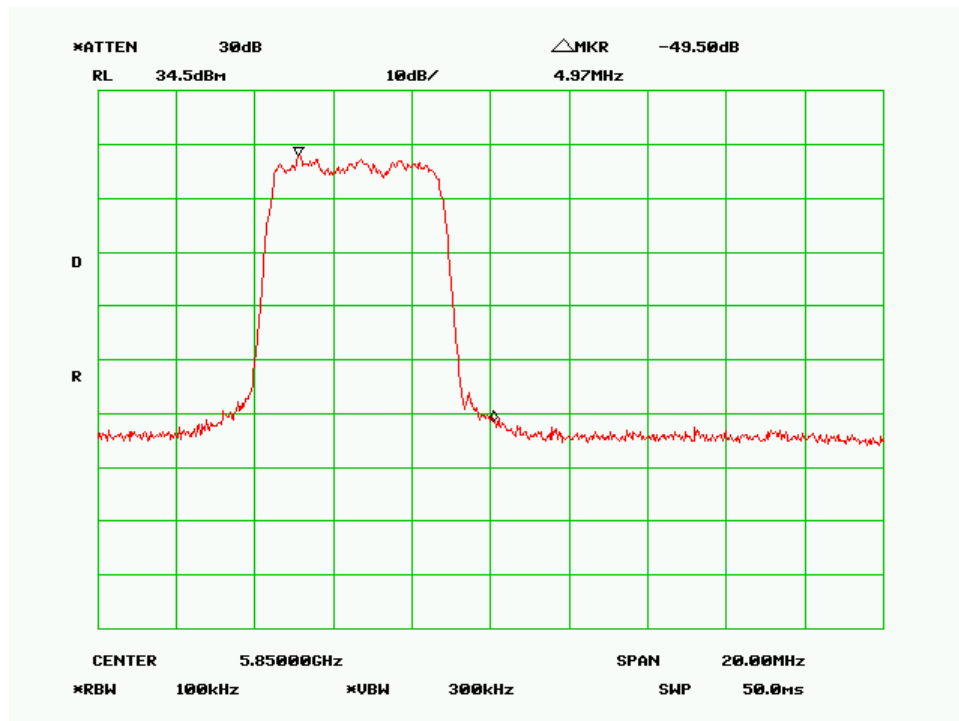
High Channel-5MHz, 256QAM
