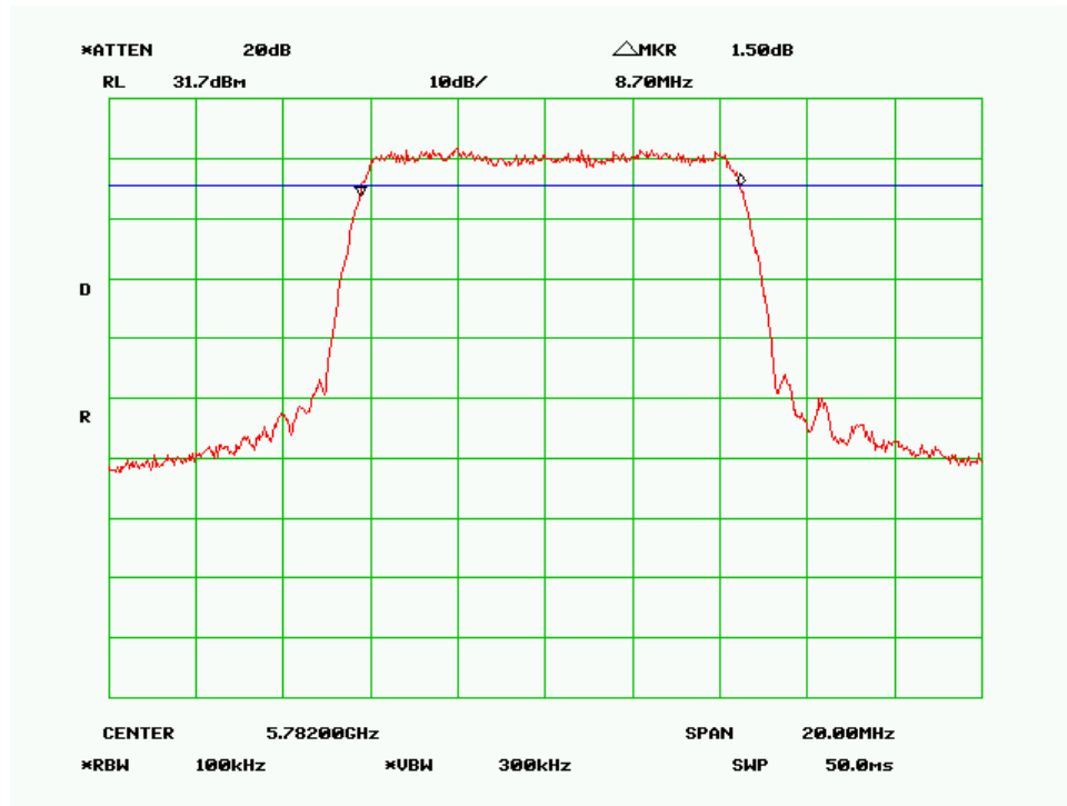
6 dB Bandwidth – Mid Channel (10MHz QPSK Mode)
