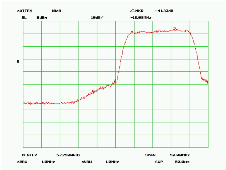
Low Channel-20MHz, 256QAM, Horizontal Polarity
