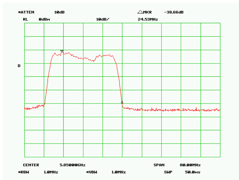
High Channel-30MHz, 256QAM, Vertical Polarity
