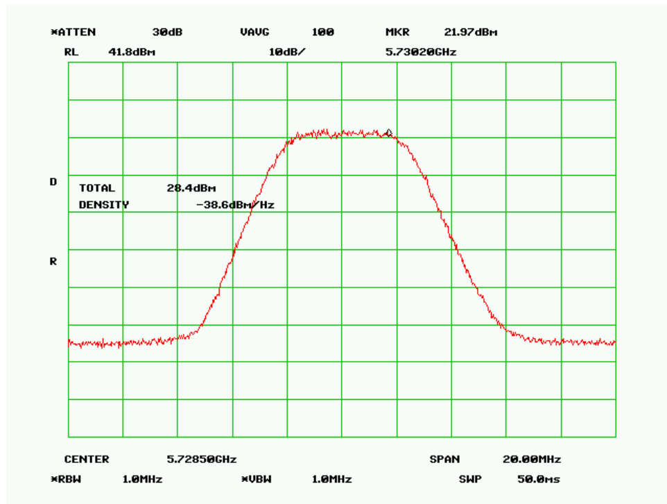
Low Channel (5MHz 256QAM Mode)
