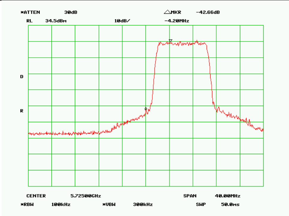
Low Channel-10MHz, 256QAM
