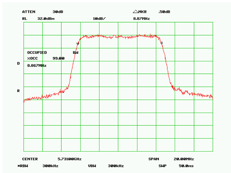
99% Bandwidth – Low Channel (10MHz 256QAM Mode)
