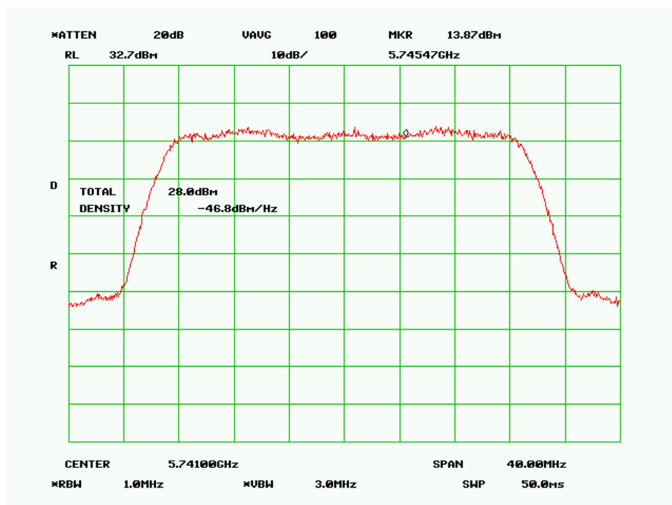
Low Channel (30MHz 256QAM Mode)
