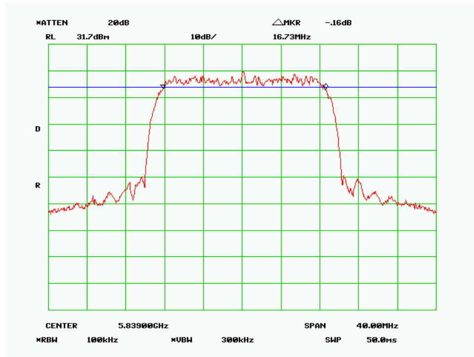
6dB Bandwidth – High Channel (20MHz QPSK Mode)
