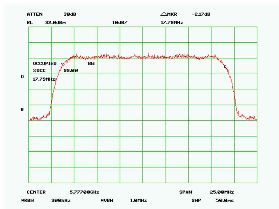
99% Bandwidth – Mid Channel (20MHz 256QAM Mode)
