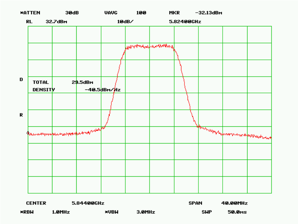
High Channel (10MHz QPSK Mode)
