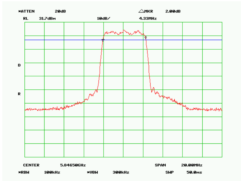
6 dB Bandwidth – High Channel (5MHz QPSK Mode)
