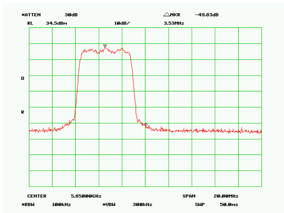
High Channel-5MHz, QPSK
