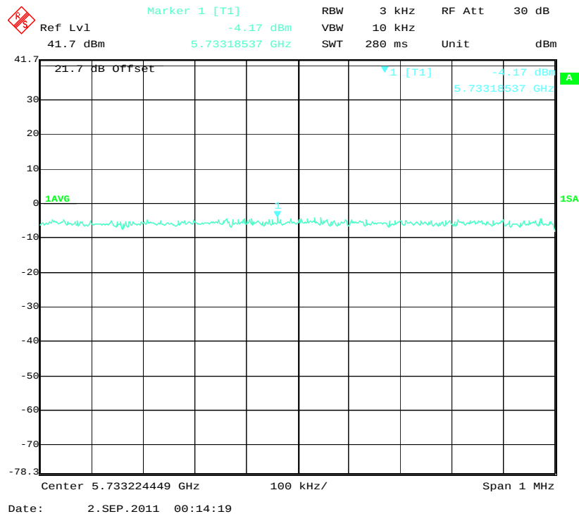
Low Channel (10MHz 256QAM Mode)
