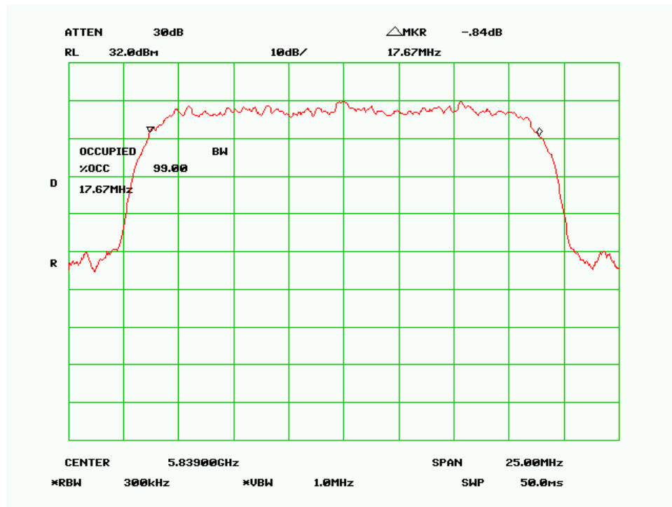
99% Bandwidth – High Channel (20MHz QPSK Mode)
