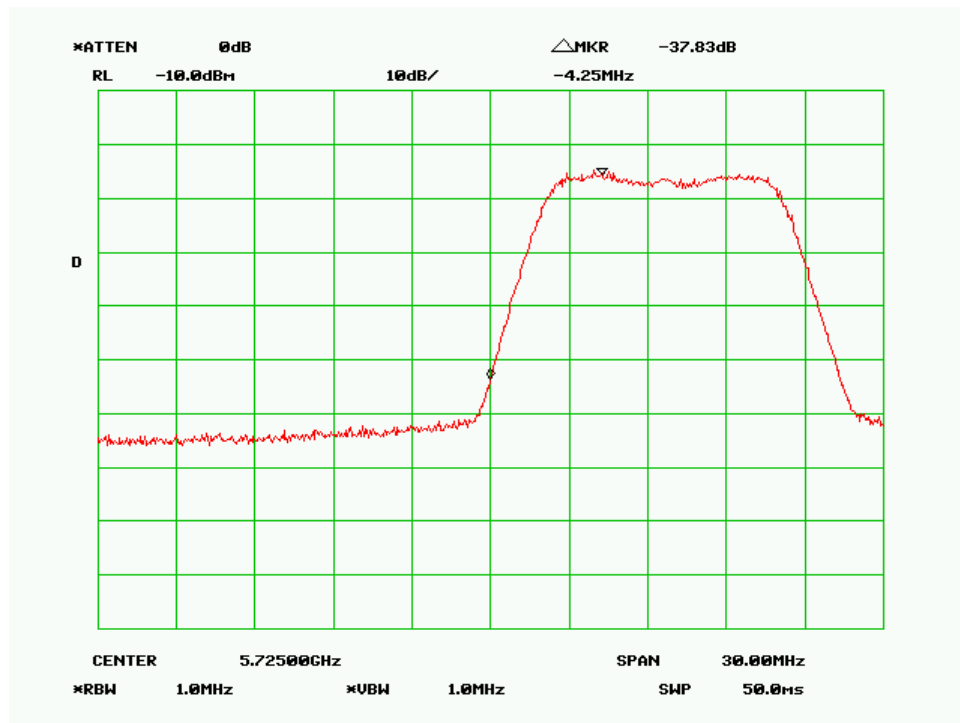
Low Channel-10MHz, 256QAM, Vertical Polarity
