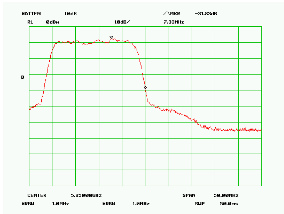
High Channel-20MHz, 256QAM, Horizontal Polarity
