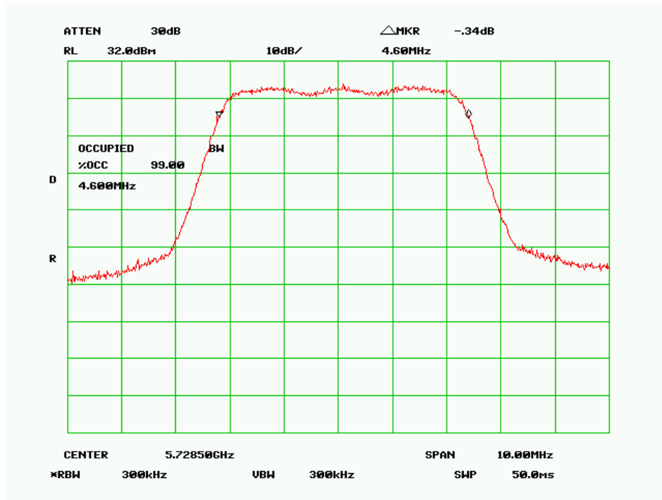
99% Bandwidth - Low Channel (5MHz QPSK Mode)
