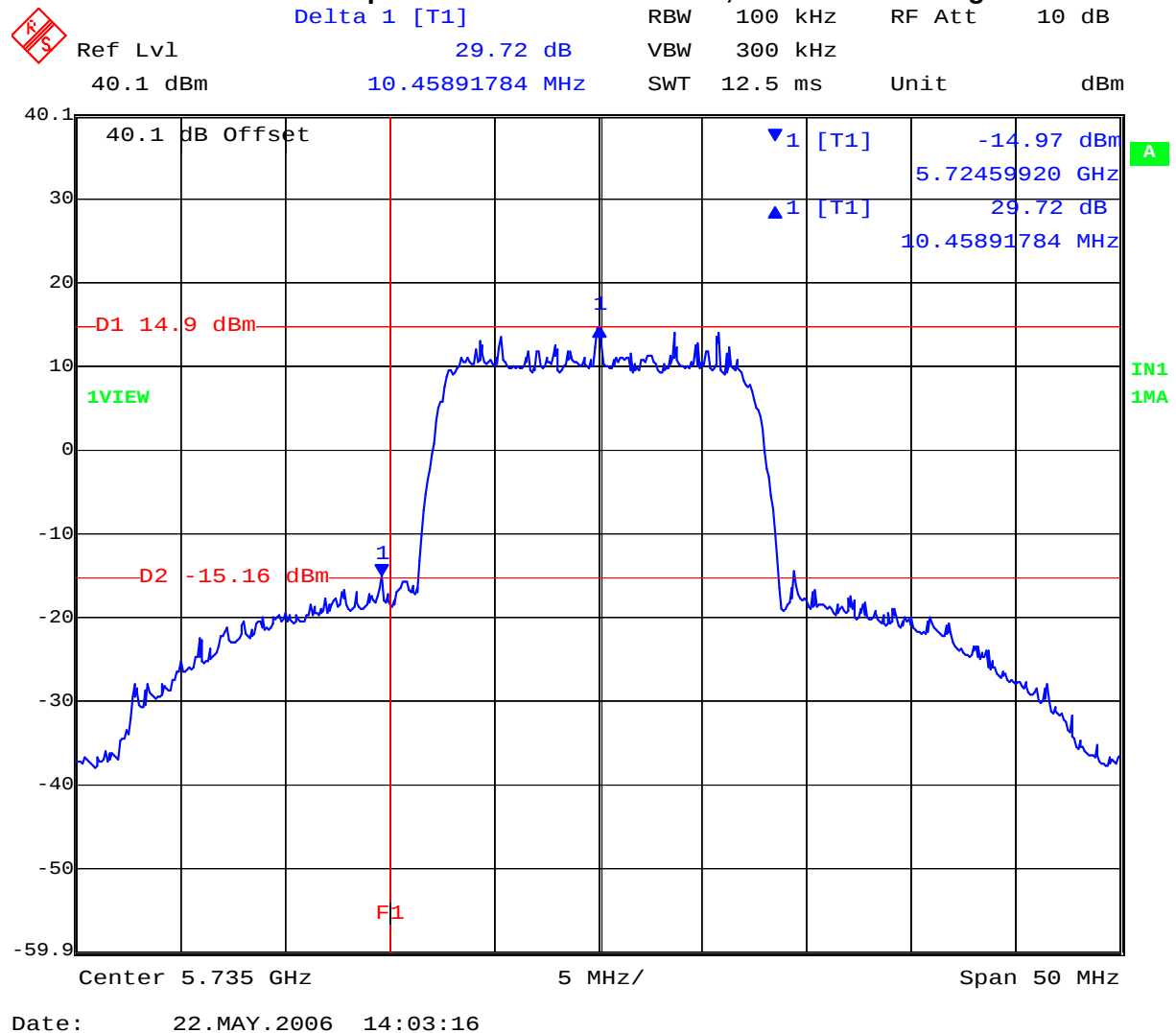
Plot 15 15 MHz Bandwidth QPSK
