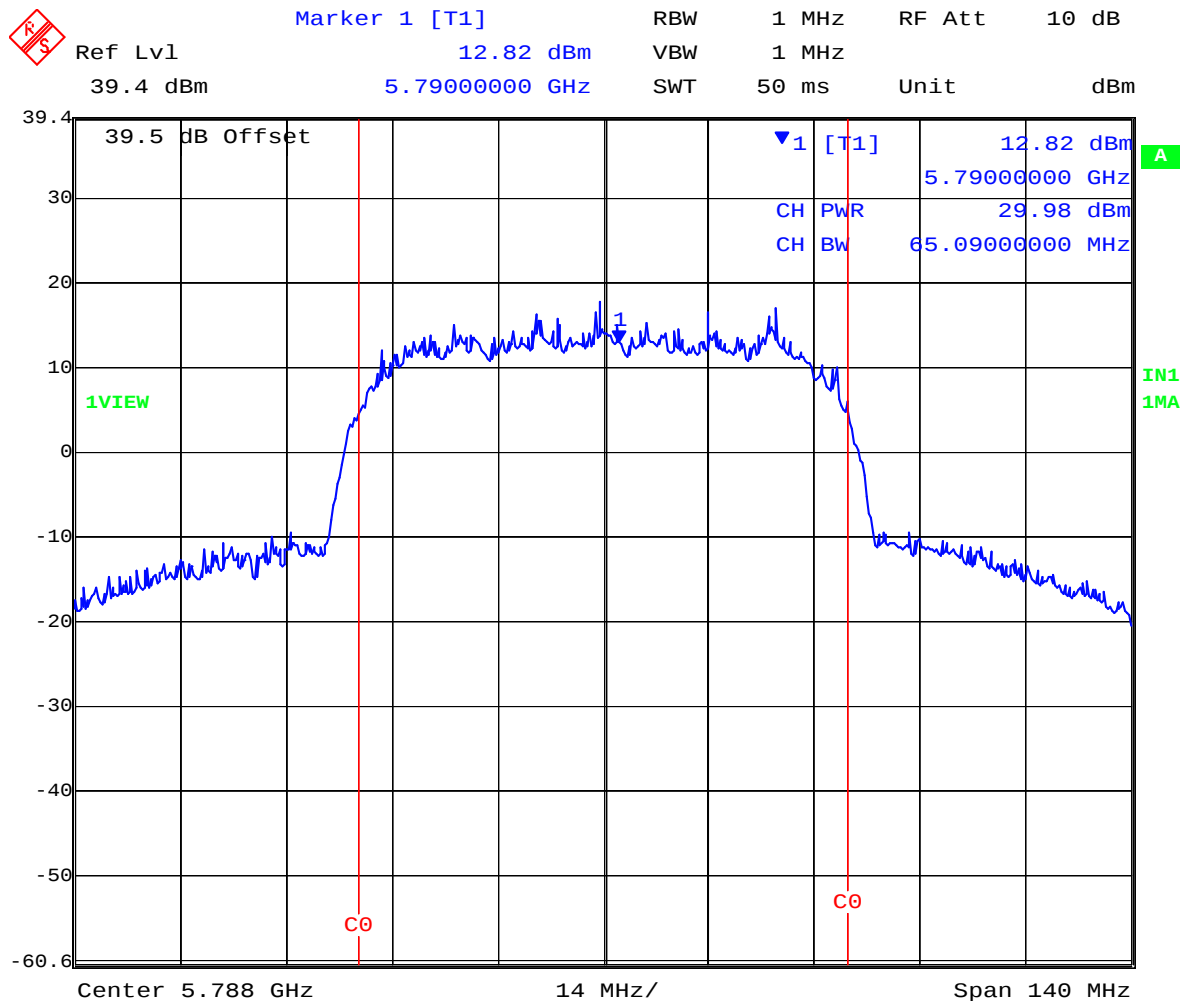
Plot 08 5,788 MHz 60 MHz QPSK Peak Power (dBm)
