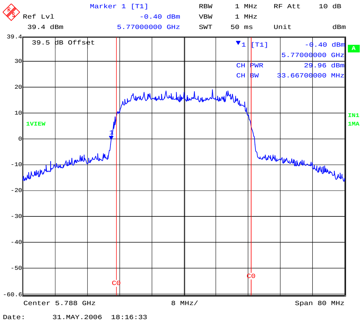
Plot 07 5,788 MHz 30 MHz QPSK Peak Power (dBm)
