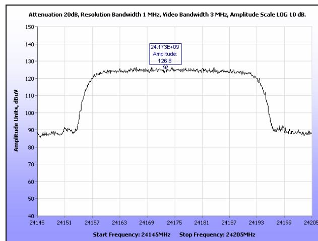
Plot 19. Radiated Field Strength of Fundamental, 40 MHz, Mid Channel
