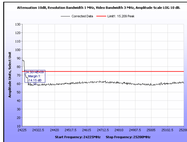
Plot 208. Radiated Band Edge, 25 MHz, High Channel, Peak
