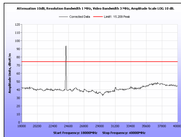
Plot 164. Radiated Spurious Emissions, 40 MHz, Low Channel, 18 GHz - 40 GHz, Peak
