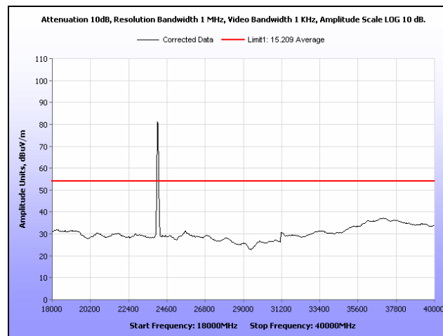
Plot 173. Radiated Spurious Emissions, 50 MHz, Low Channel, 18 GHz - 40 GHz, Average
