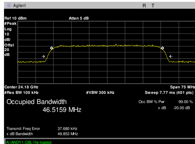
Plot 240. Occupied Bandwidth, Mid Channel, 50 MHz
