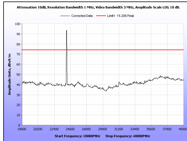
Plot 99. Radiated Spurious Emissions, 25 MHz, Low Channel, 18 GHz - 40 GHz, Peak
