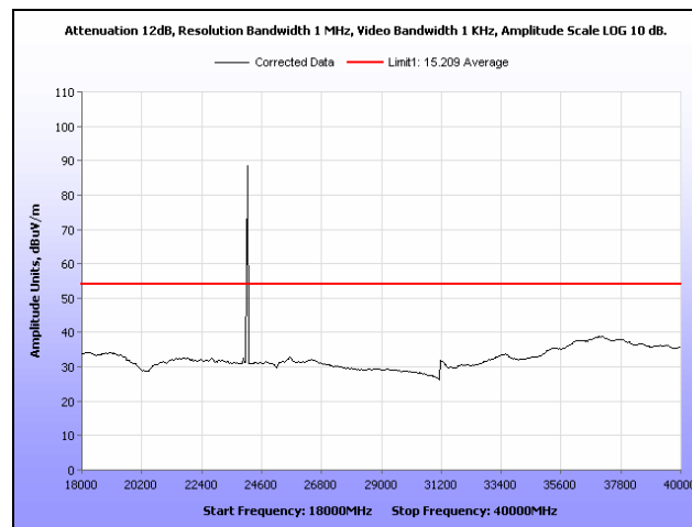
Plot 52. Radiated Spurious Emissions, 10 MHz, Low Channel, 18-40 GHz, Average
