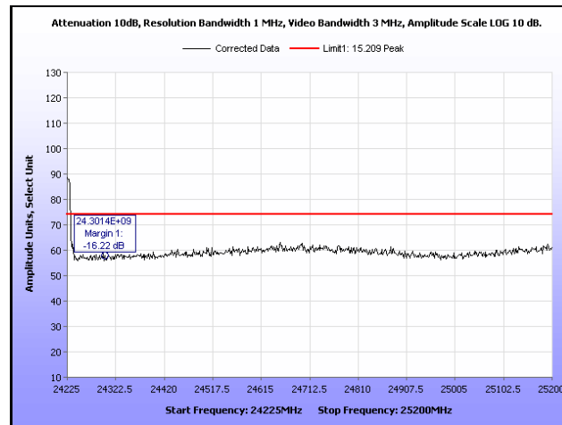
Plot 200. Radiated Band Edge, 10 MHz, High Channel, Peak
