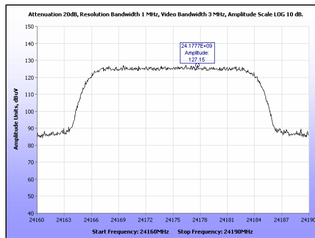
Plot 10. Radiated Field Strength of Fundamental, 20 MHz, Mid Channel
