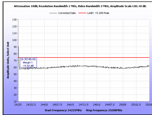
Plot 196. Radiated Band Edge, 5 MHz, High Channel, Peak
