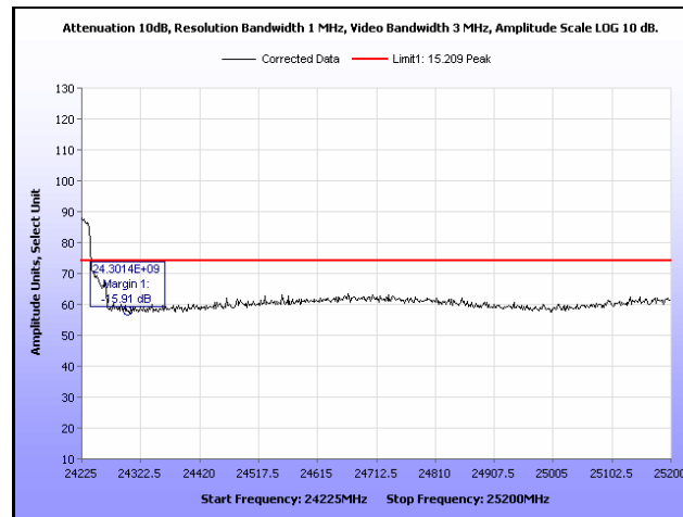
Plot 212. Radiated Band Edge, 30 MHz, High Channel, Peak
