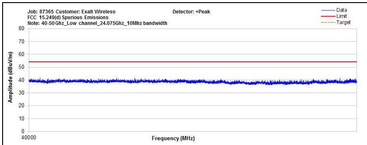
Plot 53. Radiated Spurious Emissions, 10 MHz, Low Channel, 40 GHz - 50 GHz
