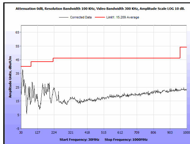
Plot 64. Radiated Spurious Emissions, 10 MHz, High Channel, 30 MHz – 1 GHz
