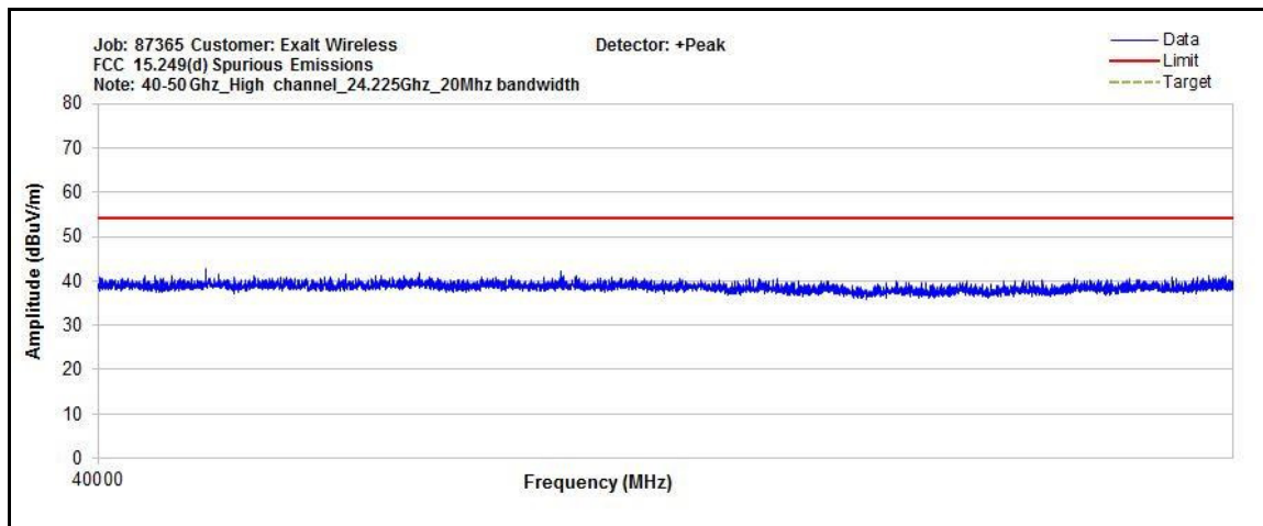
Plot 93. Radiated Spurious Emissions, 20 MHz, High Channel, 40 GHz – 50 GHz
