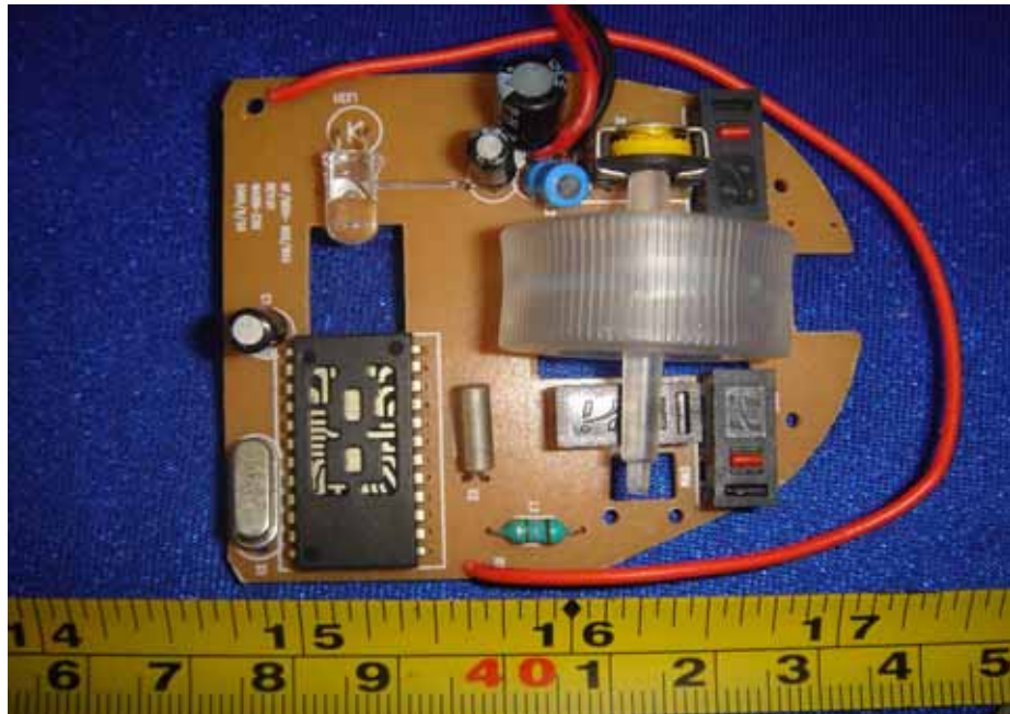
PCB – Component View
