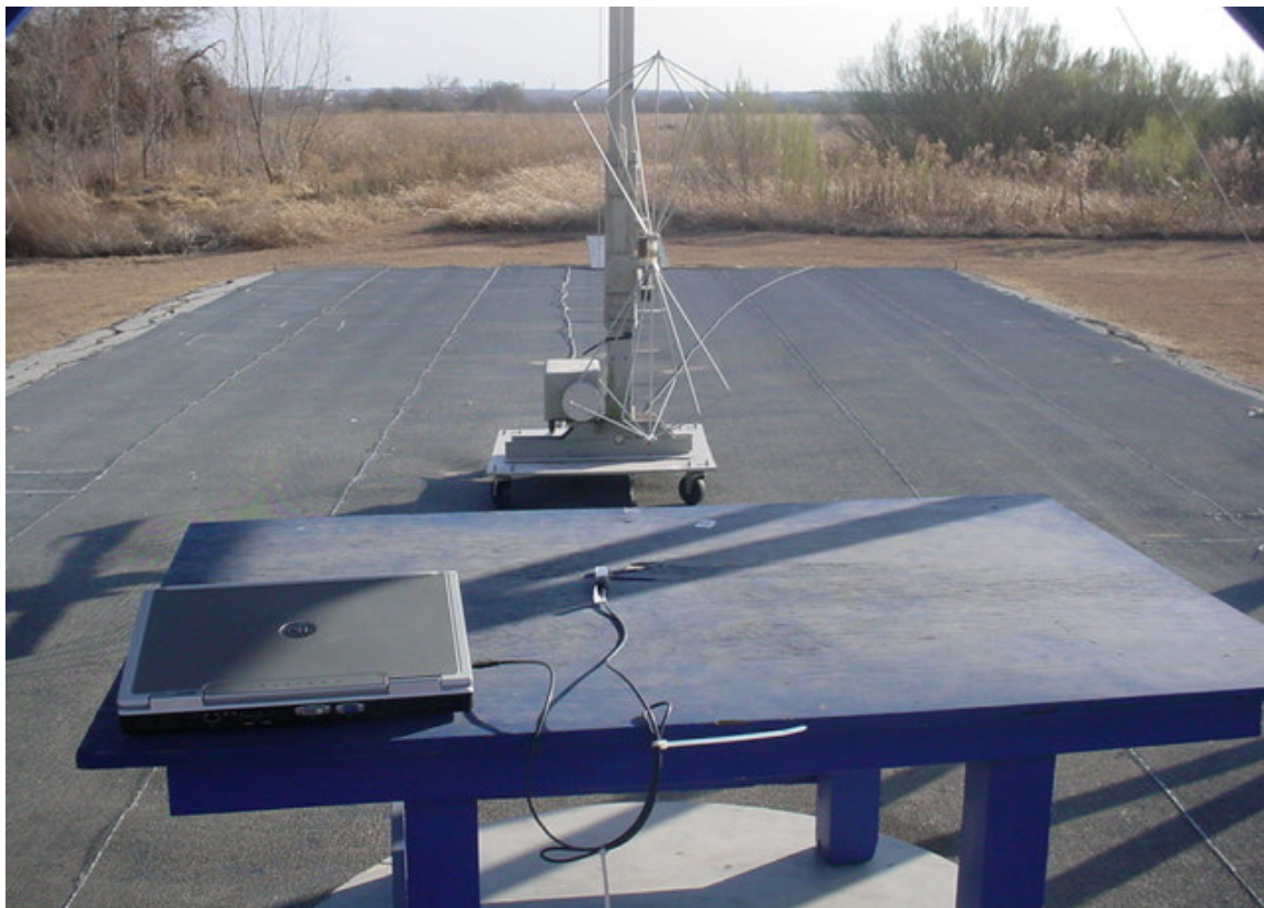
Figure 2 - Radiated Spurious Emissions < 1 GHz
