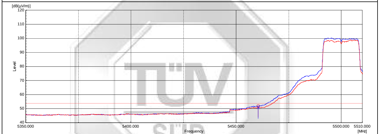
Plot 6 – Average Plot at Upper Band Edge at 5.4600GHz
