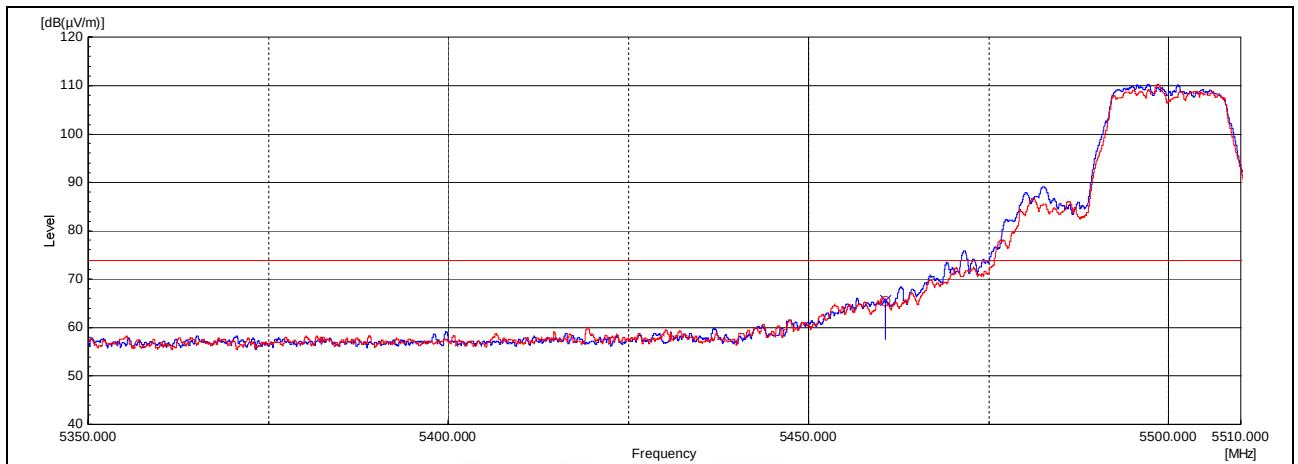
Plot 5 – Peak Plot at Upper Band Edge at 5.4600GHz
