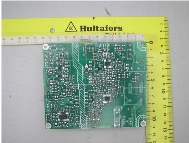
PSU bottom
