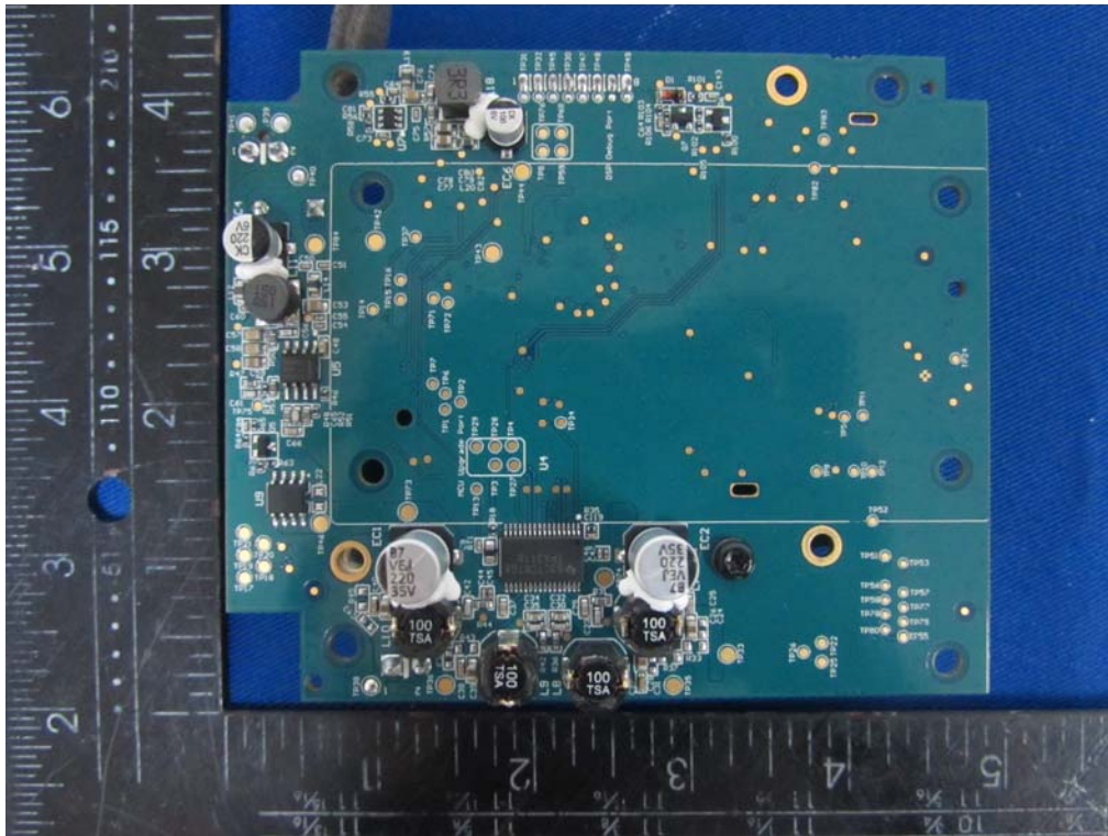
Internal Photos M/N: Beoplay M3
