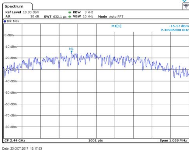
Channel 19 / 2440 MHz
