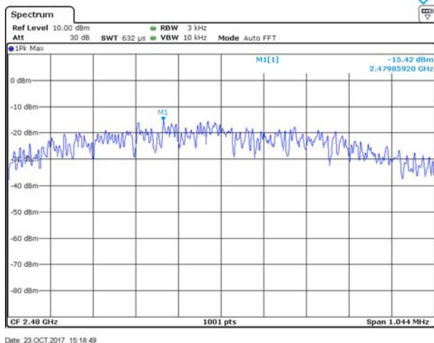
Channel 39 / 2480 MHz
