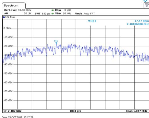
Channel 0 / 2402 MHz
