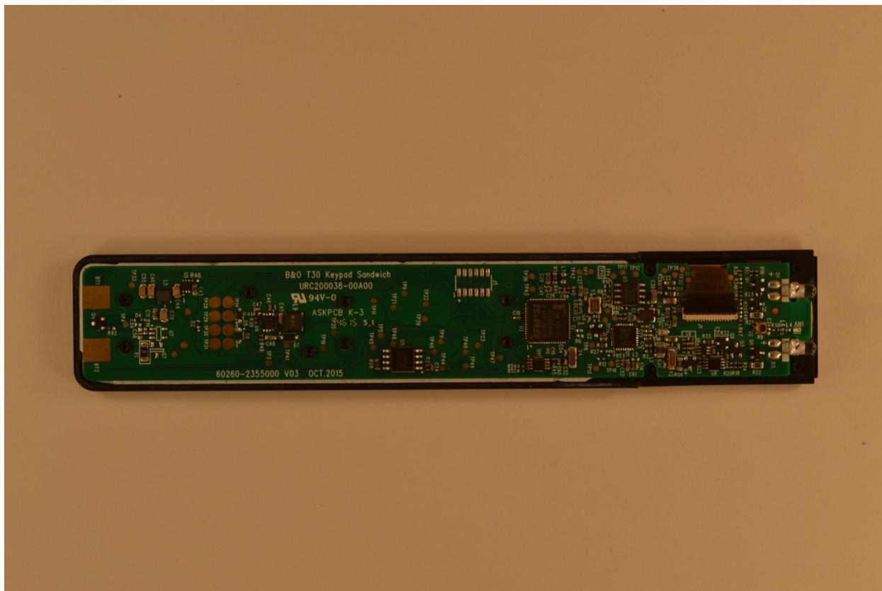
EUT Control Unit Internal – Bottom View
