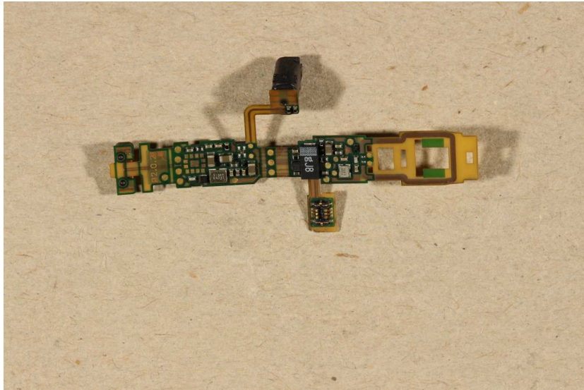
Photo 3: FPC, bottom side view
