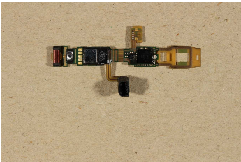
Photo 4: FPC, top side view
