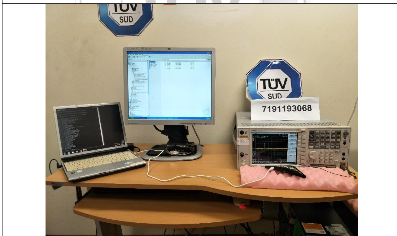
RF Conducted Spurious Emissions (Restricted Bands) Test Setup
