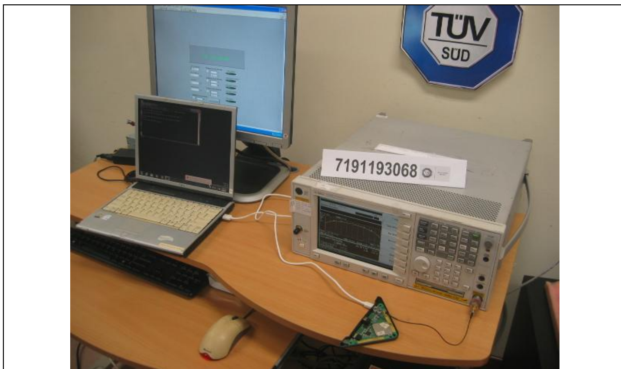
RF Conducted Spurious Emissions (Non-Restricted Bands) Test Setup
