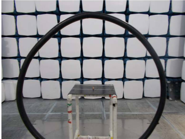
Test Setup Photograph(s)
