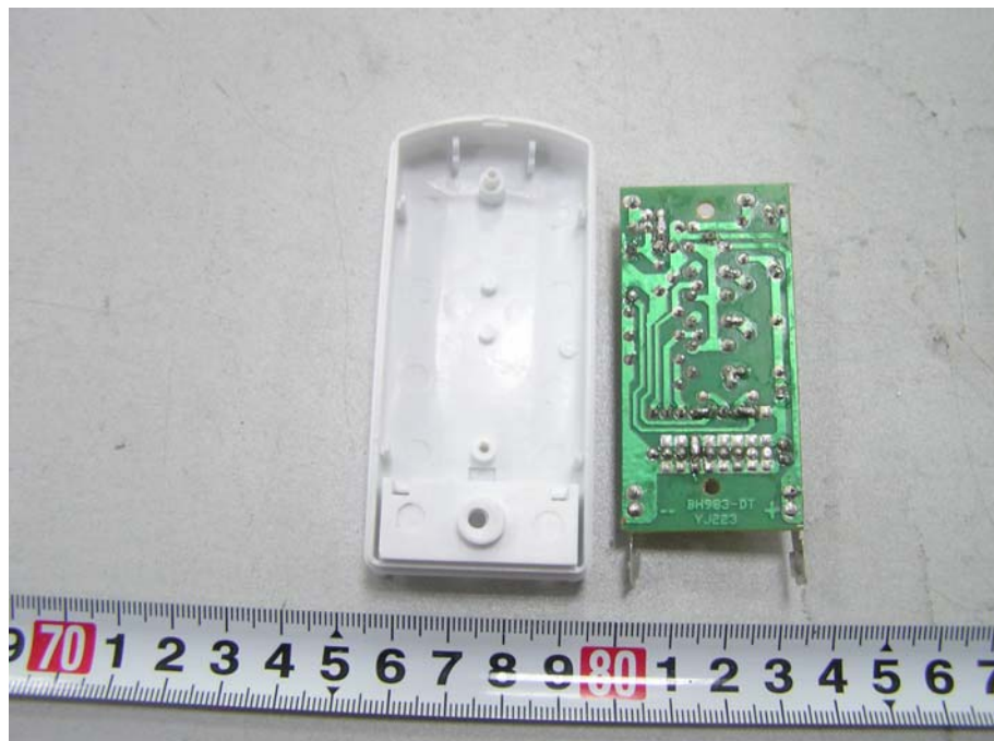
EUT –Inside (PCB Bottom) View
