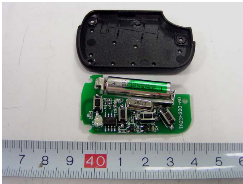
EUT-Inside View (3)
