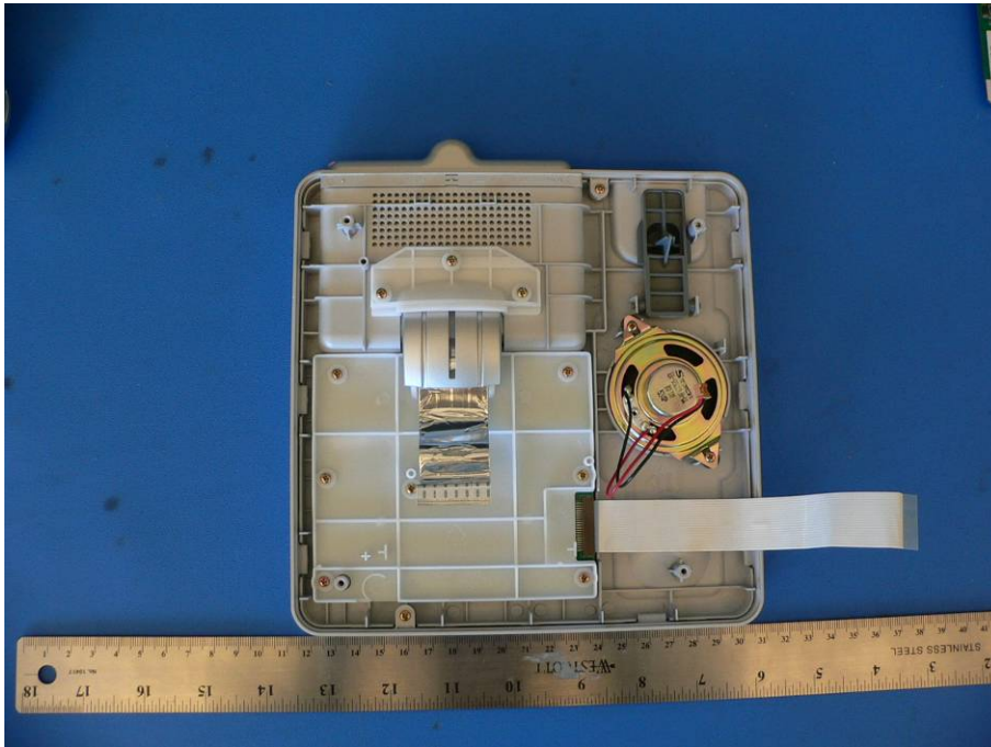
Power Supply Side View
