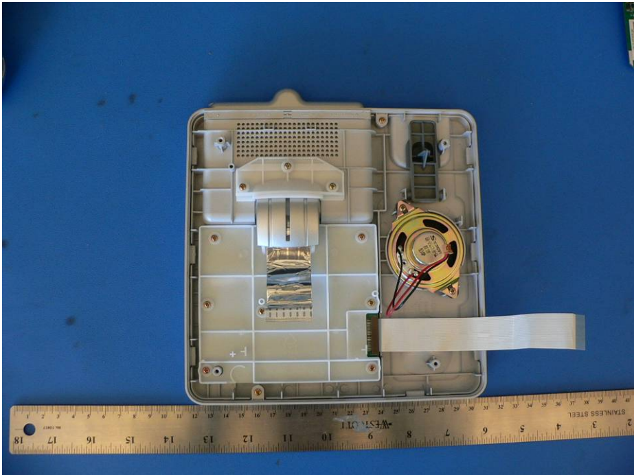
EUT-Top Chassis bottom View
