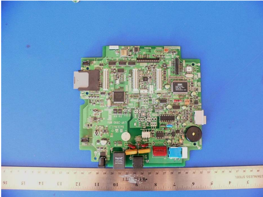
EUT- Main PCB Component Side View
