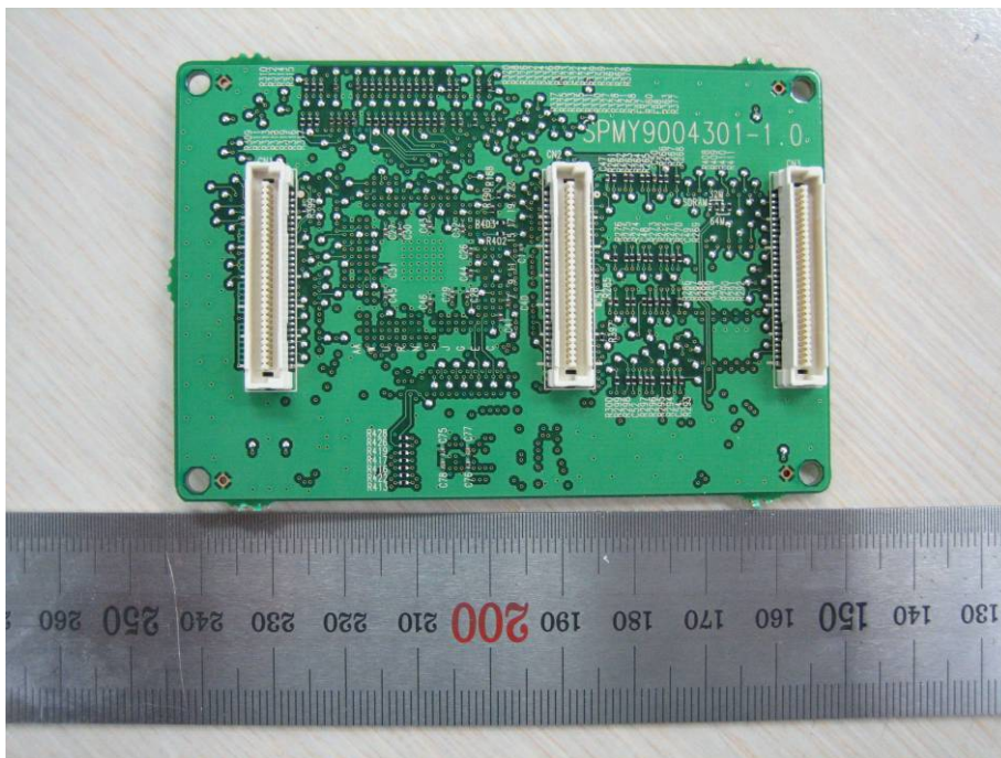
EUT-SUB PCB Solder Side View
