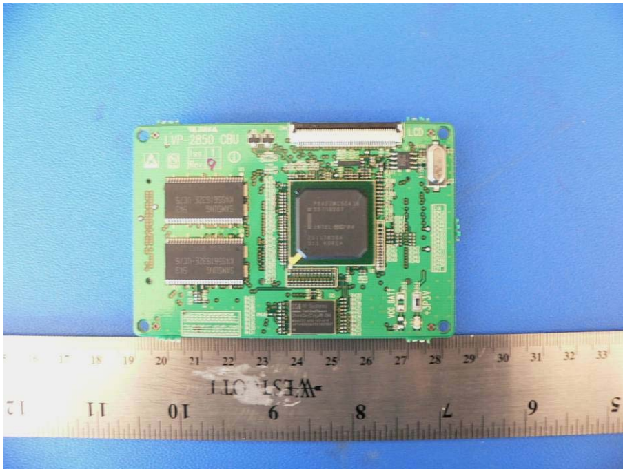
EUT- SUB PCB Component Side View
