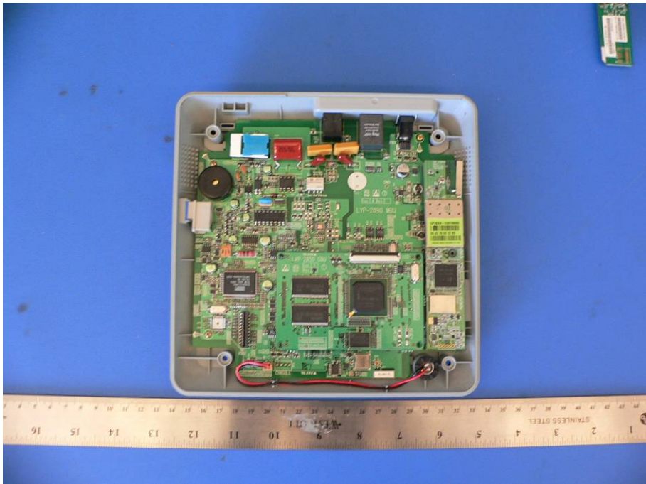
EUT- Chassis off with Samsung RF Module View
