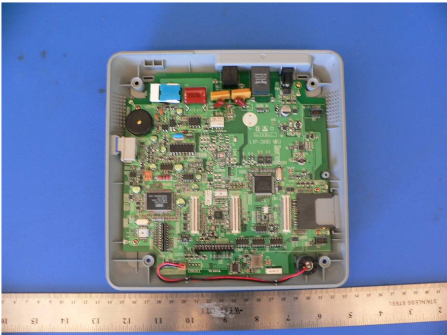
EUT- Chassis off without RF module SUB PCB View
