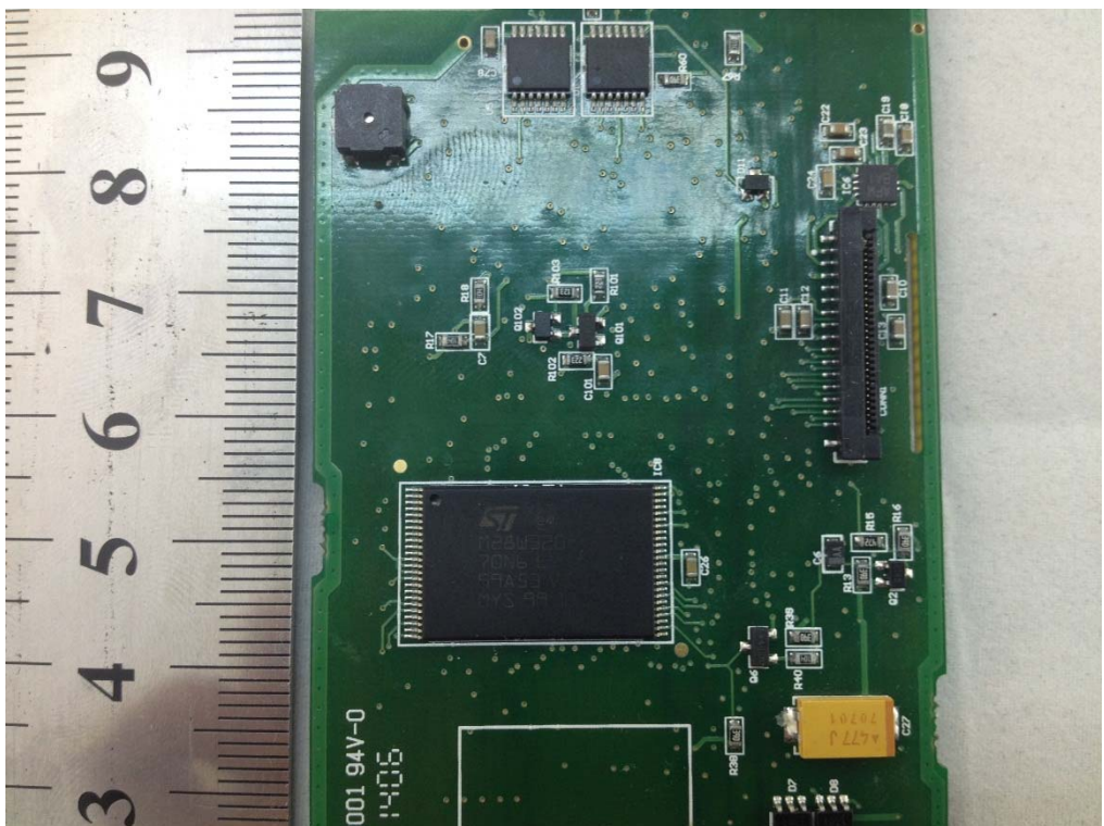
MAIN BOARD VIEW 4
