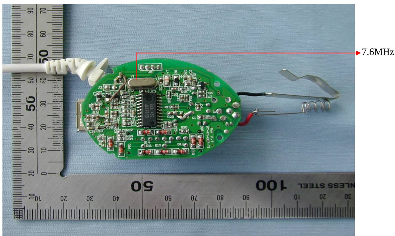
Full View of Solder Side
