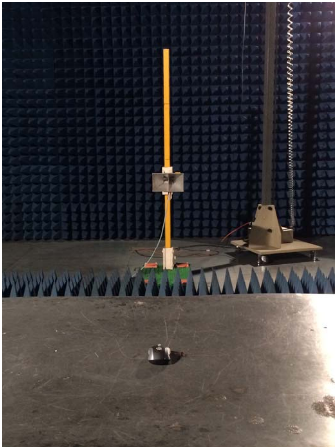
Radiated emissions test > 1GHz
